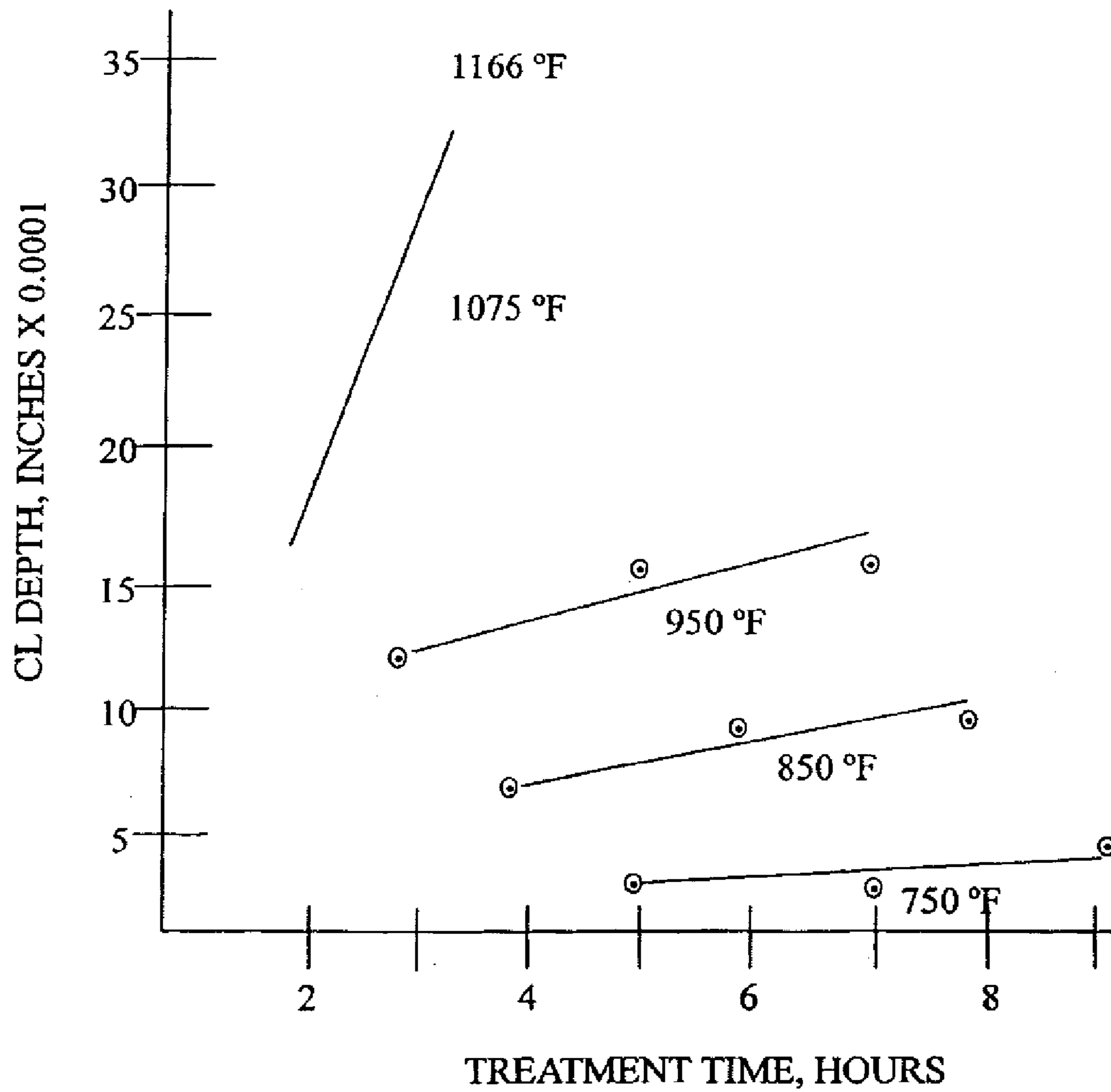
DIFFUSION 416 STAINLESS STEEL
