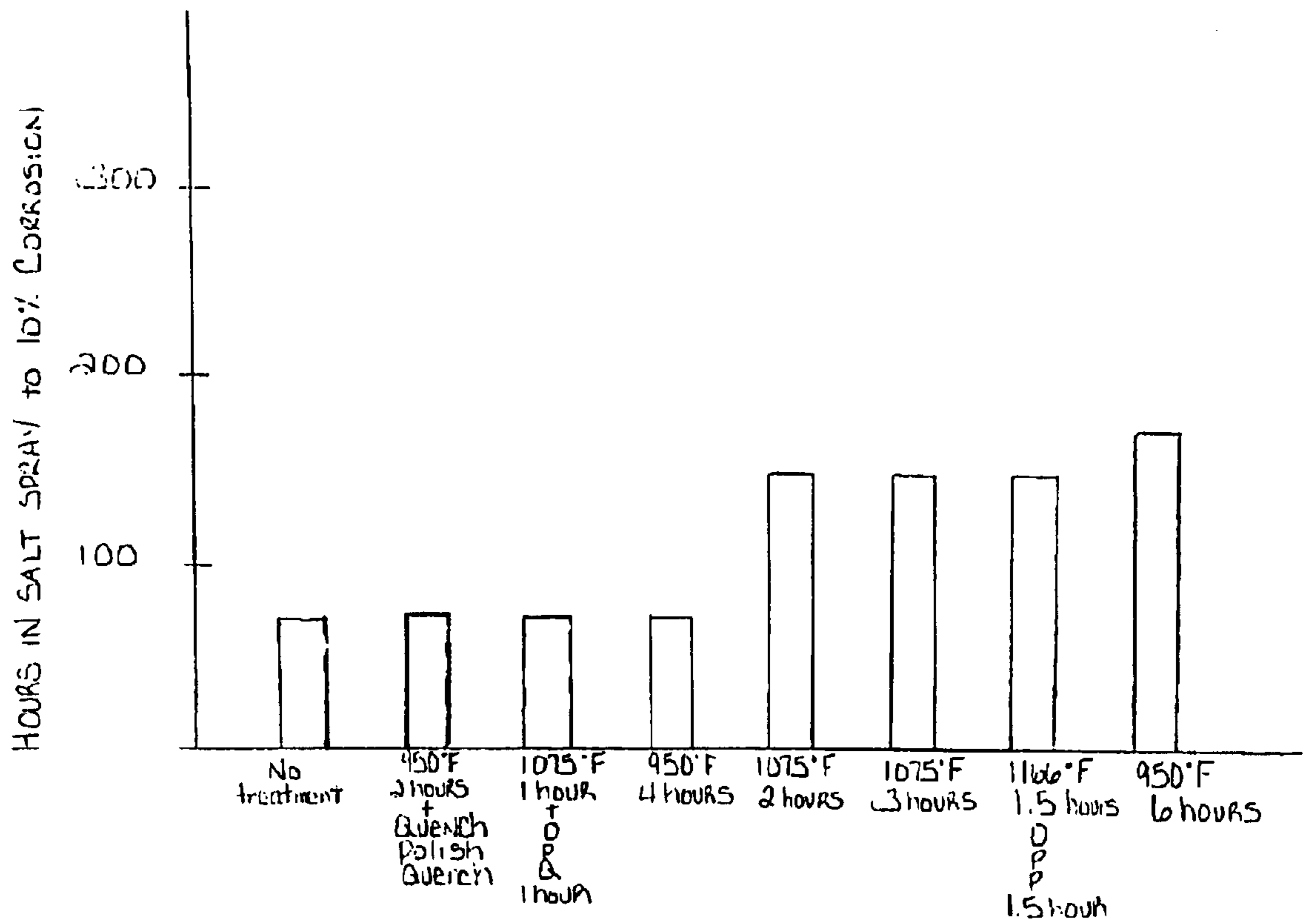
4/6 Stainless Steel Fig. 3
