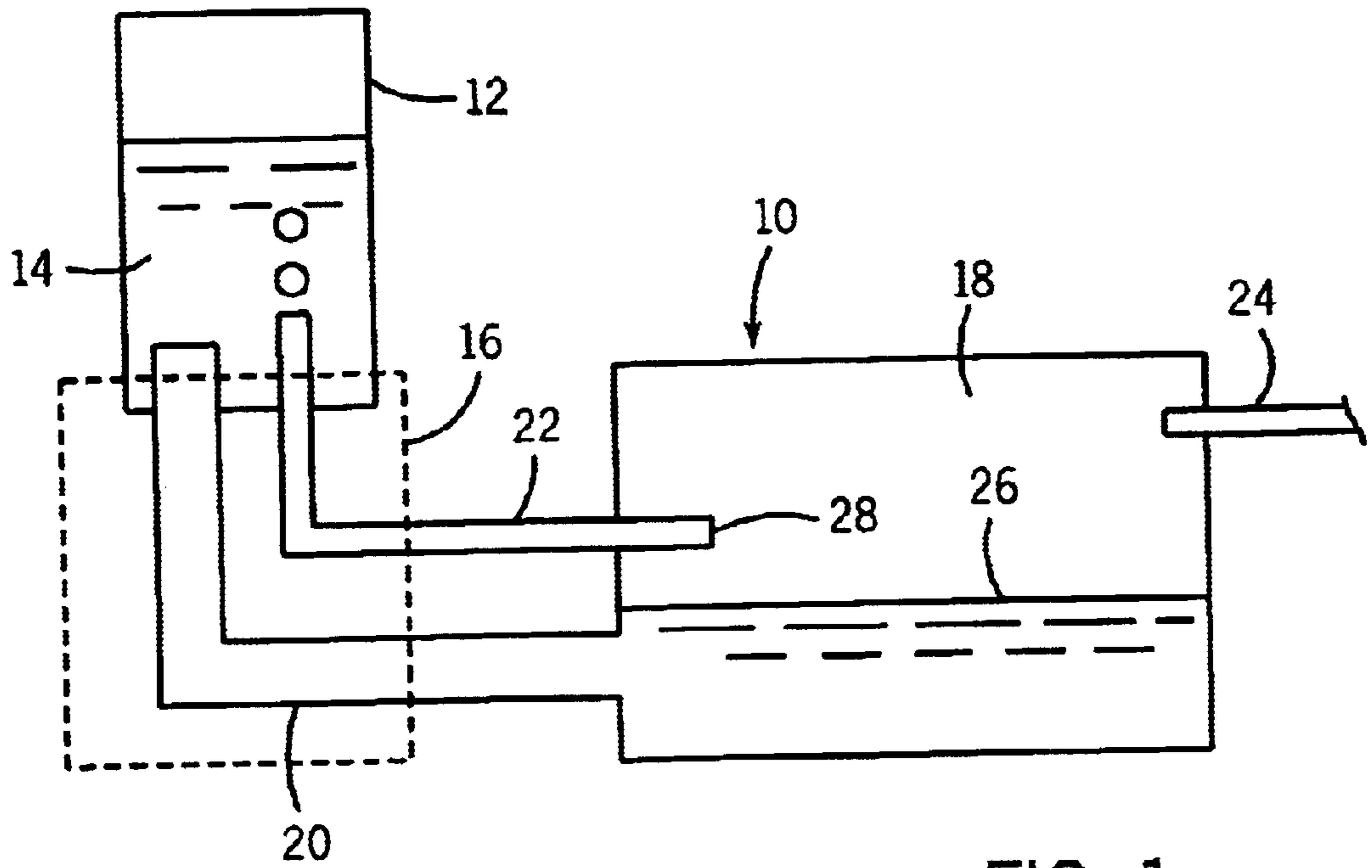
FIG. 1 PRIOR ART
