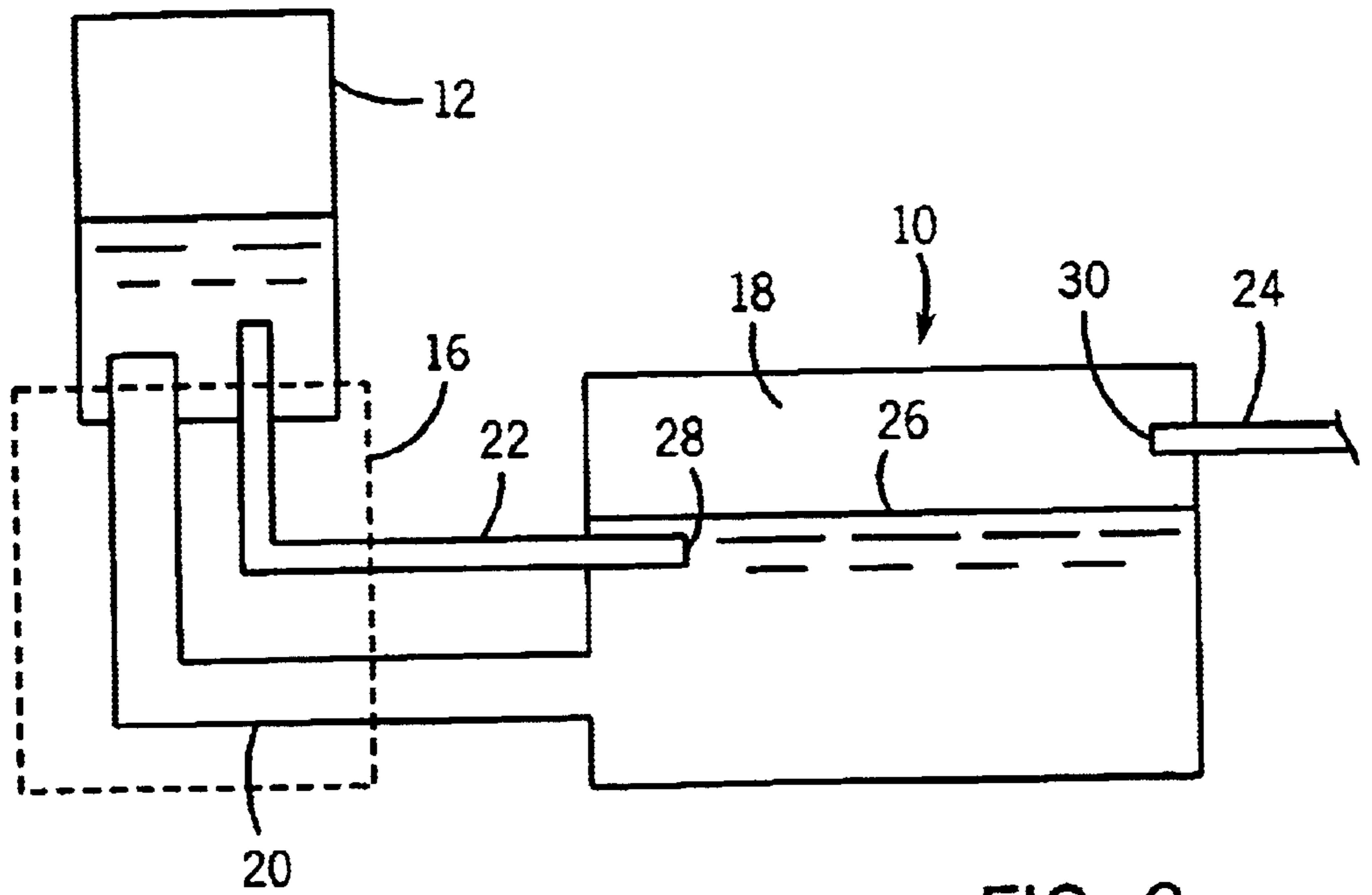
FIG. 2 PRIOR ART
