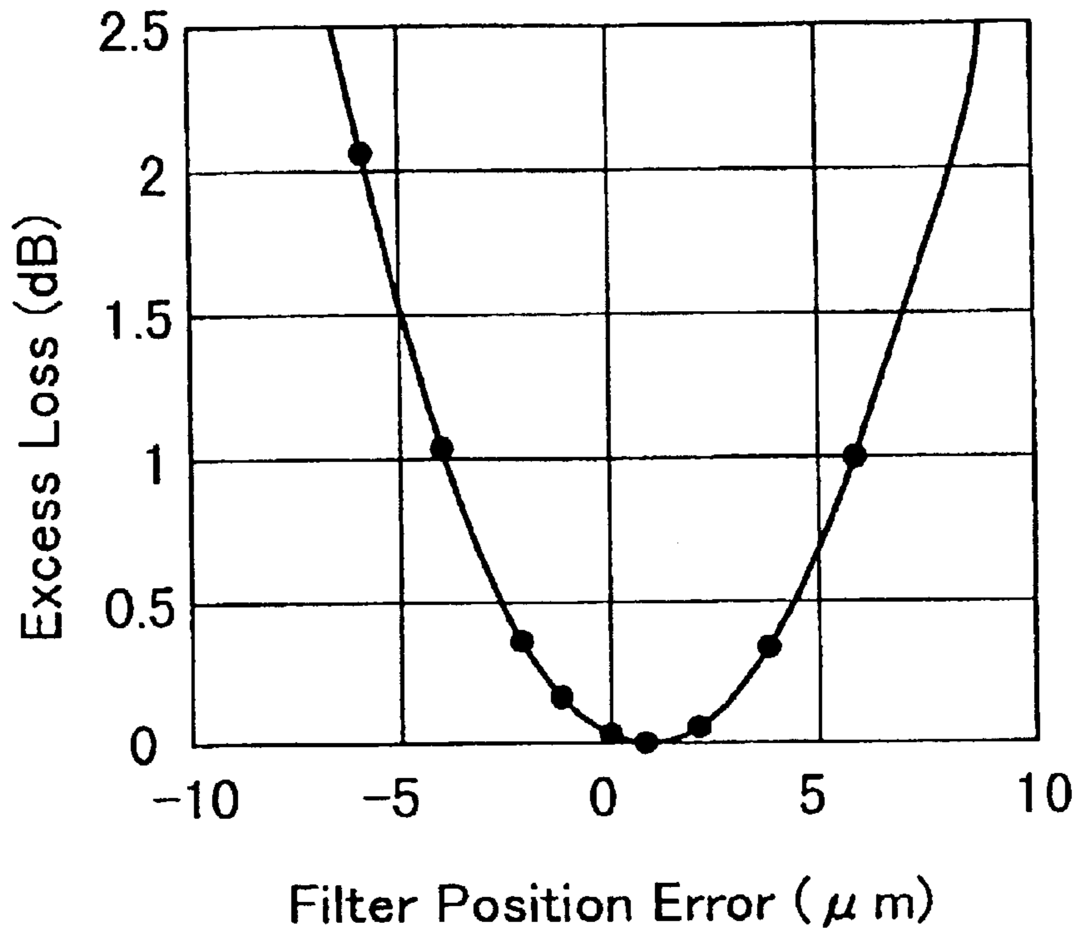
FIG. 3 PRIOR ART
