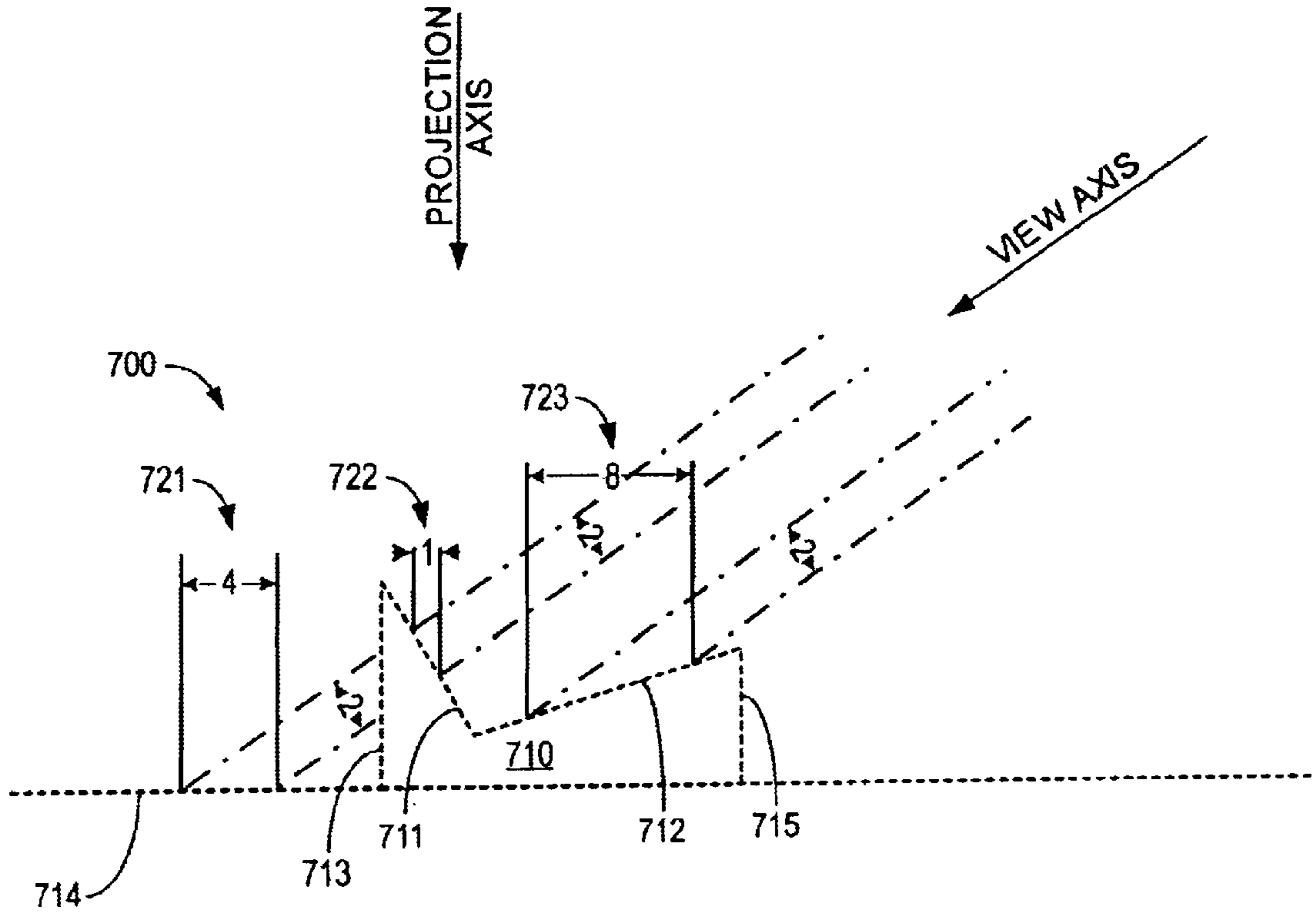
FIG. 8 PRIOR ART
