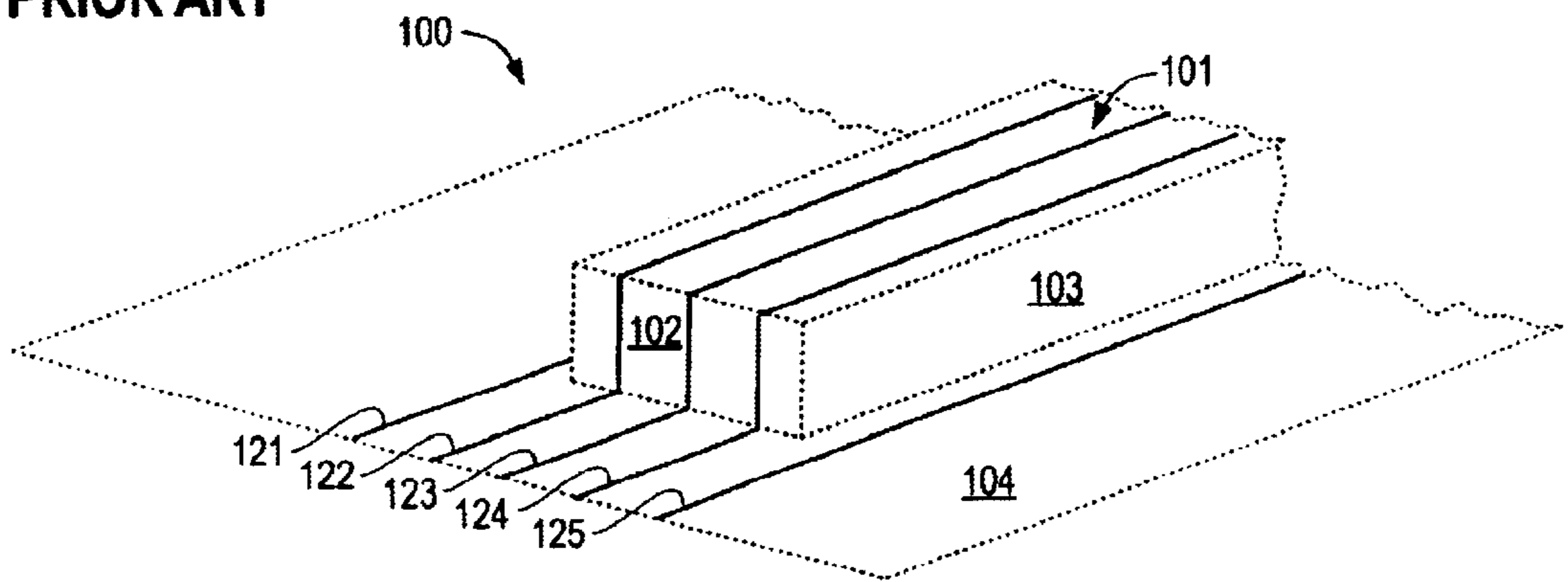
FIG. 2 PRIOR ART
