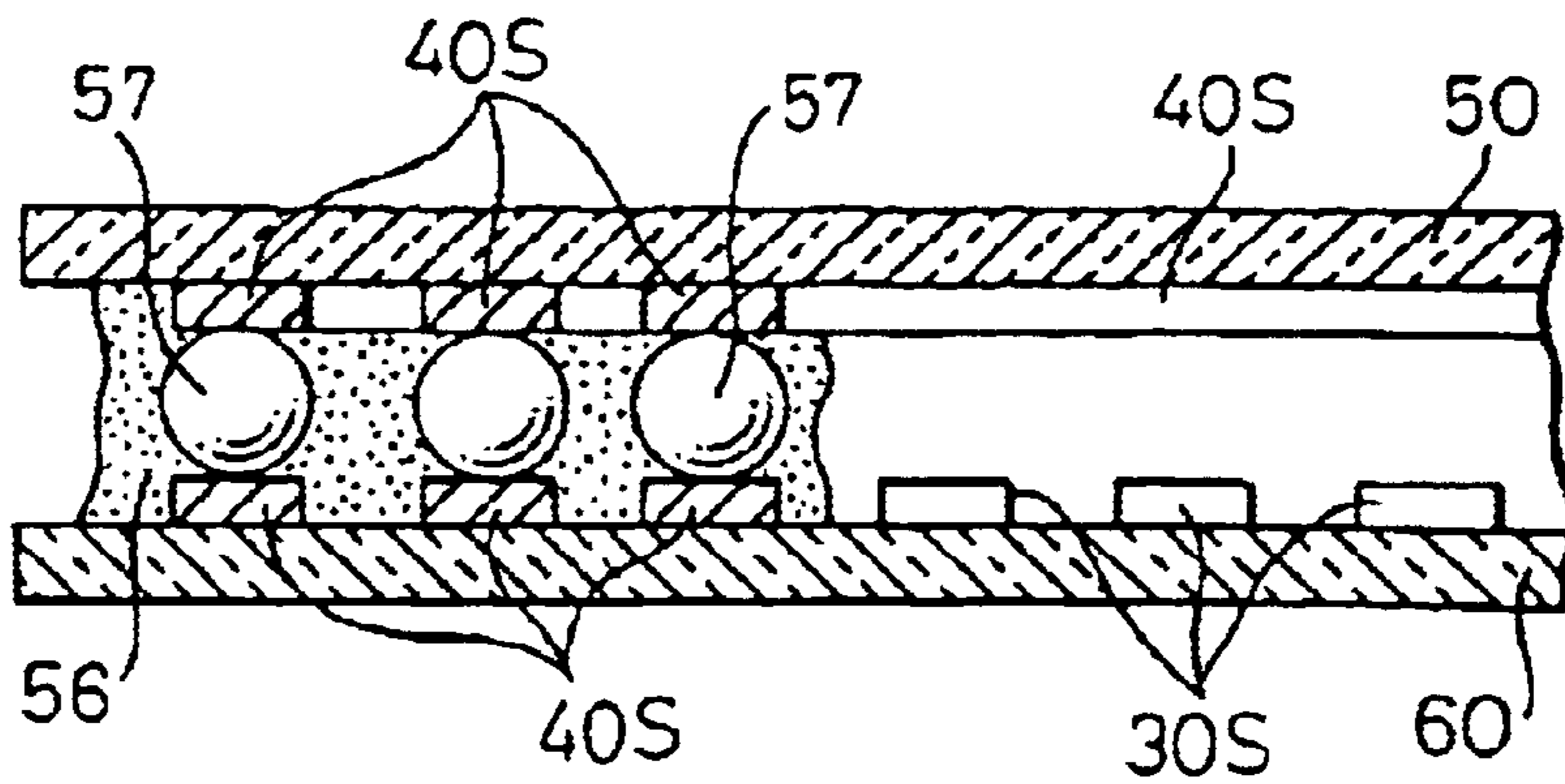
Fig. 8 PRIOR ART
