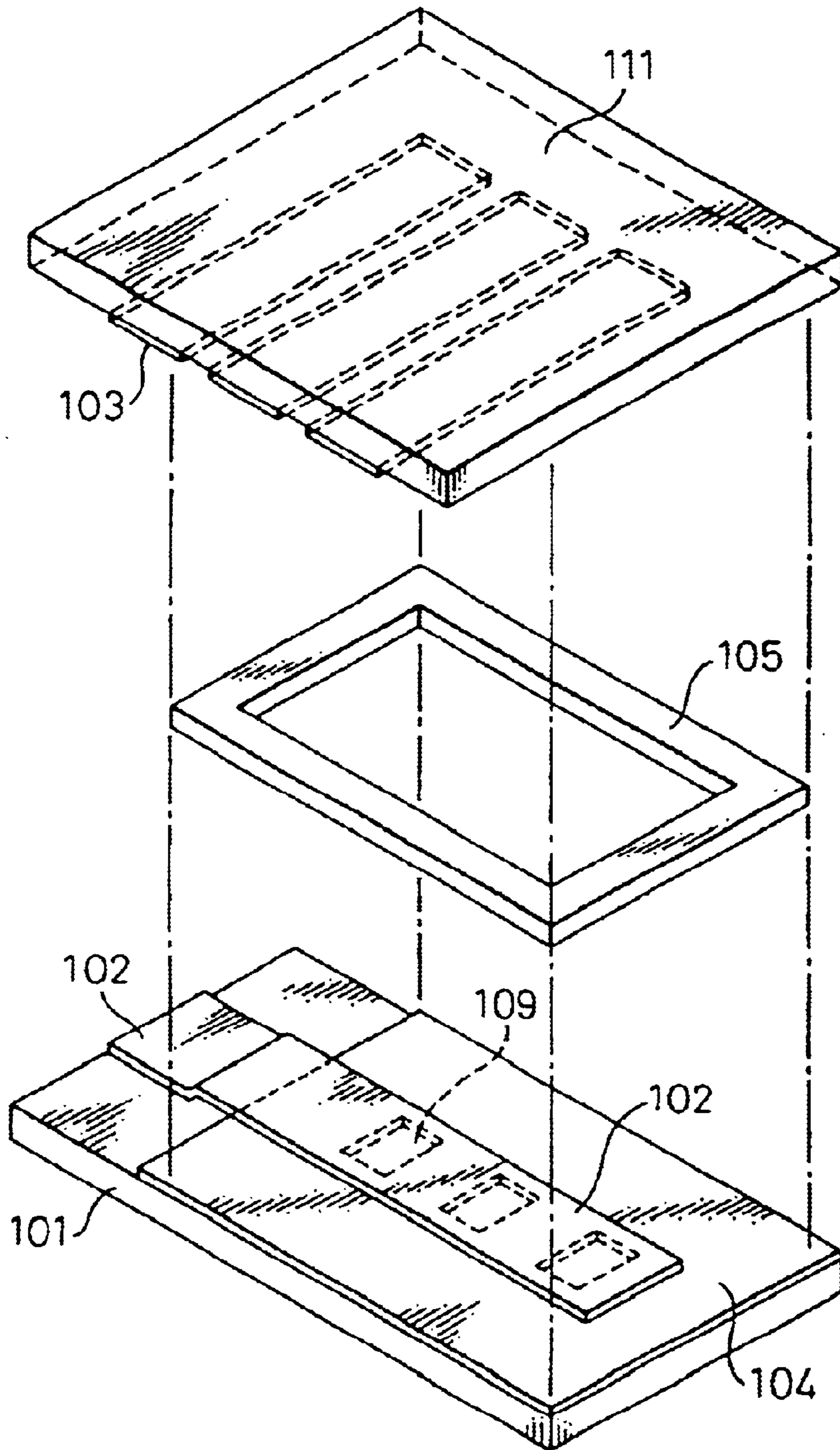
Fig. 19 PRIOR ART
