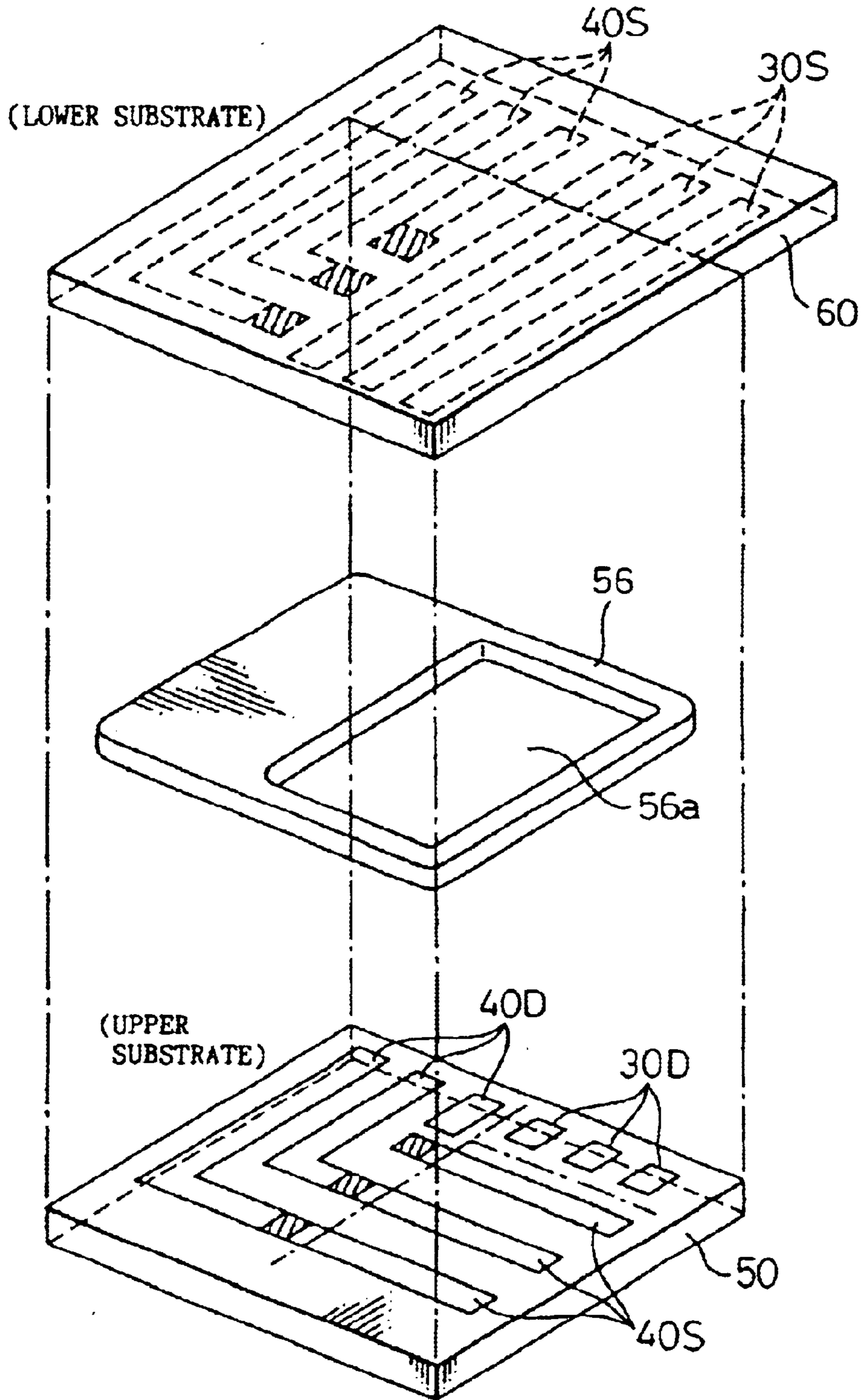
Fig. 5 PRIOR ART
