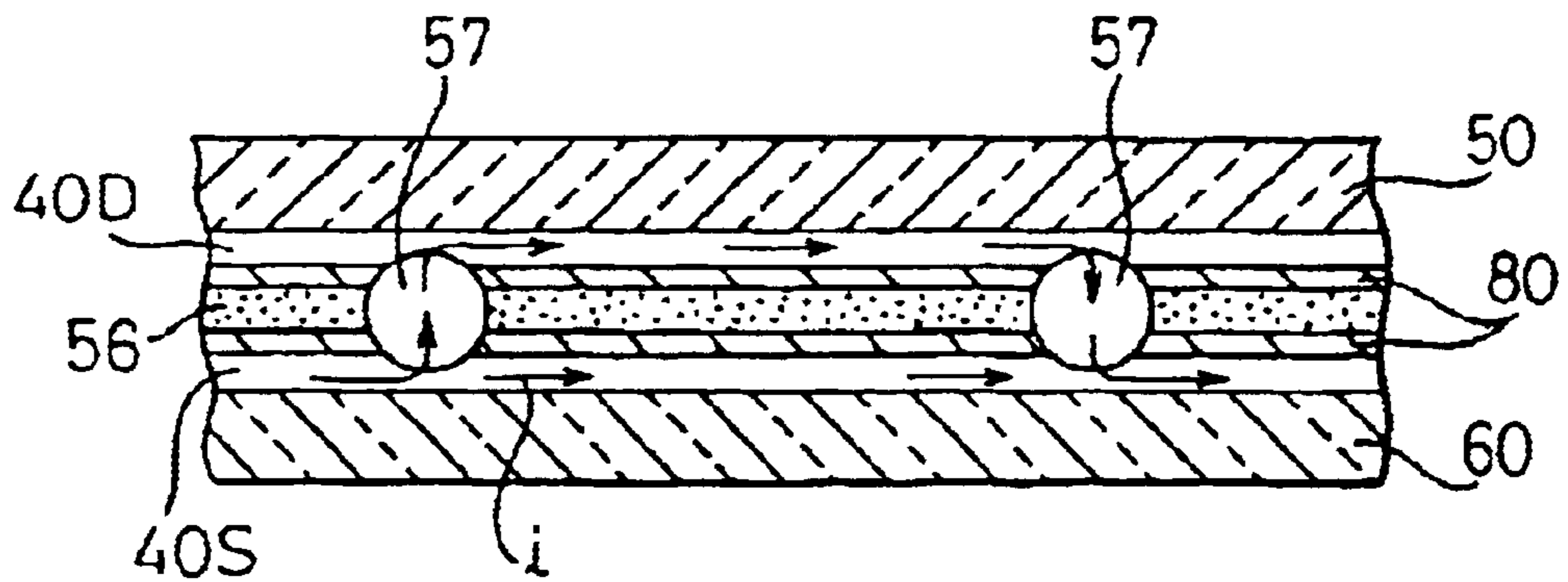
Fig. 10 PRIOR ART
