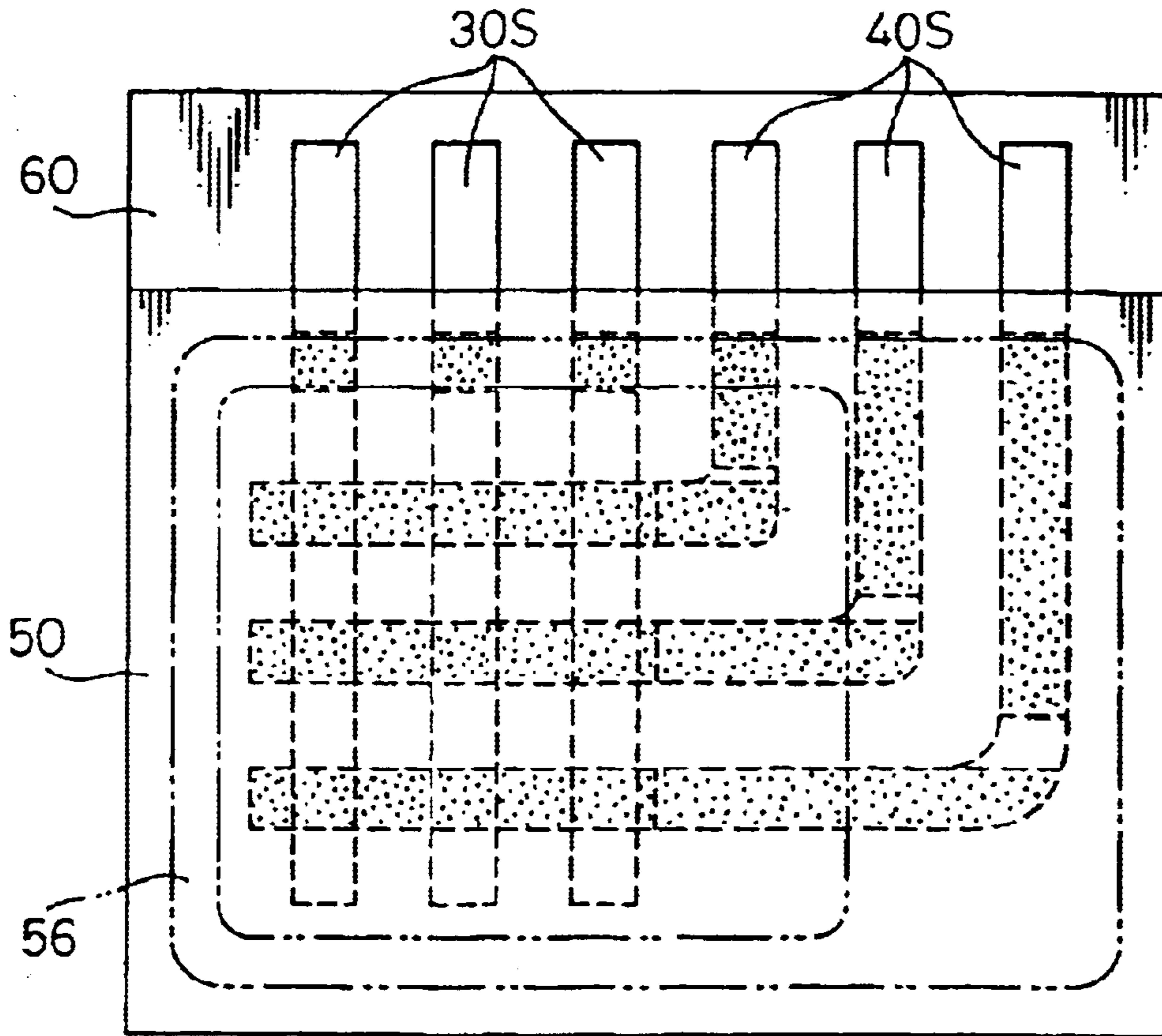
Fig. 7 PRIOR ART
