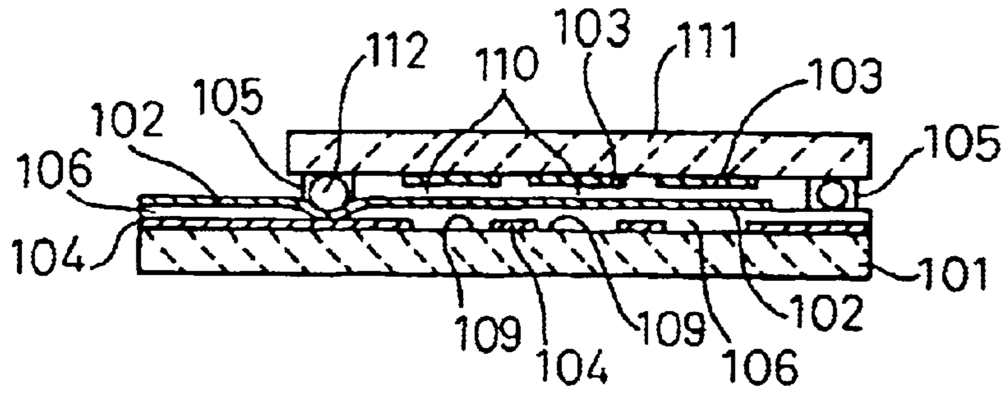
Fig. 23 PRIOR ART
