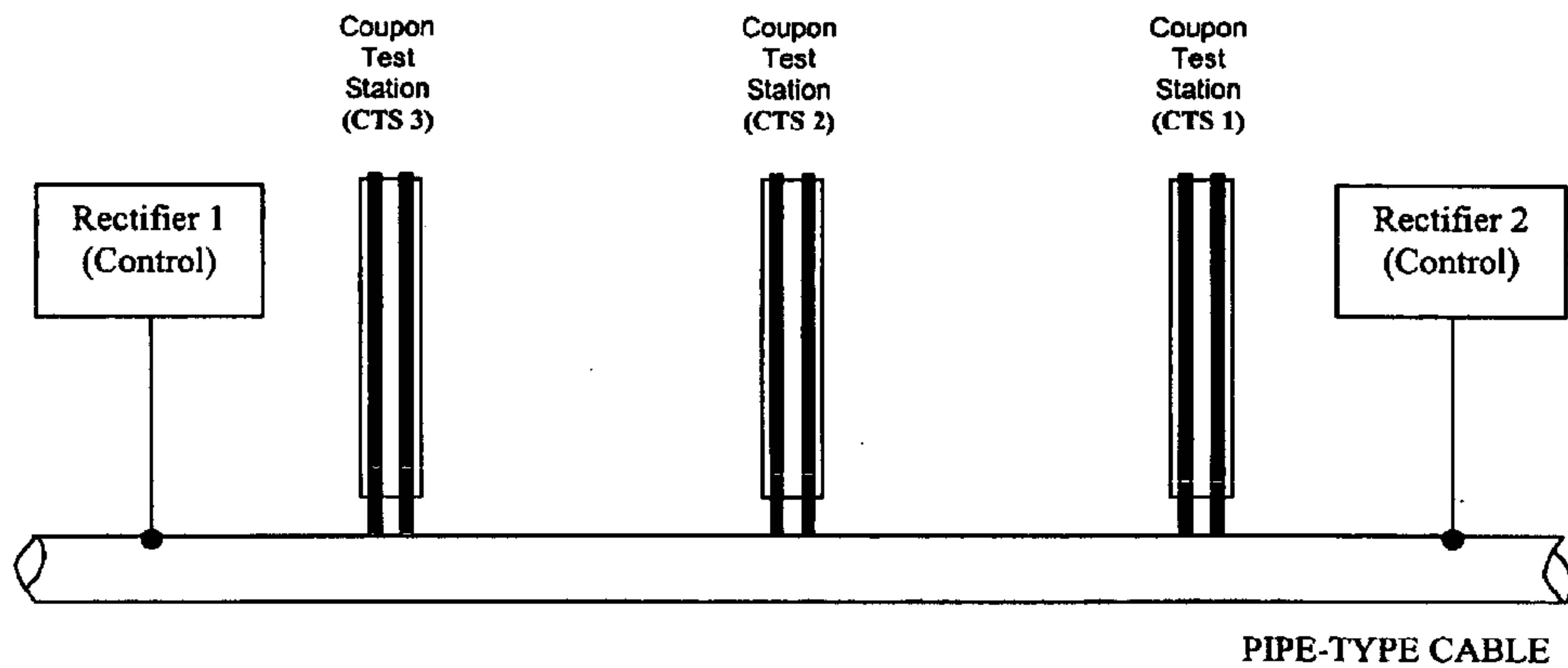
10 FIGURE 3 – Schematic of a simplified CP system for a pipe-type cable with CTS monitoring.
