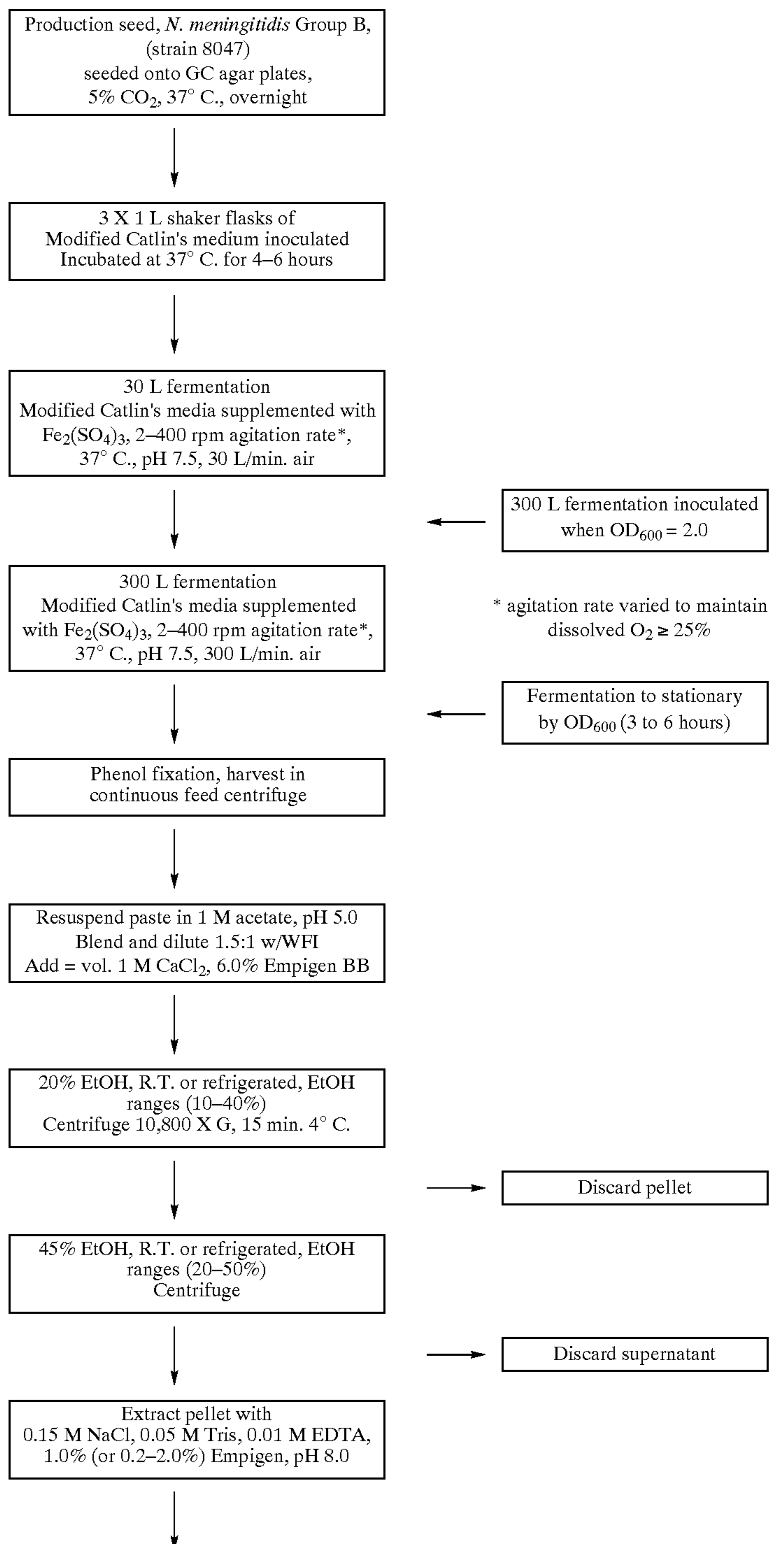
Manufacture of Proteosome Bulk Material: FLOWCHART 1
