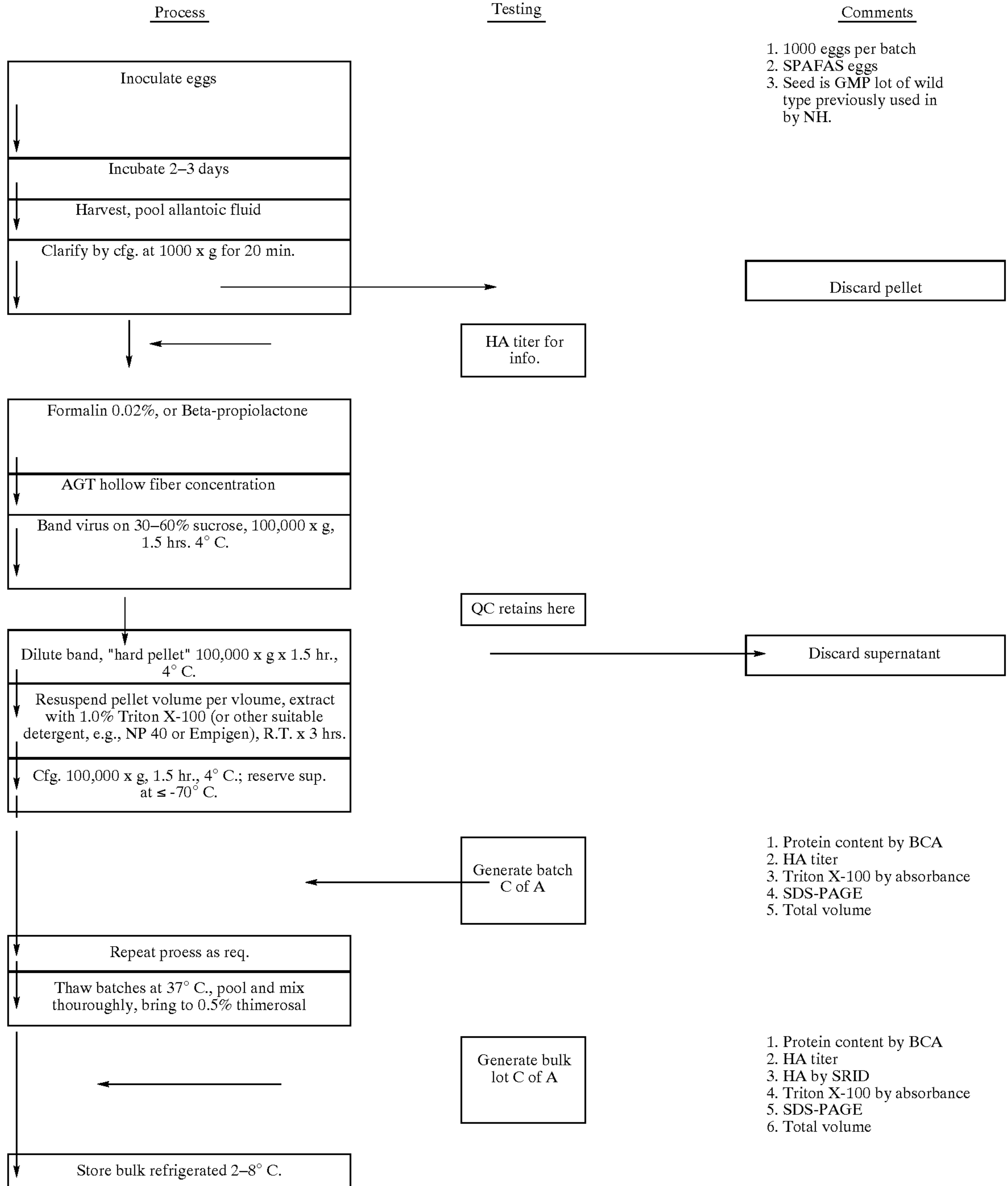
Bulk Influenza Antigen Process: FLOWCHART 2
