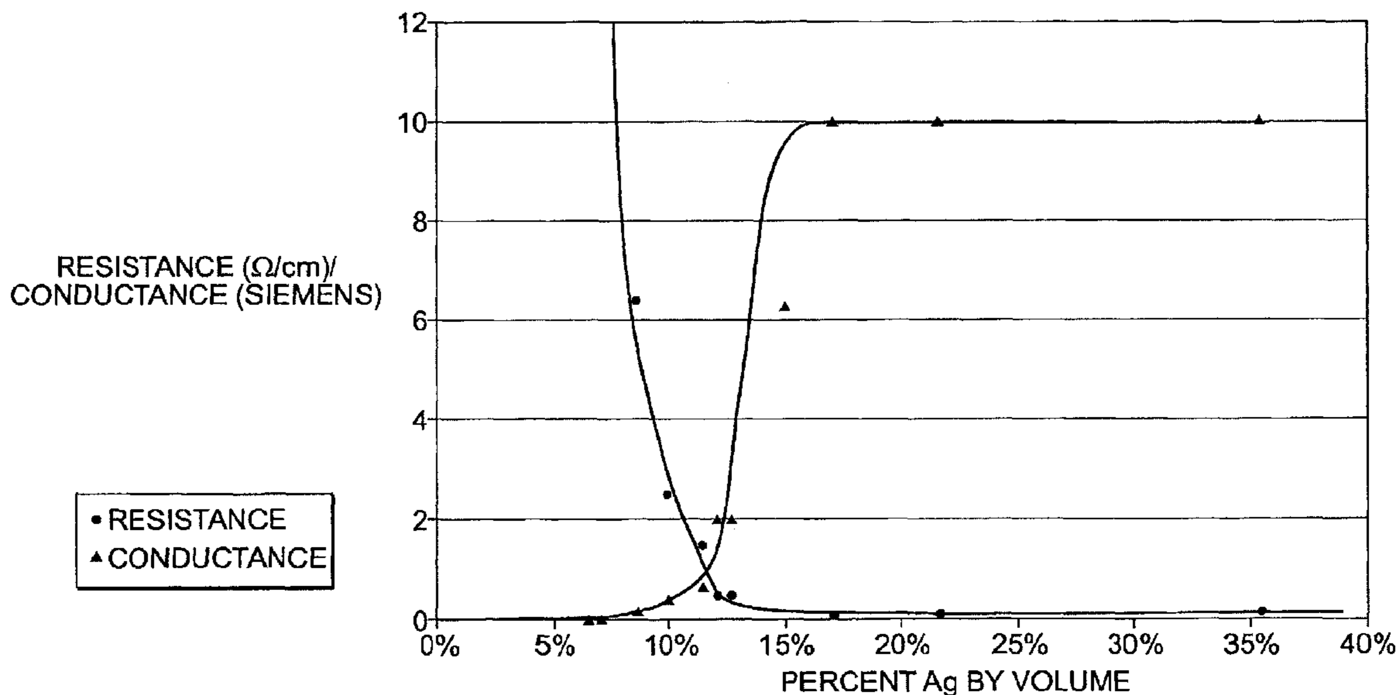
RESISTANCE / CONDUCTANCE VERSUS PERCENT Ag BY VOLUME
