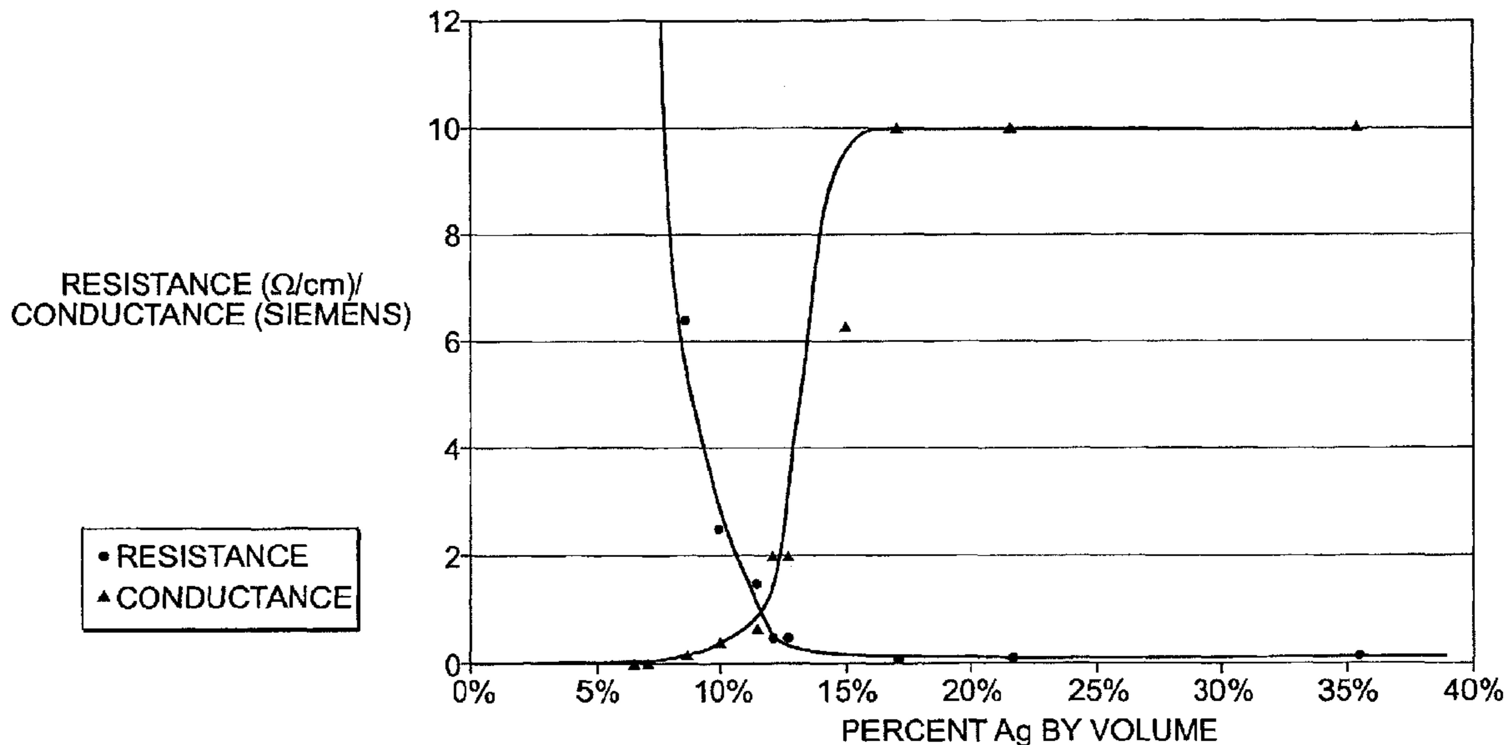
RESISTANCE / CONDUCTANCE VERSUS PERCENT Ag BY VOLUME
