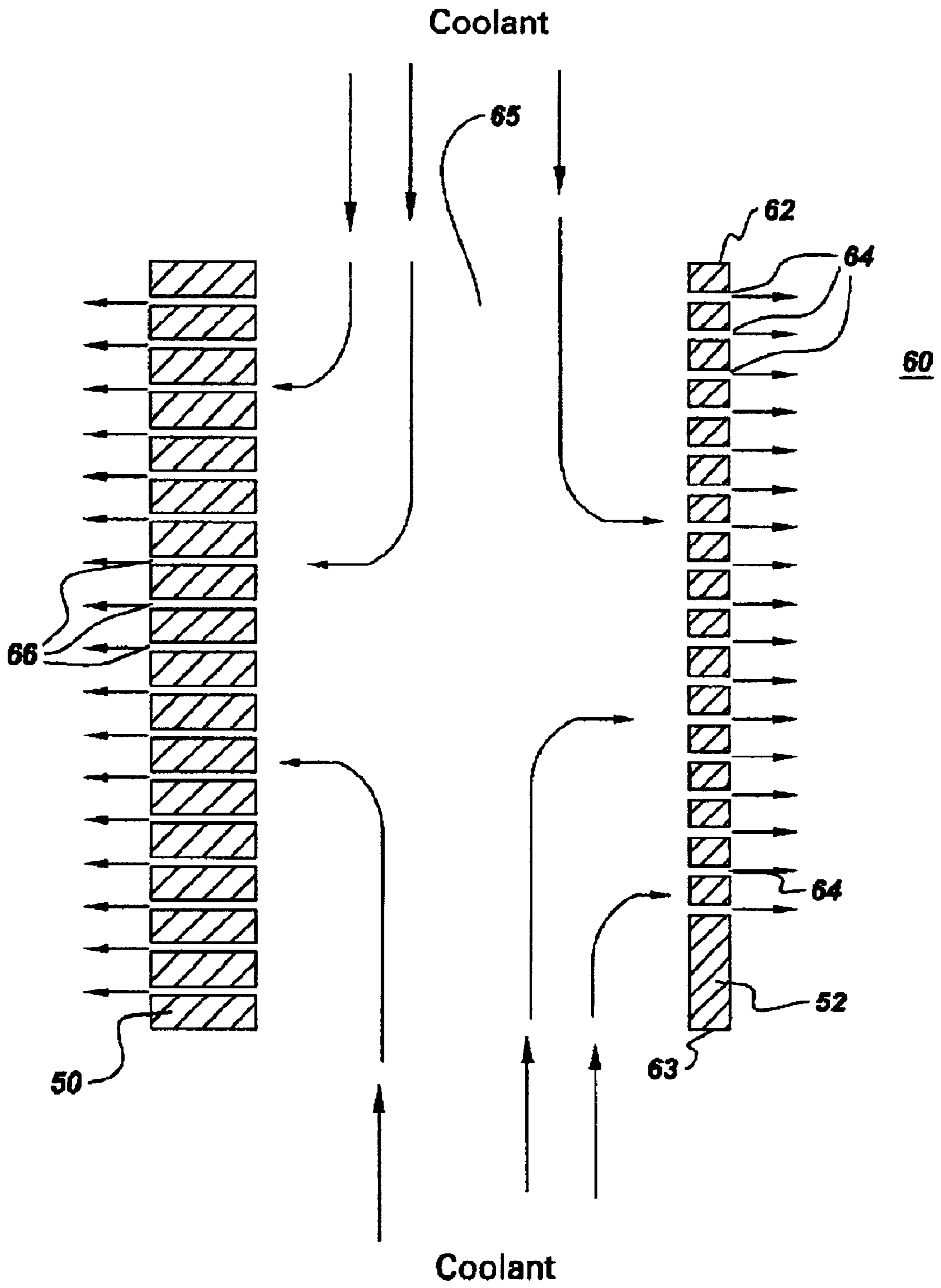
Fig. 4 Prior Art
