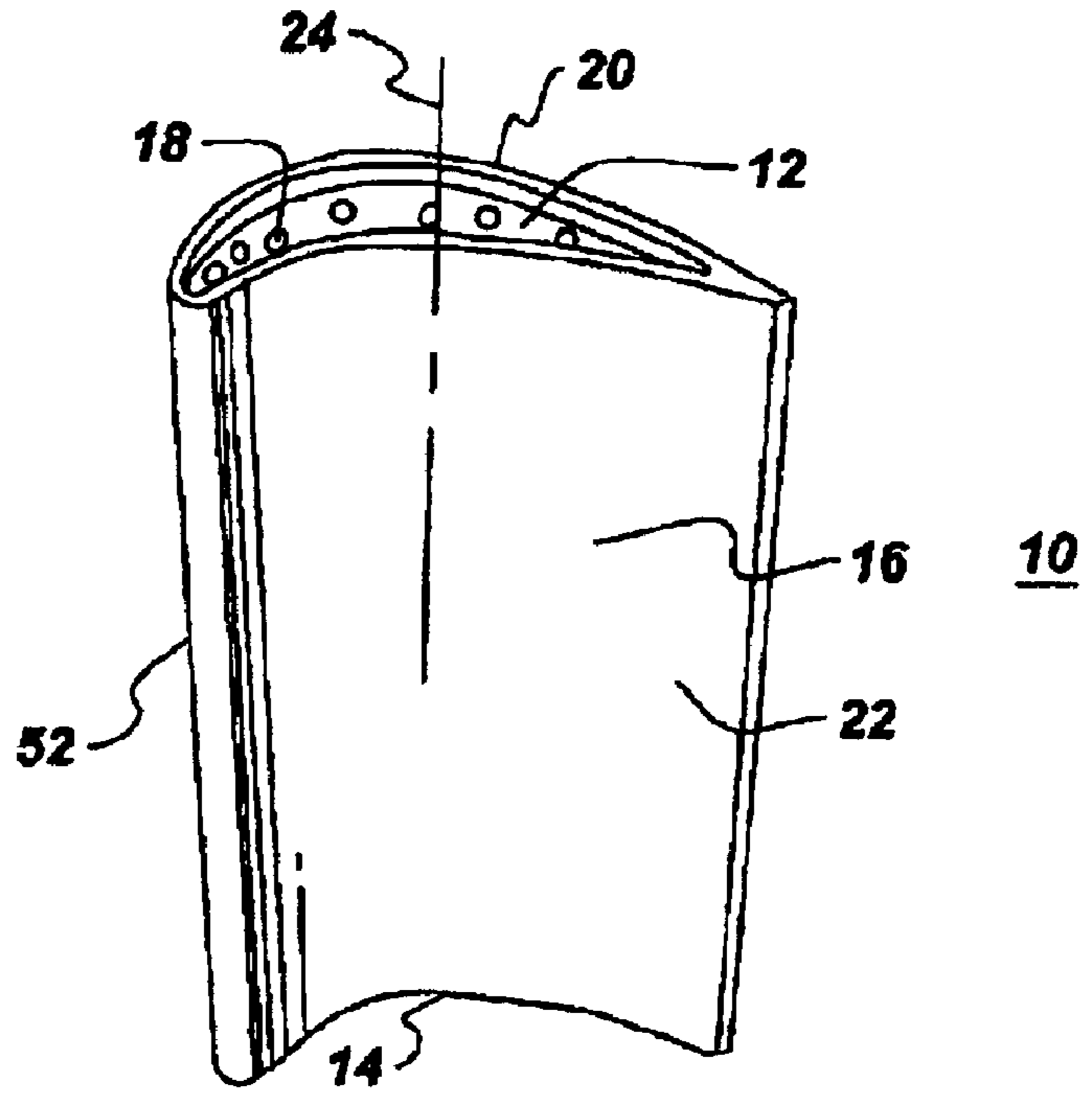
Fig. 1 Prior Art
