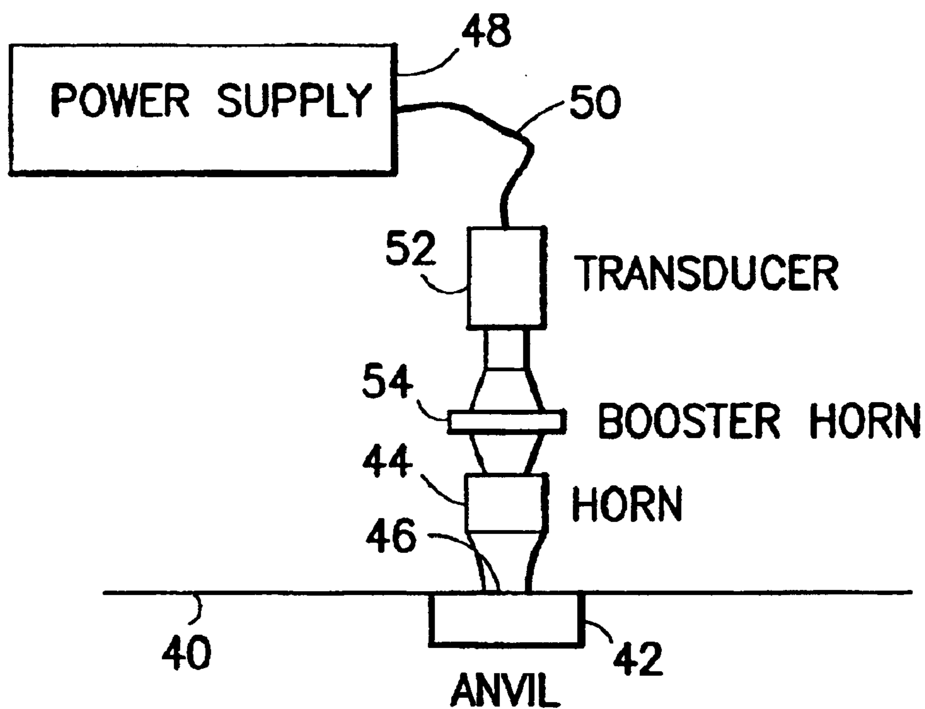
FIG. 4 PRIOR ART
