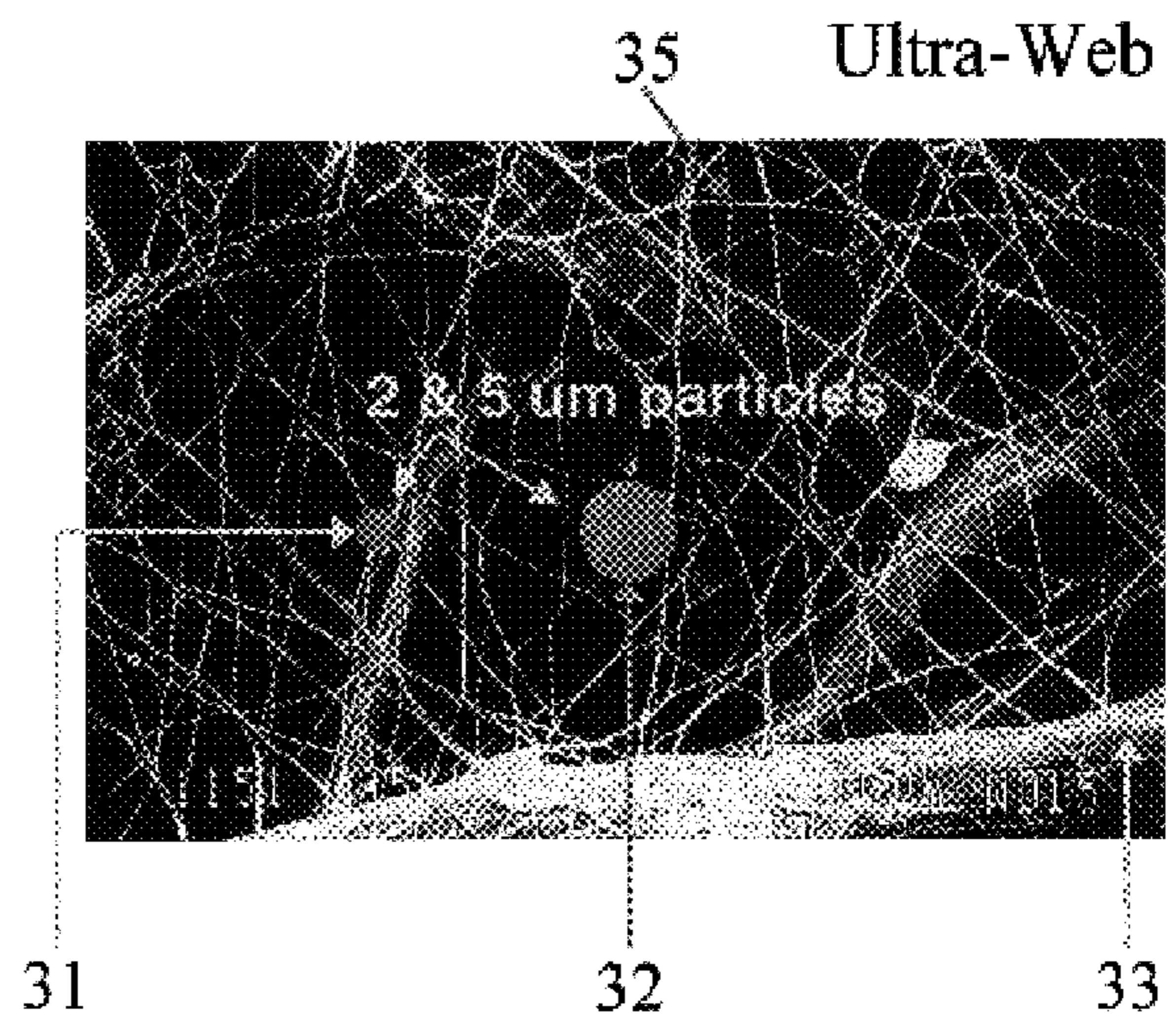
2,000 X Scanning Electron Microscope Images
