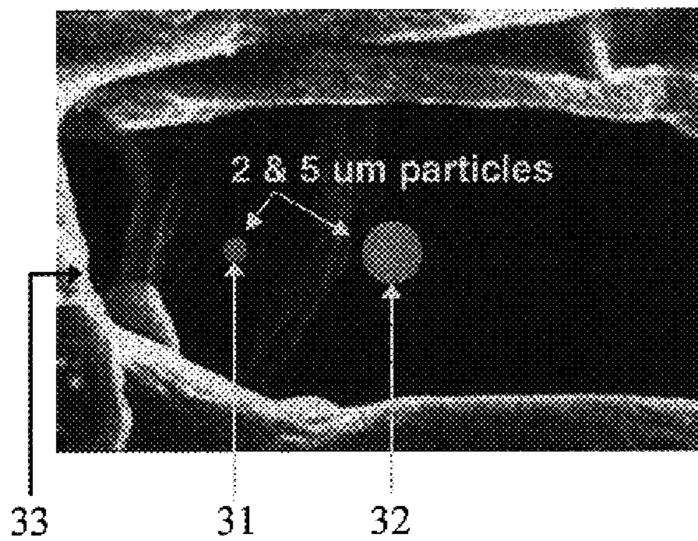
2,000 X Scanning Electron Microscope Images
