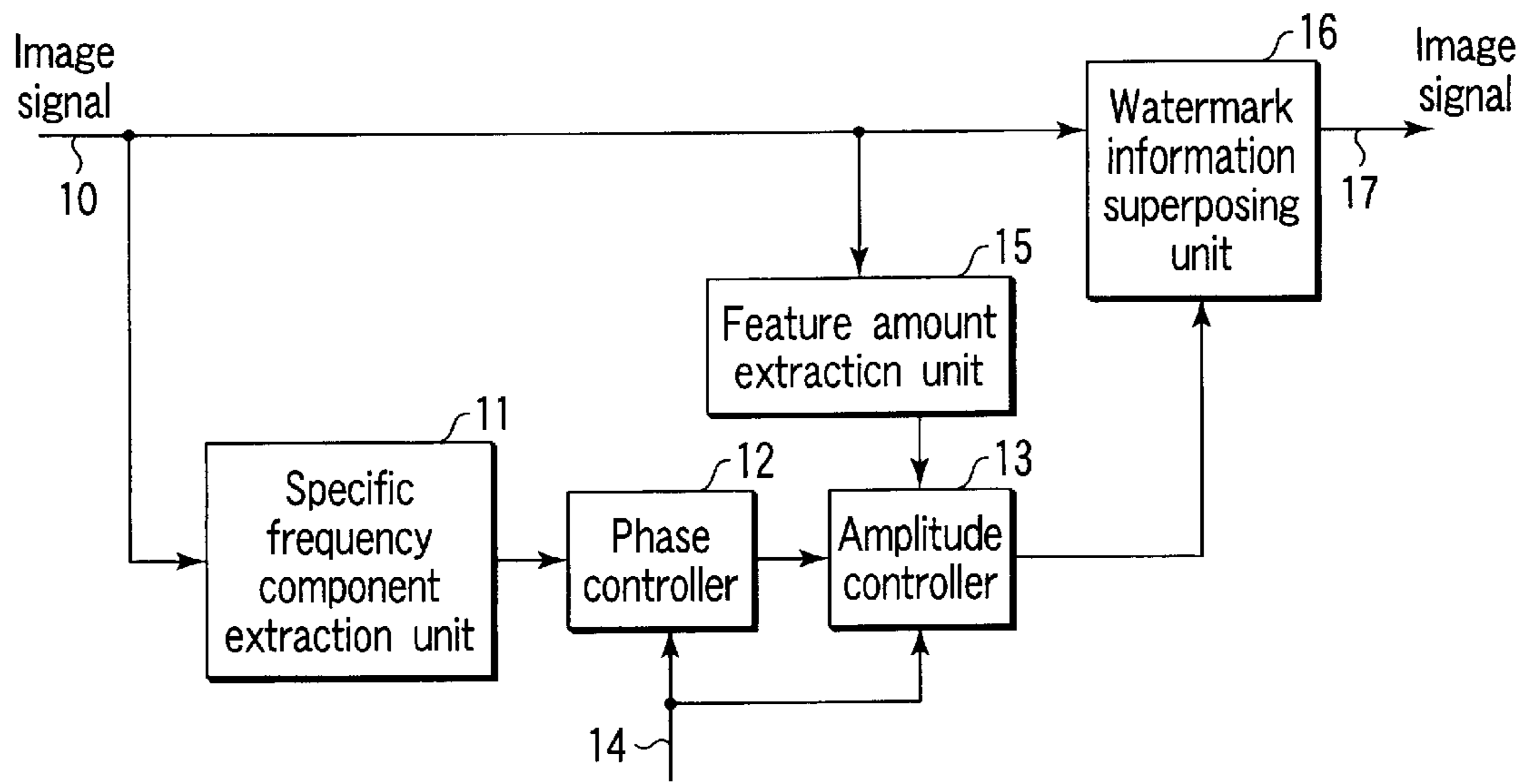
FIG. 1 Watermark information
