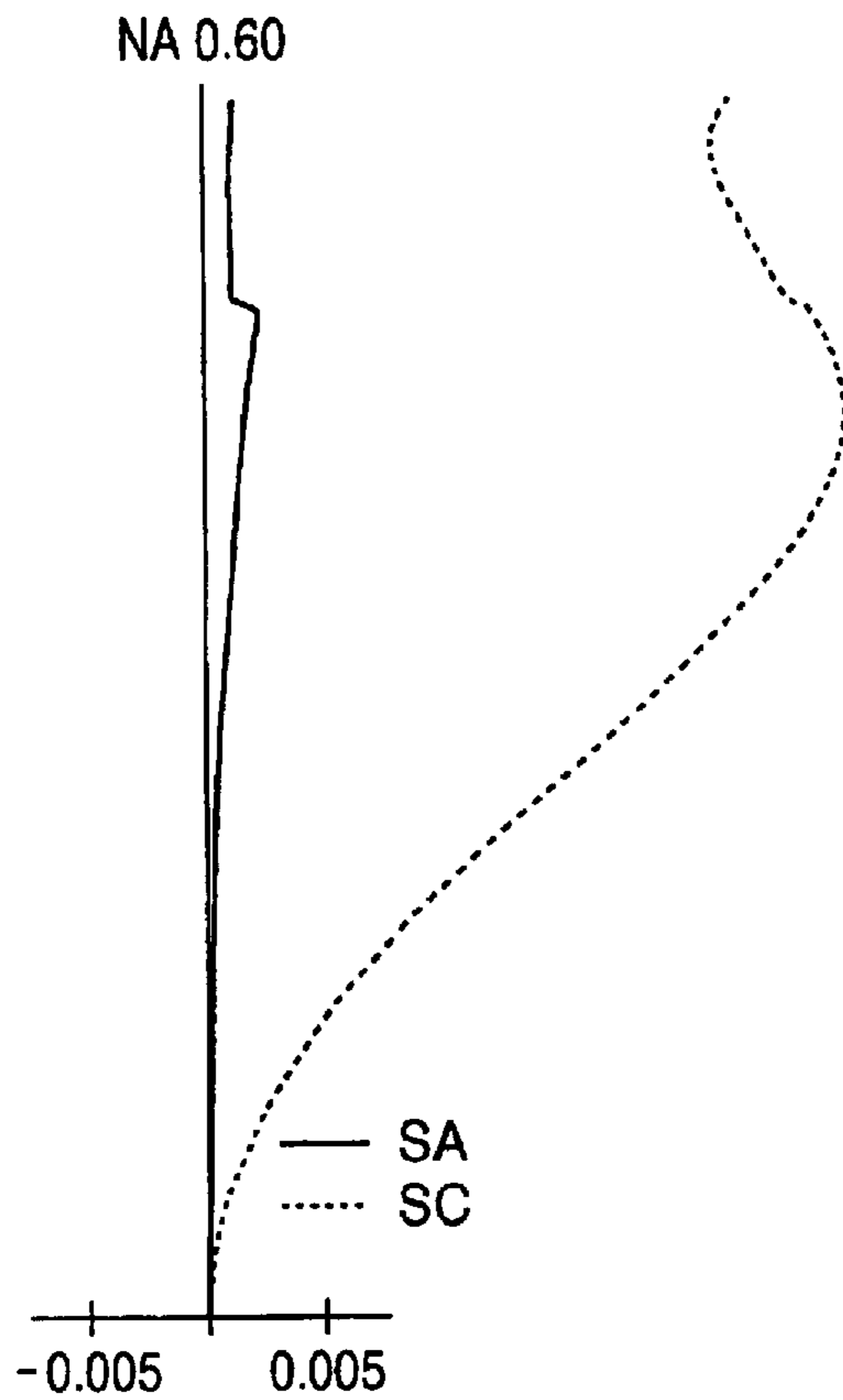
SPHERICAL ABERRATION SA SINE CONDITION SC
