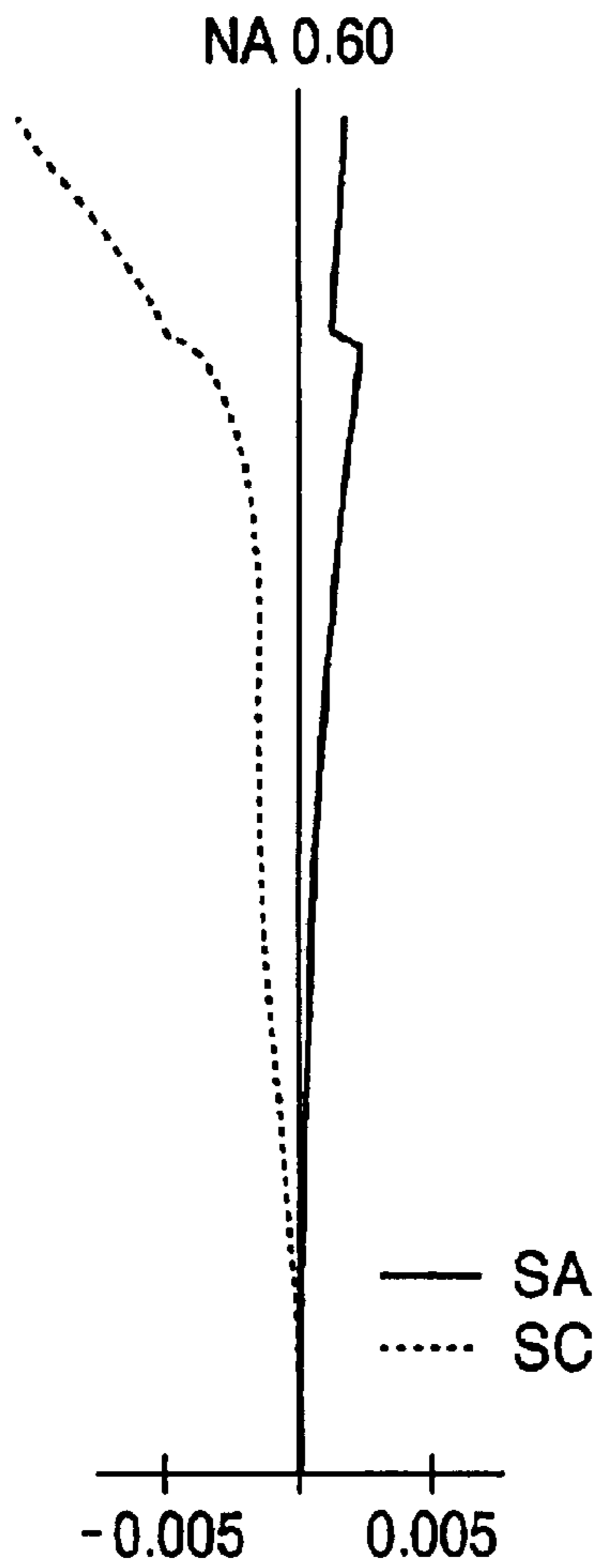
SPHERICAL ABERRATION SA SINE CONDITION SC
