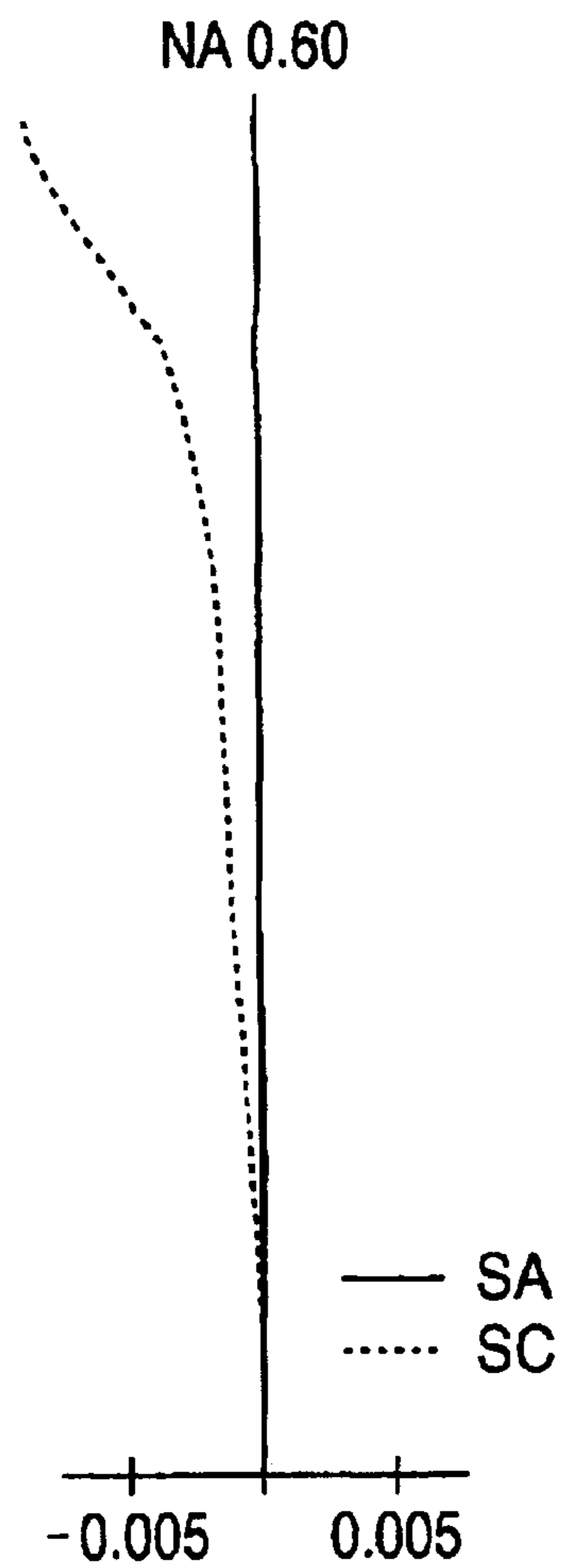
SPHERICAL ABERRATION SA SINE CONDITION SC
