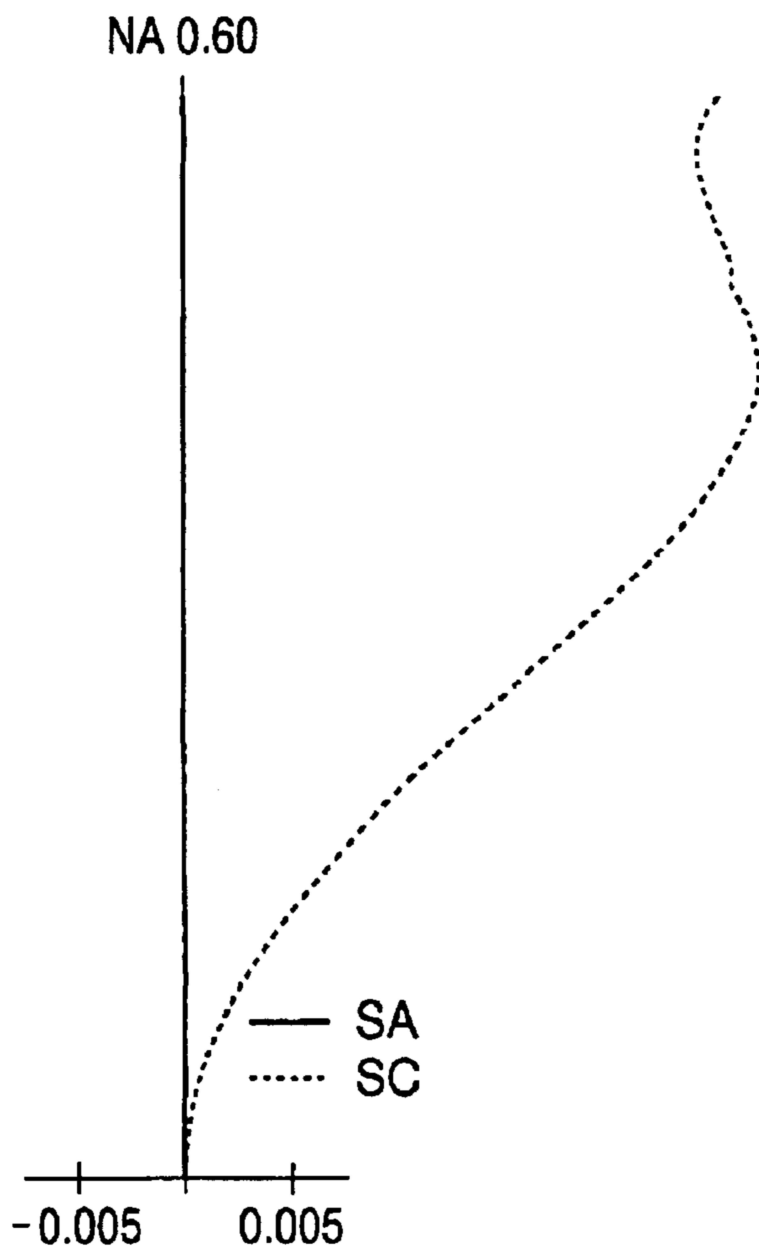
SPHERICAL ABERRATION SA SINE CONDITION SC
