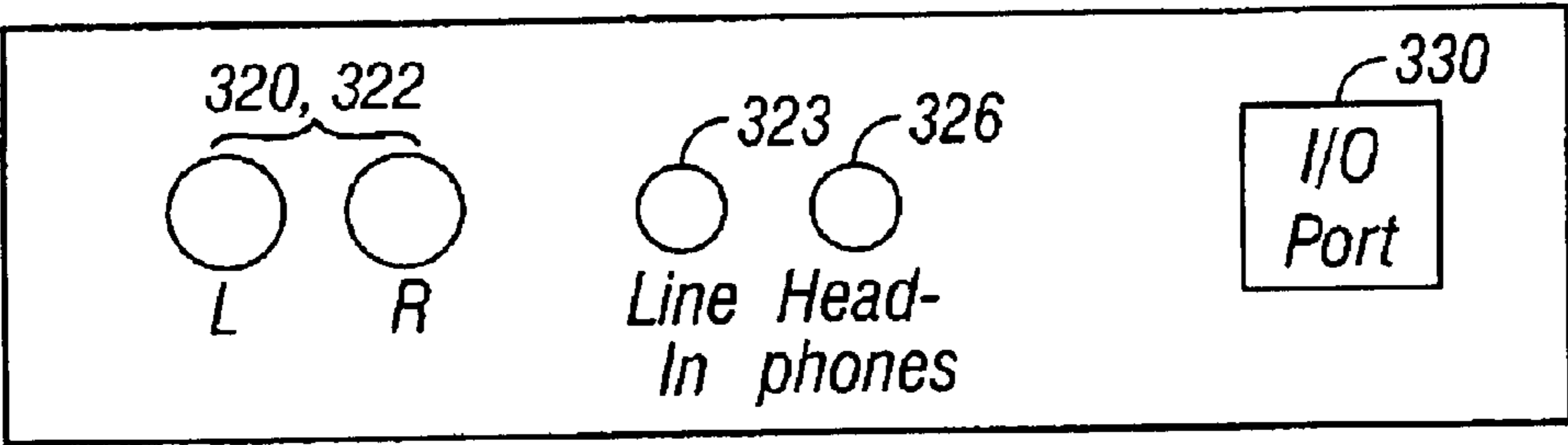
Back View FIG. 3c
