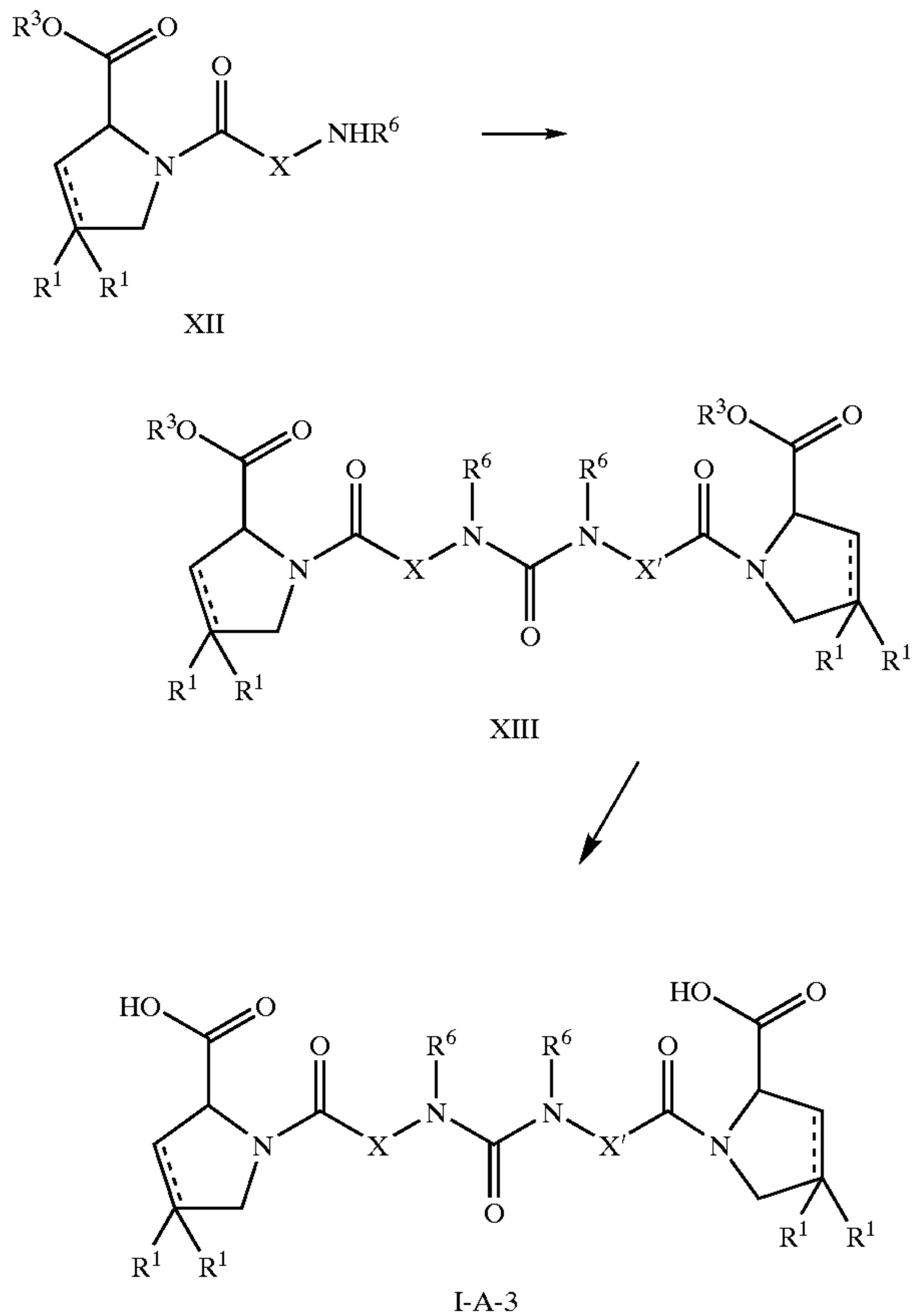
Scheme 4
