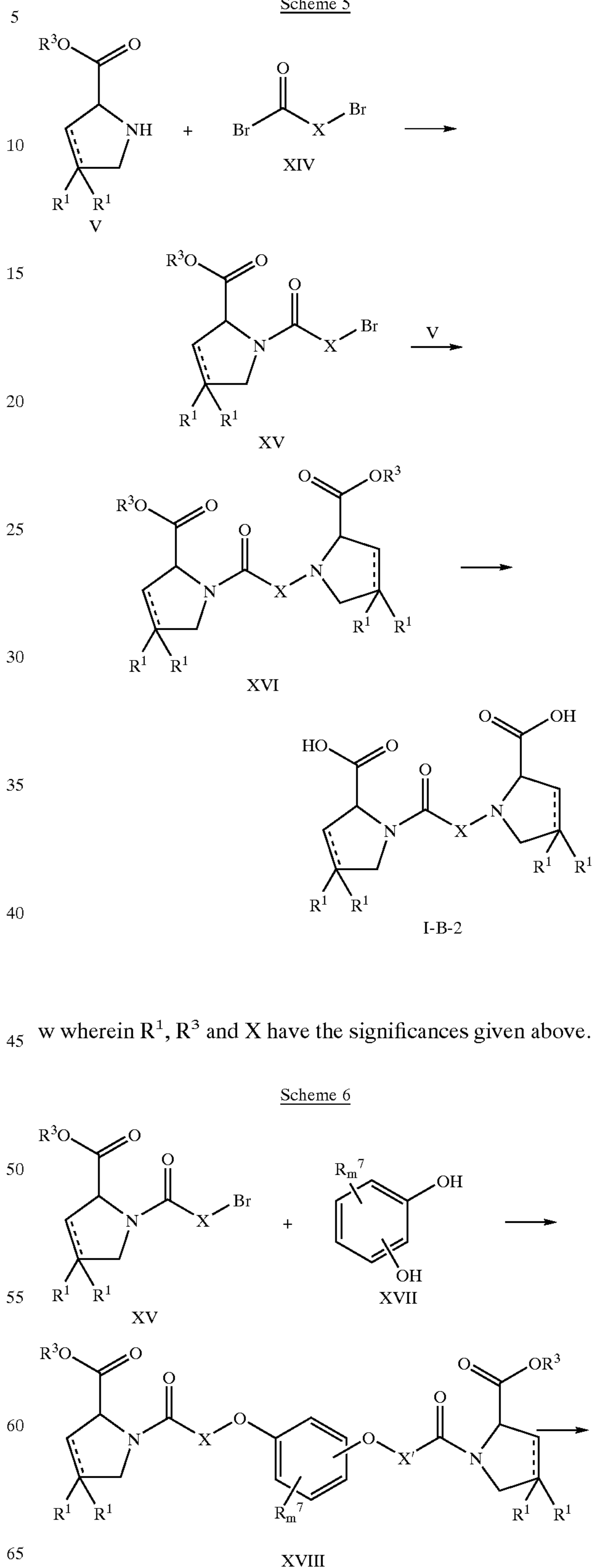
Scheme 5
