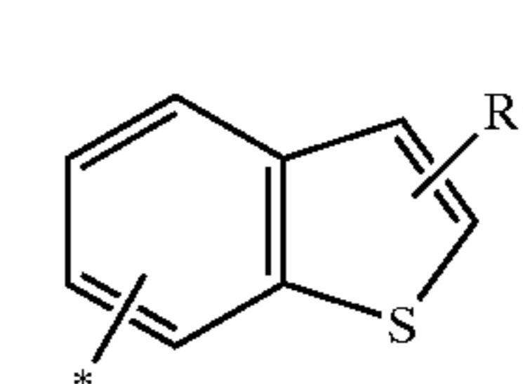
benzo[b]thienyl
