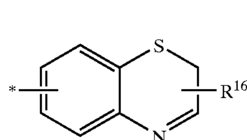
1,4-benzothiazinyl
