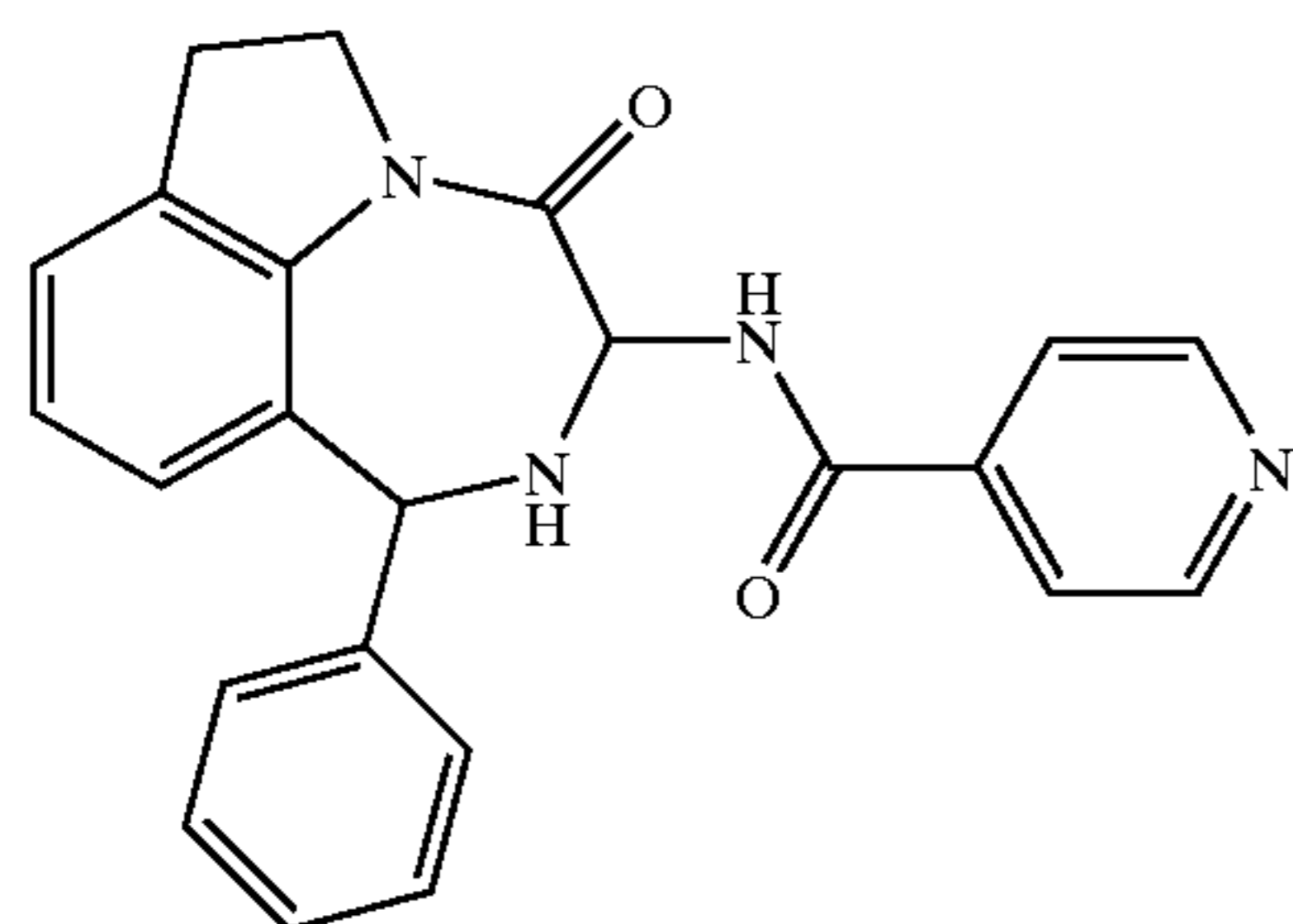
PD-168787
