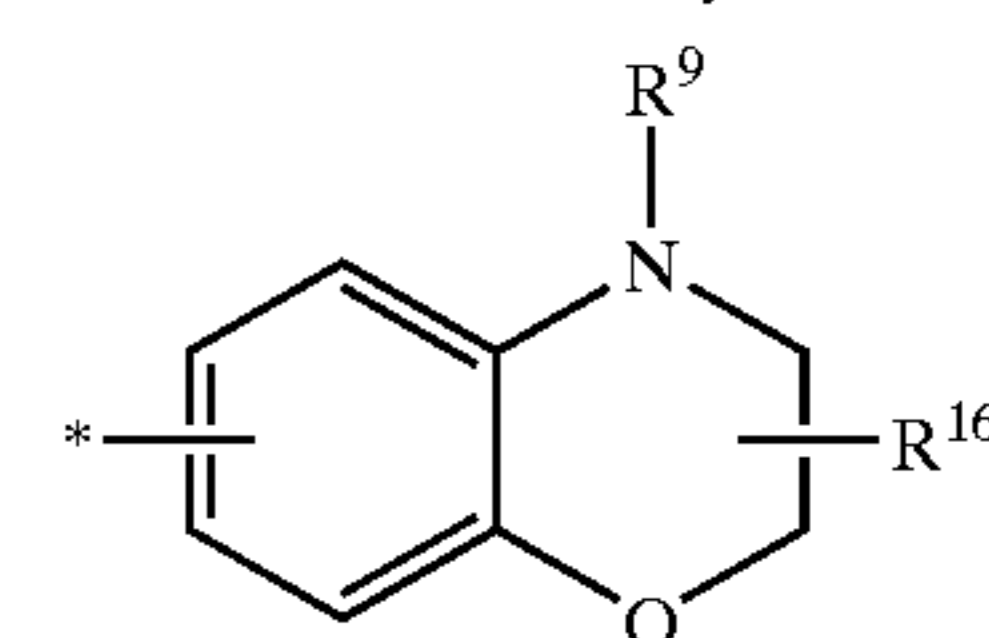
1,4-benzodioxanyl
