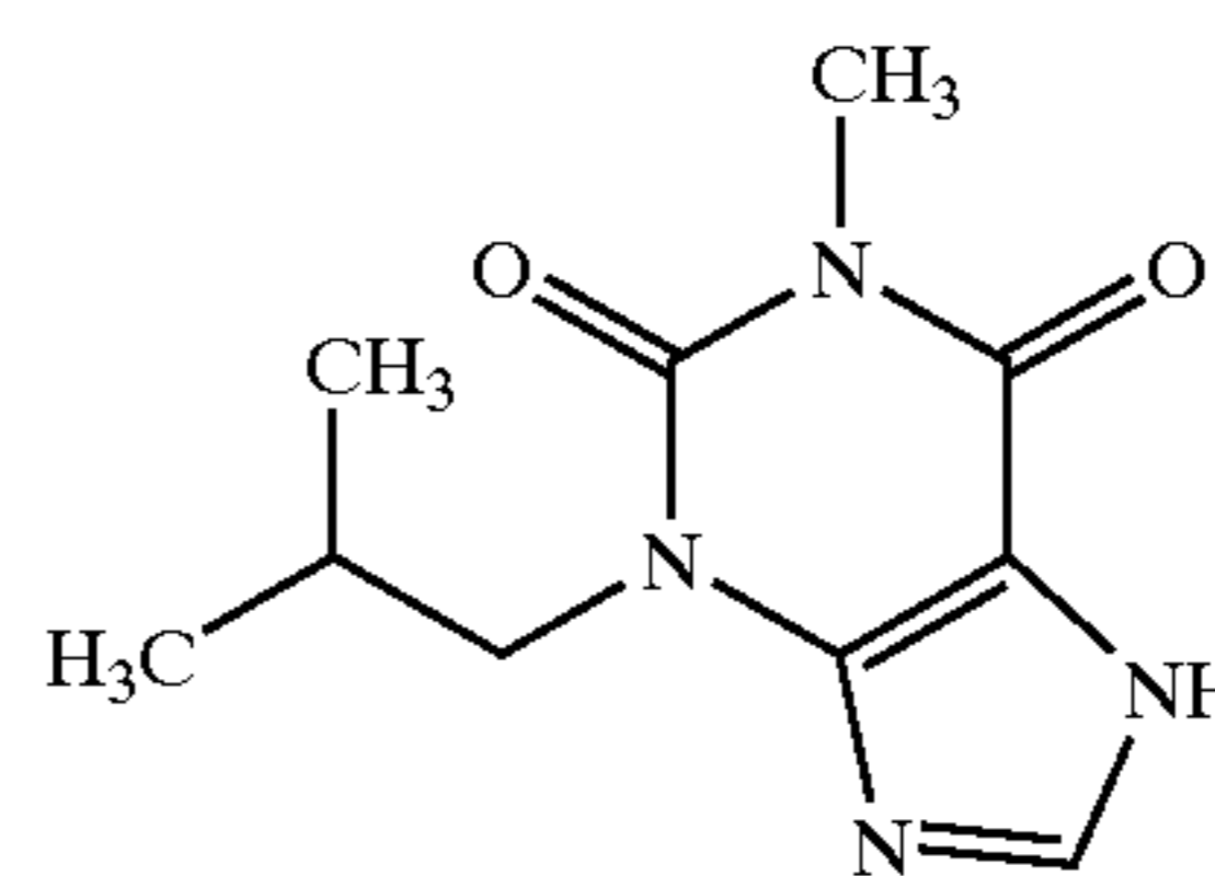
IBMX
