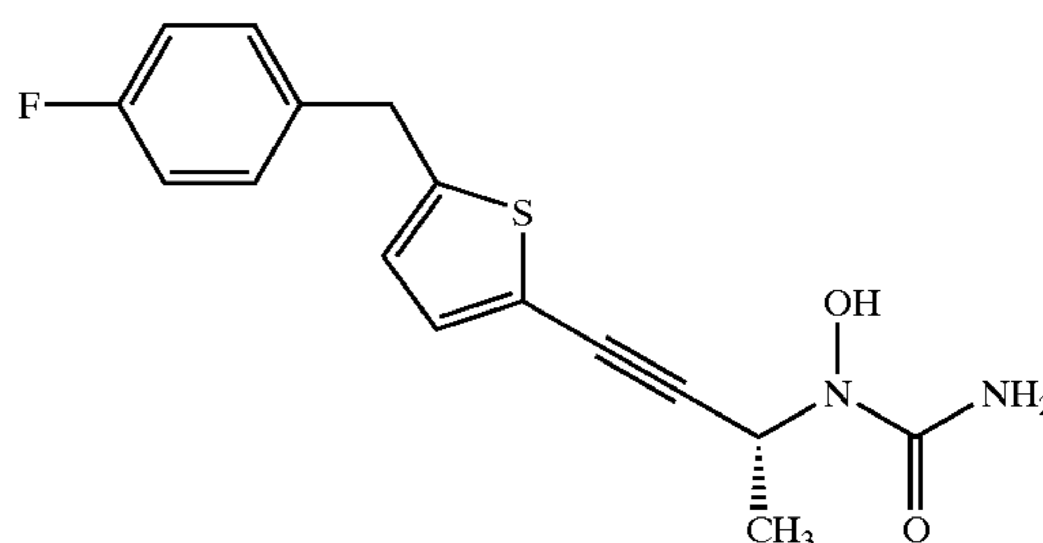
ABT-761
