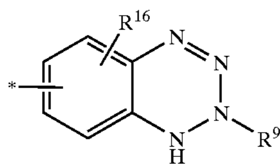
benzotetrazinyl
