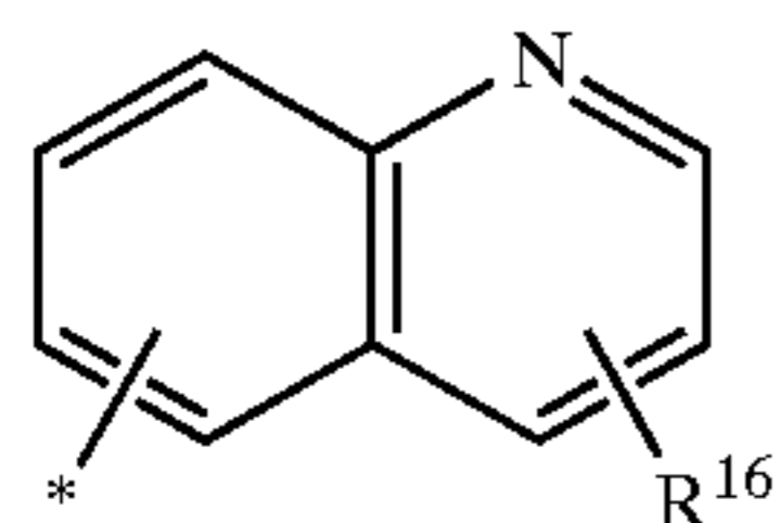
quinolinylyl
