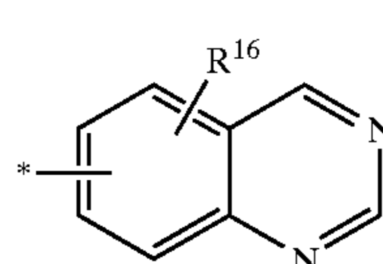
quinazolinylyl
