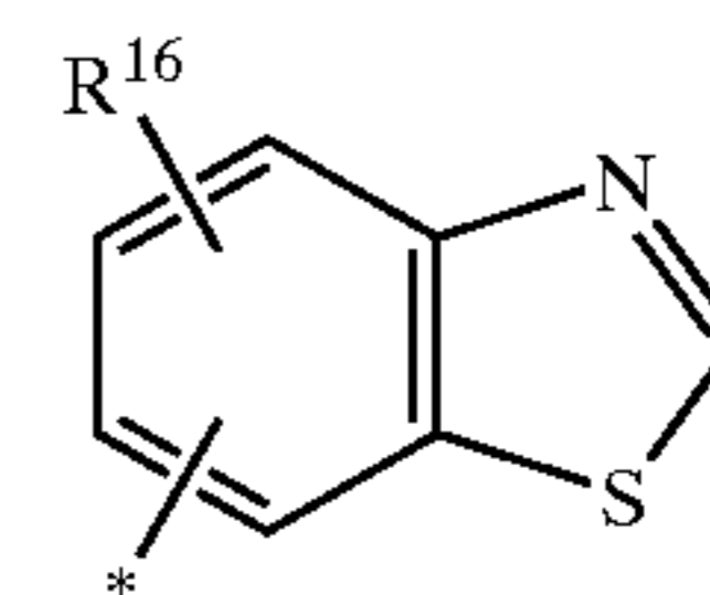
benzothiazolyl
