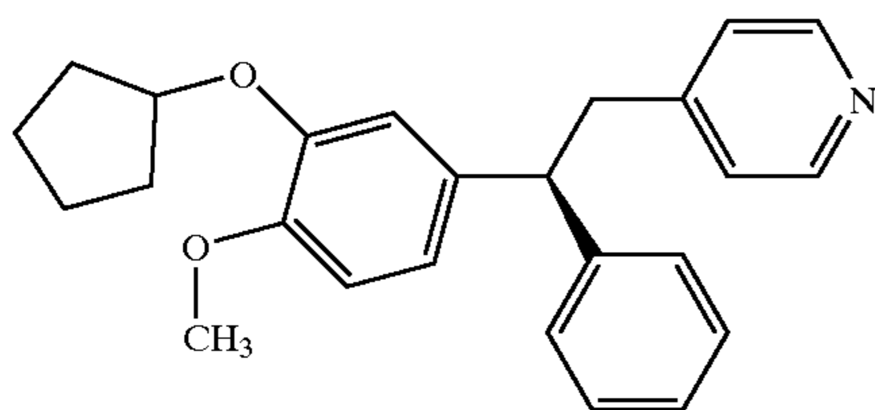
CT-1731
