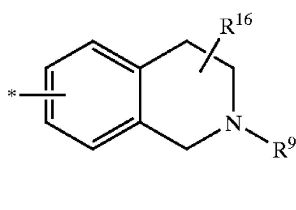
1,2,3,4-tetrahydroisoquinolinylyl
