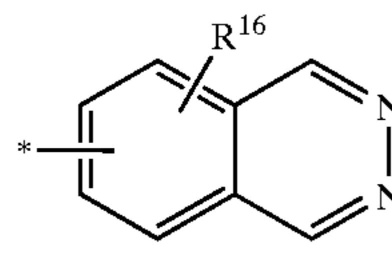
phthalazinyl
