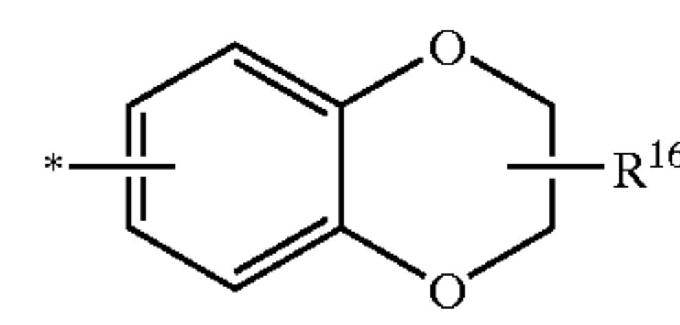
1,4-benzodioxanyl
