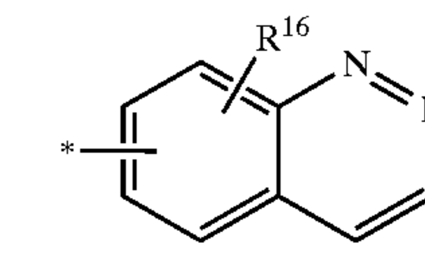
cinnolinylyl
