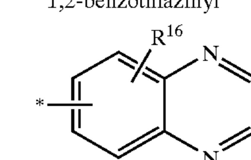
quinoxalinylyl
