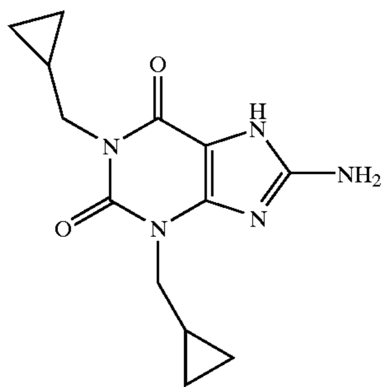
Cipamfylline (BRL-61,063)
