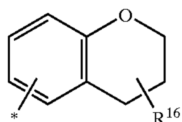
chromanyl
