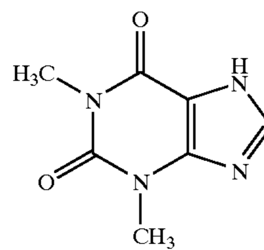
Theophylline
