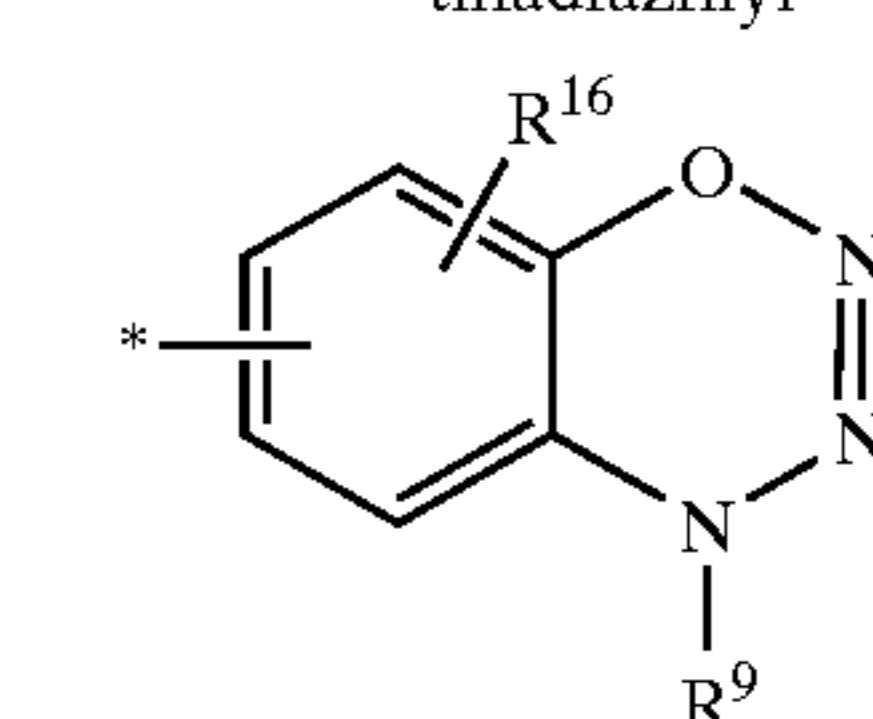
benzotriazinyl
