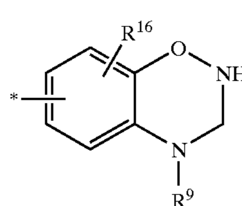
2H-1,2,4-benzoxadiazinyl
