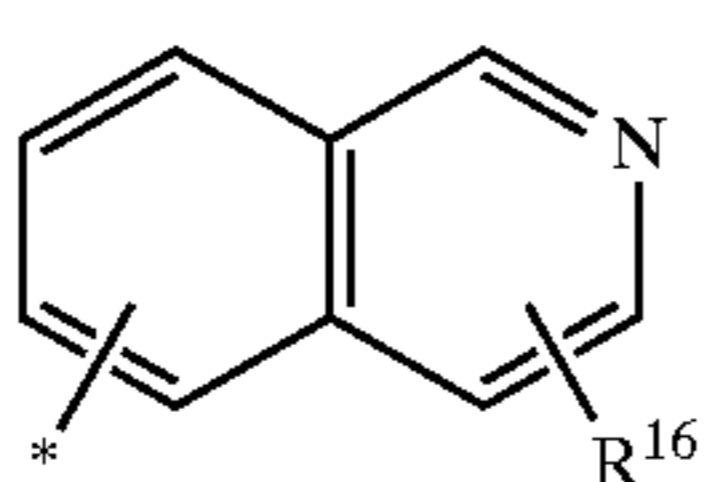
isoquinolinylyl
