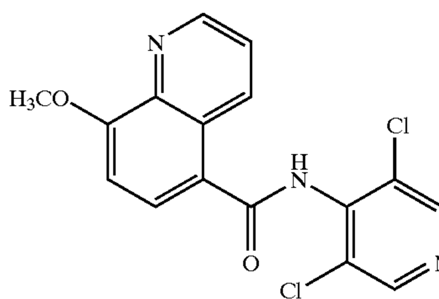
D4418
