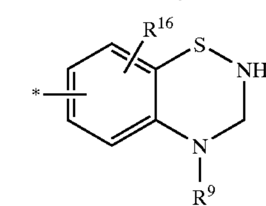
2H-1,2,4-benzothiadiazinyl
