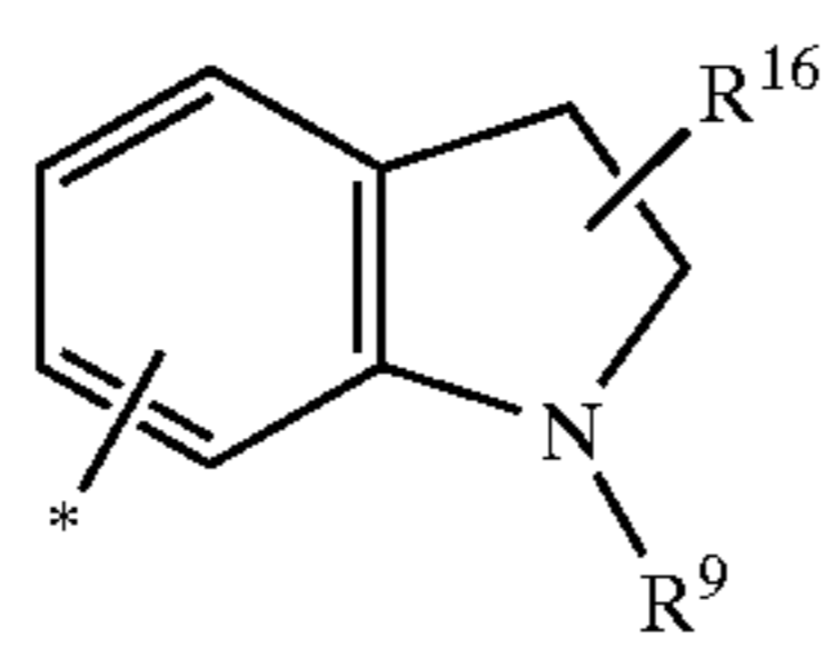
indolinyl
