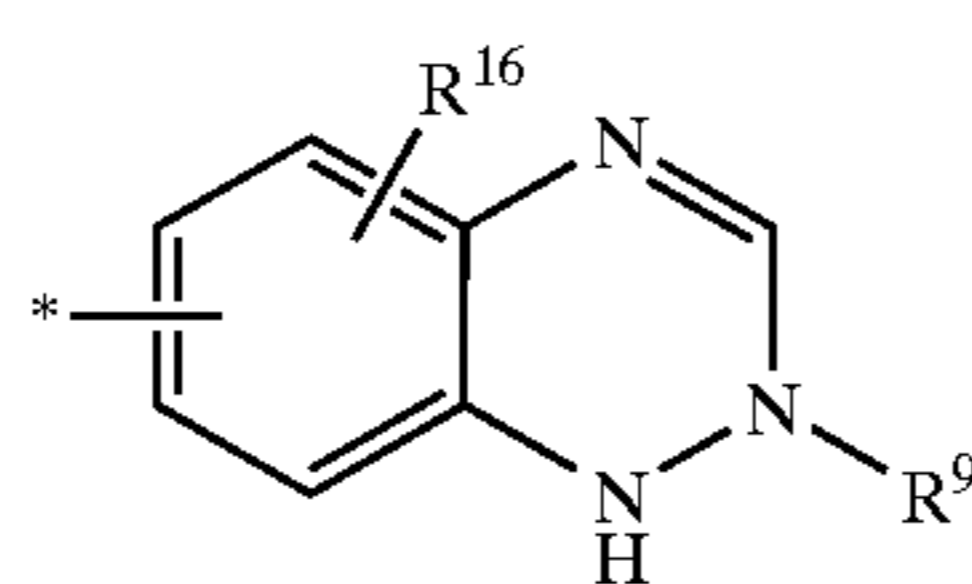
1,2,4-benzotriazinyl
