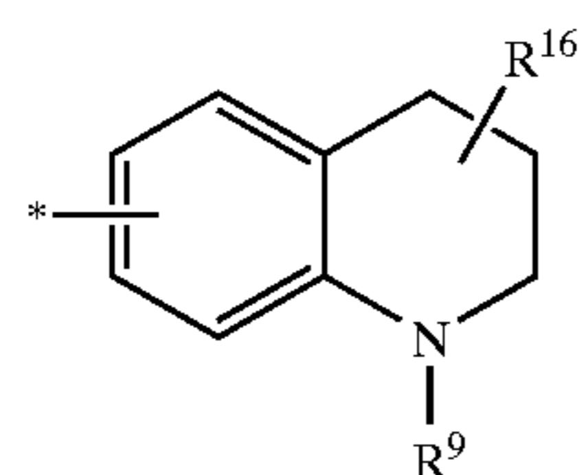
1,2,3,4-tetrahydroquinolinylyl
