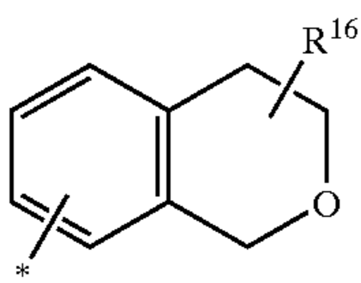
isochromanyl
