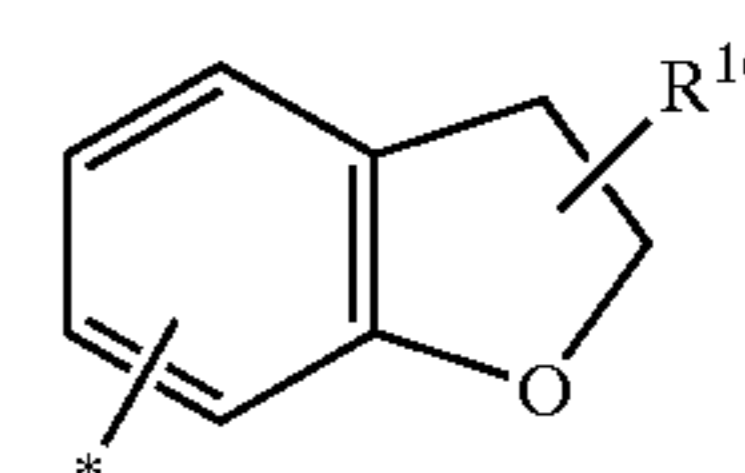
2,3-dihydrobenzofuranyl
