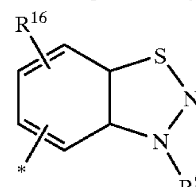
phthalazinyl
