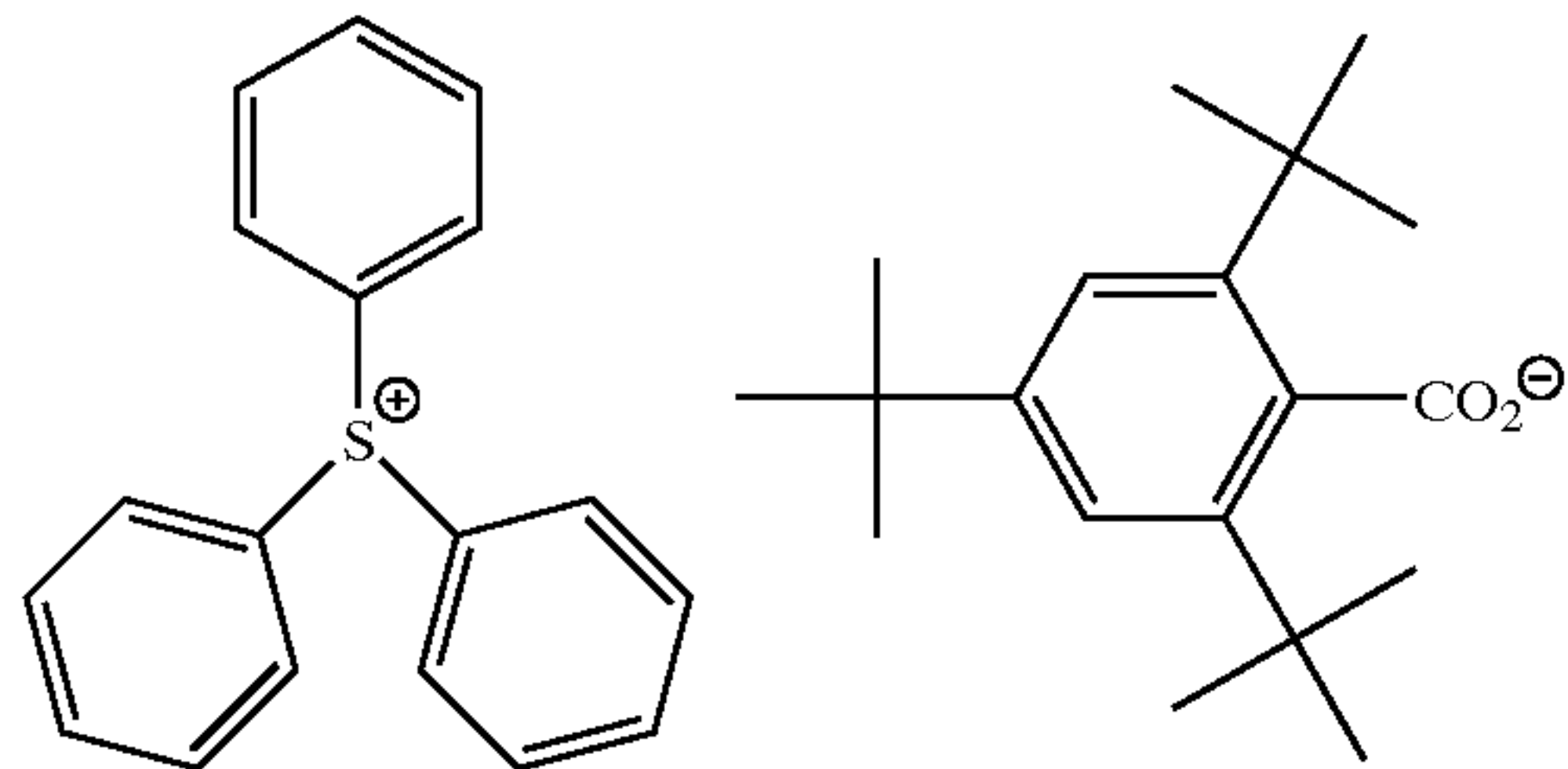
Structure of Sulfonium Salt Compound TN-2:
