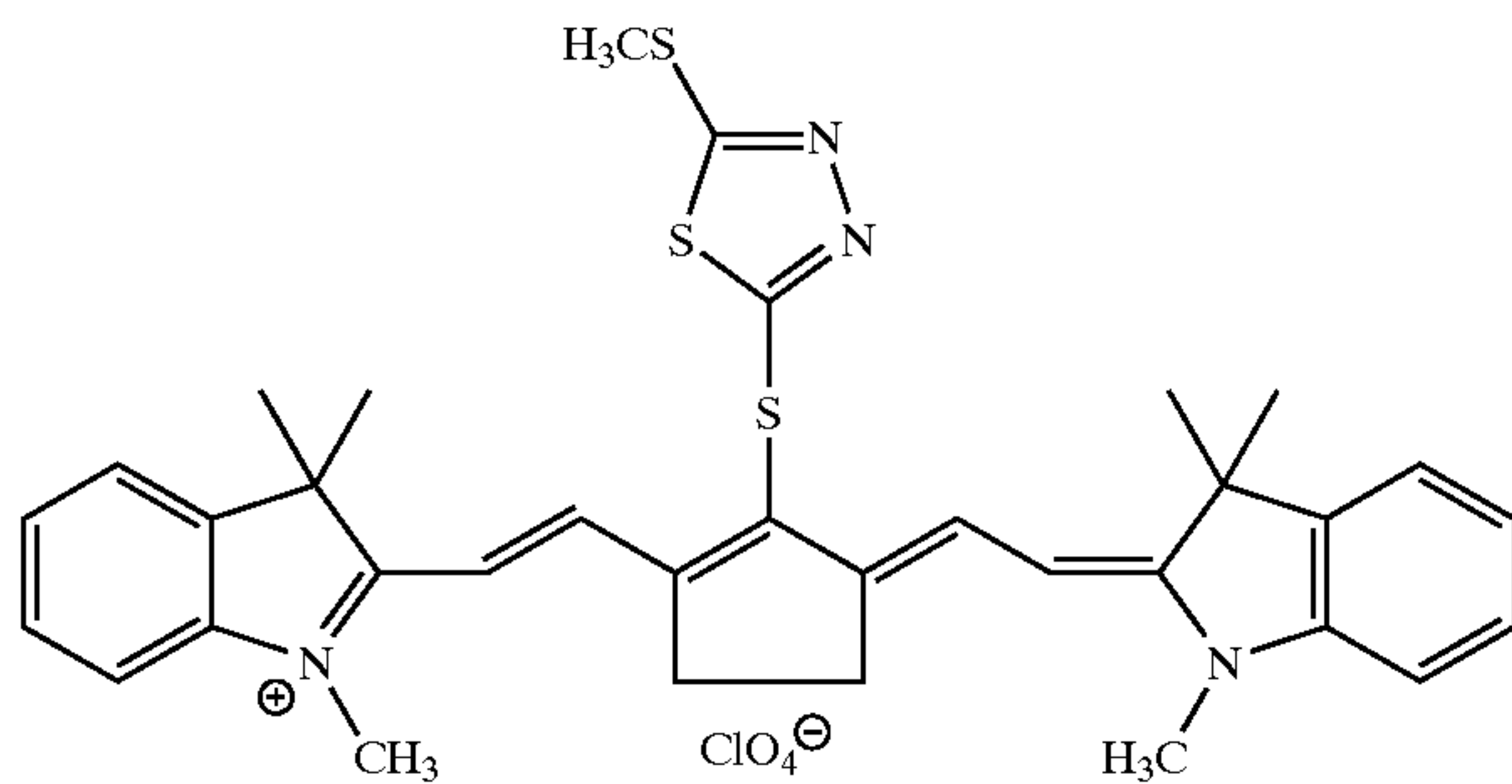
Structure of Sulfonium Salt Compound TN-2:
