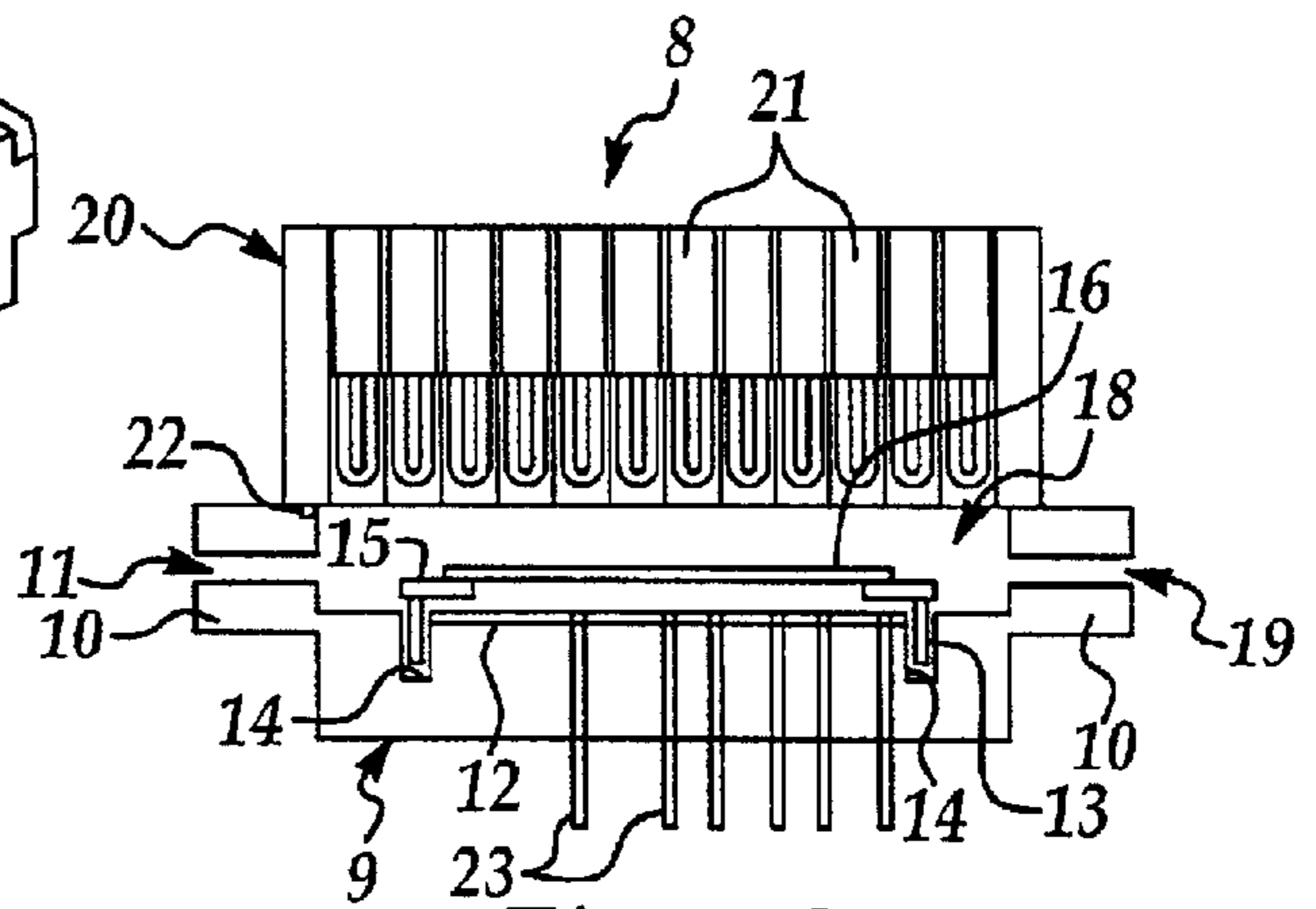
Figure 2 Prior Art
