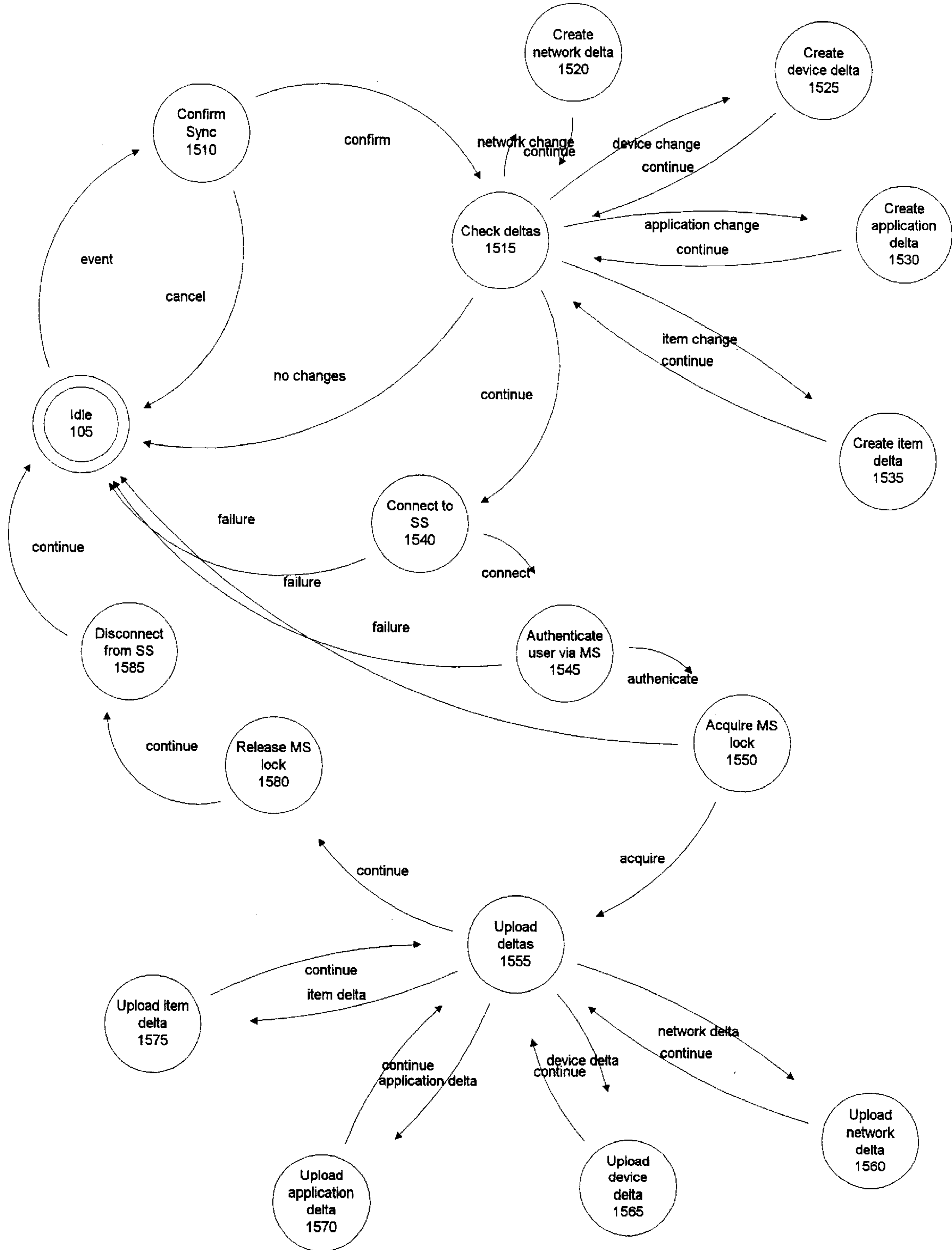
Figure 16 Push Synchronization
