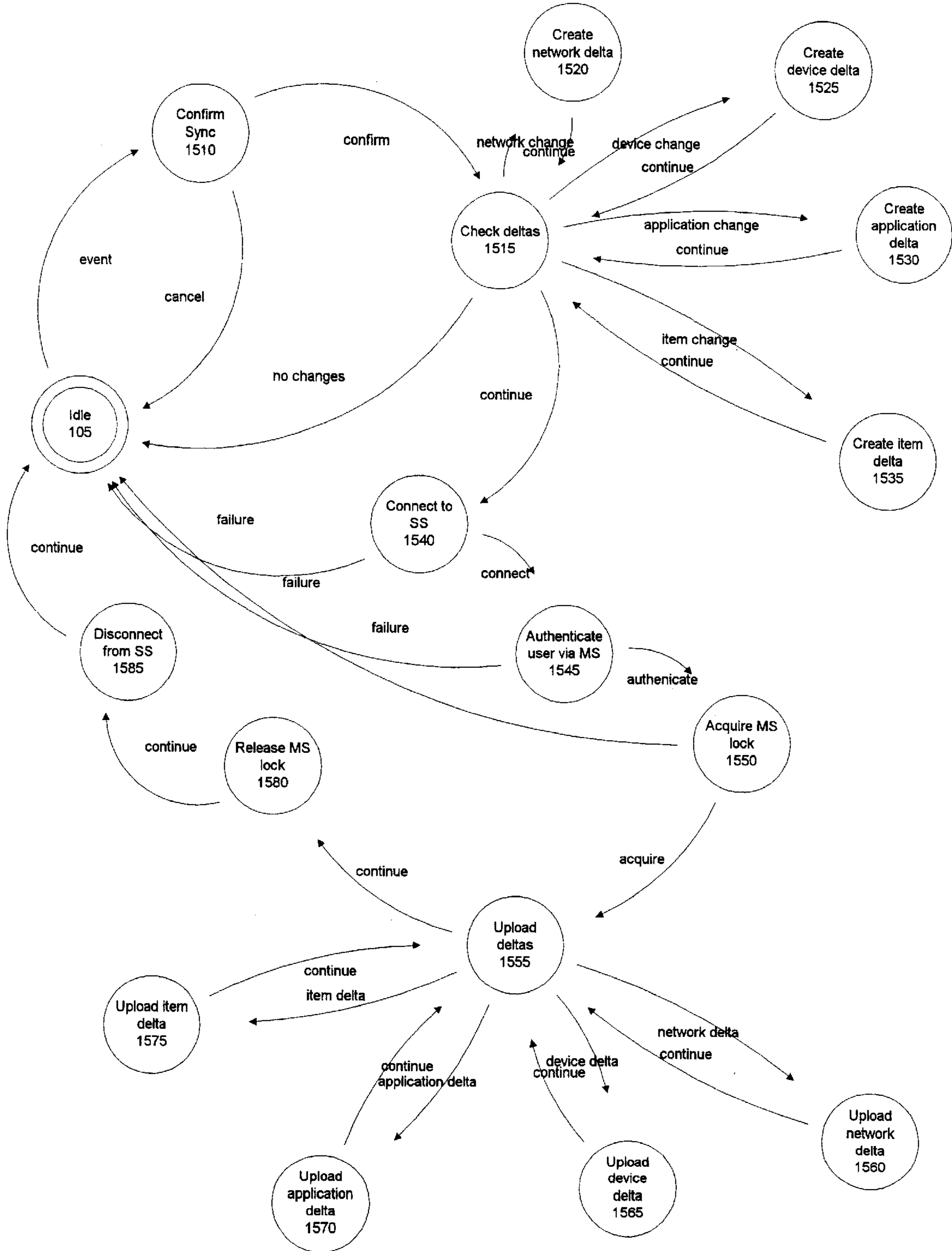
Figure 16 Push Synchronization
