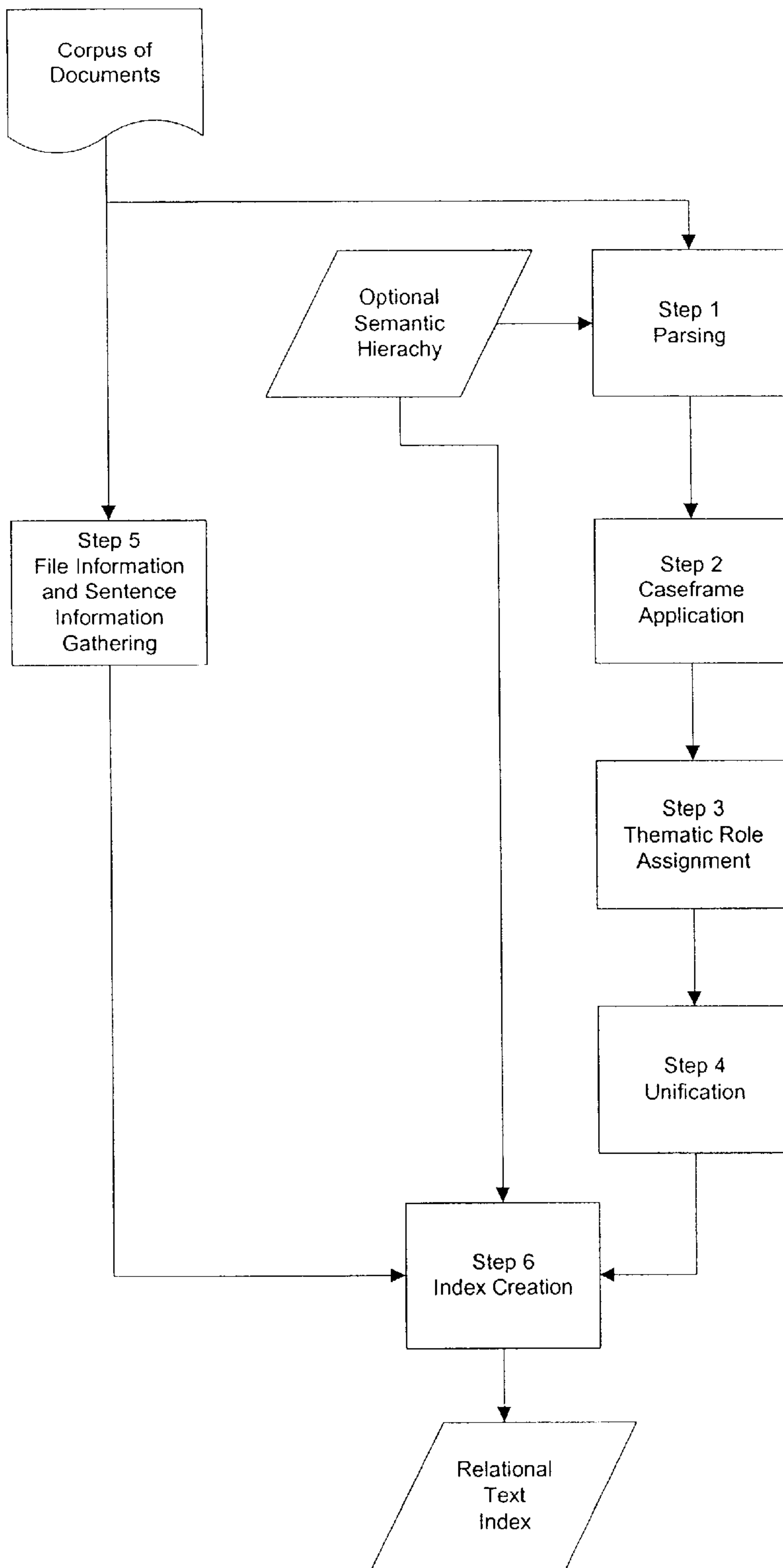
Figure 3 Index Creation Algorithm, High Level
