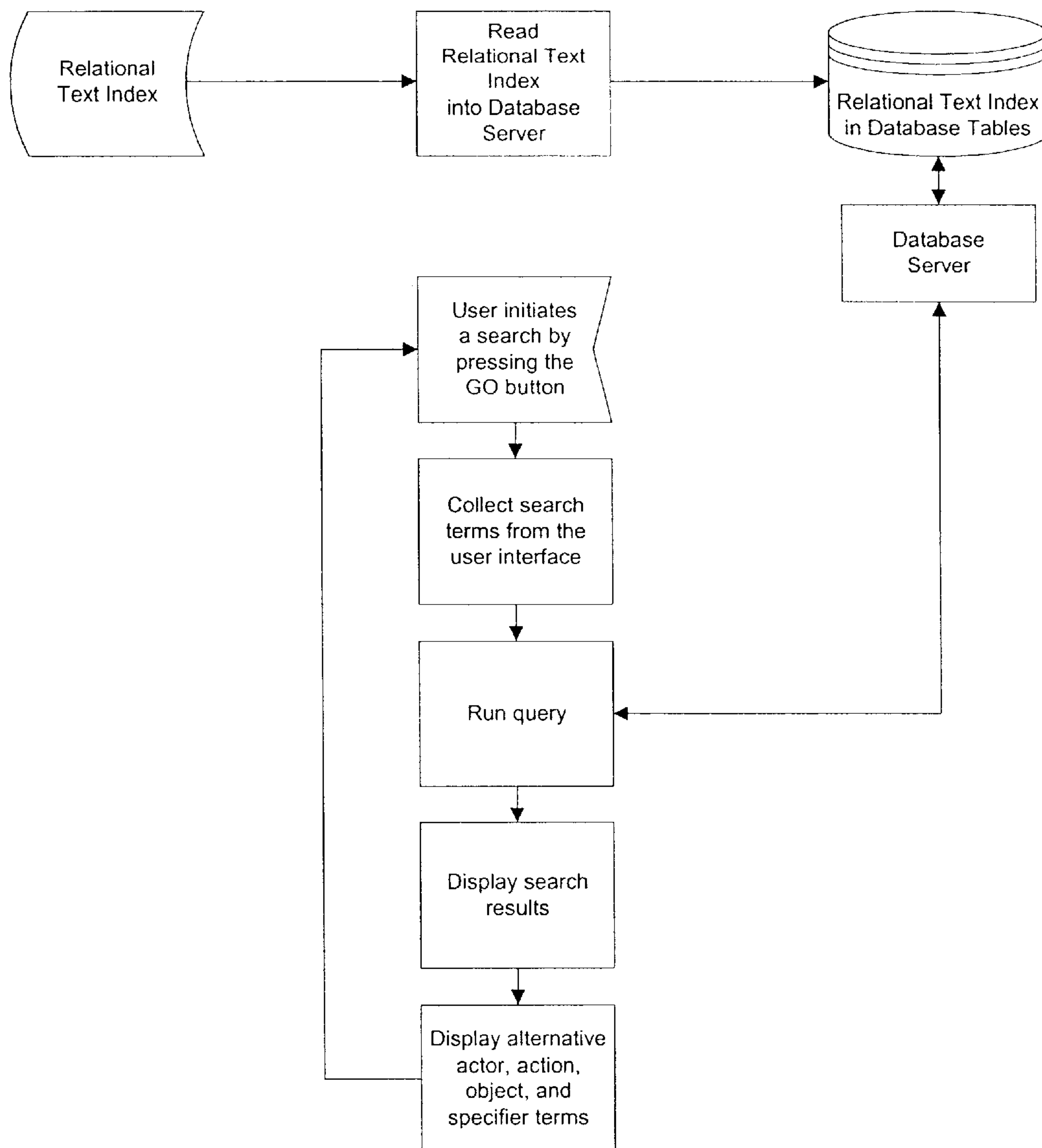
Figure 6 Flowchart – PowerDrill
