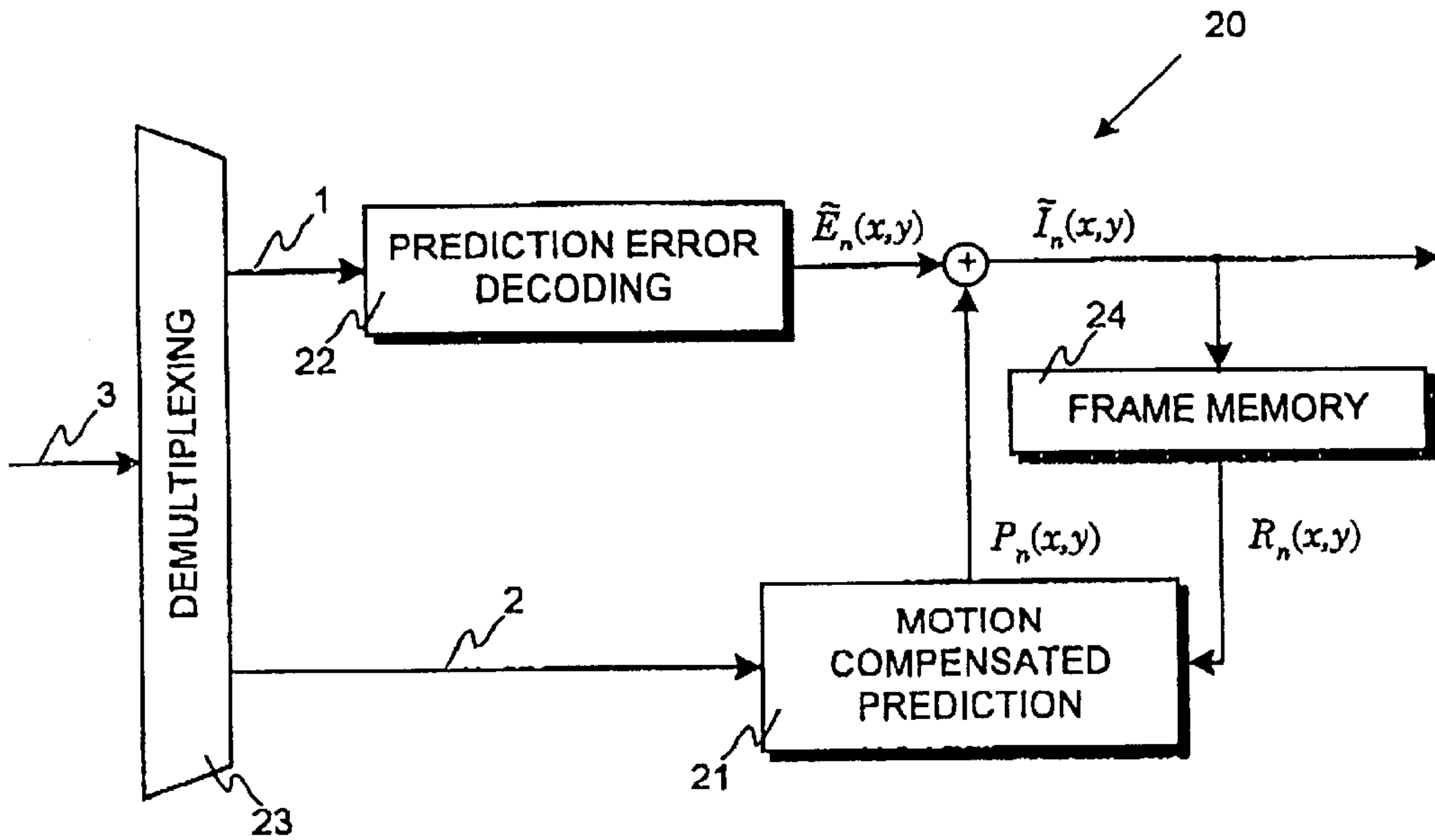
FIG. 2 PRIOR ART
