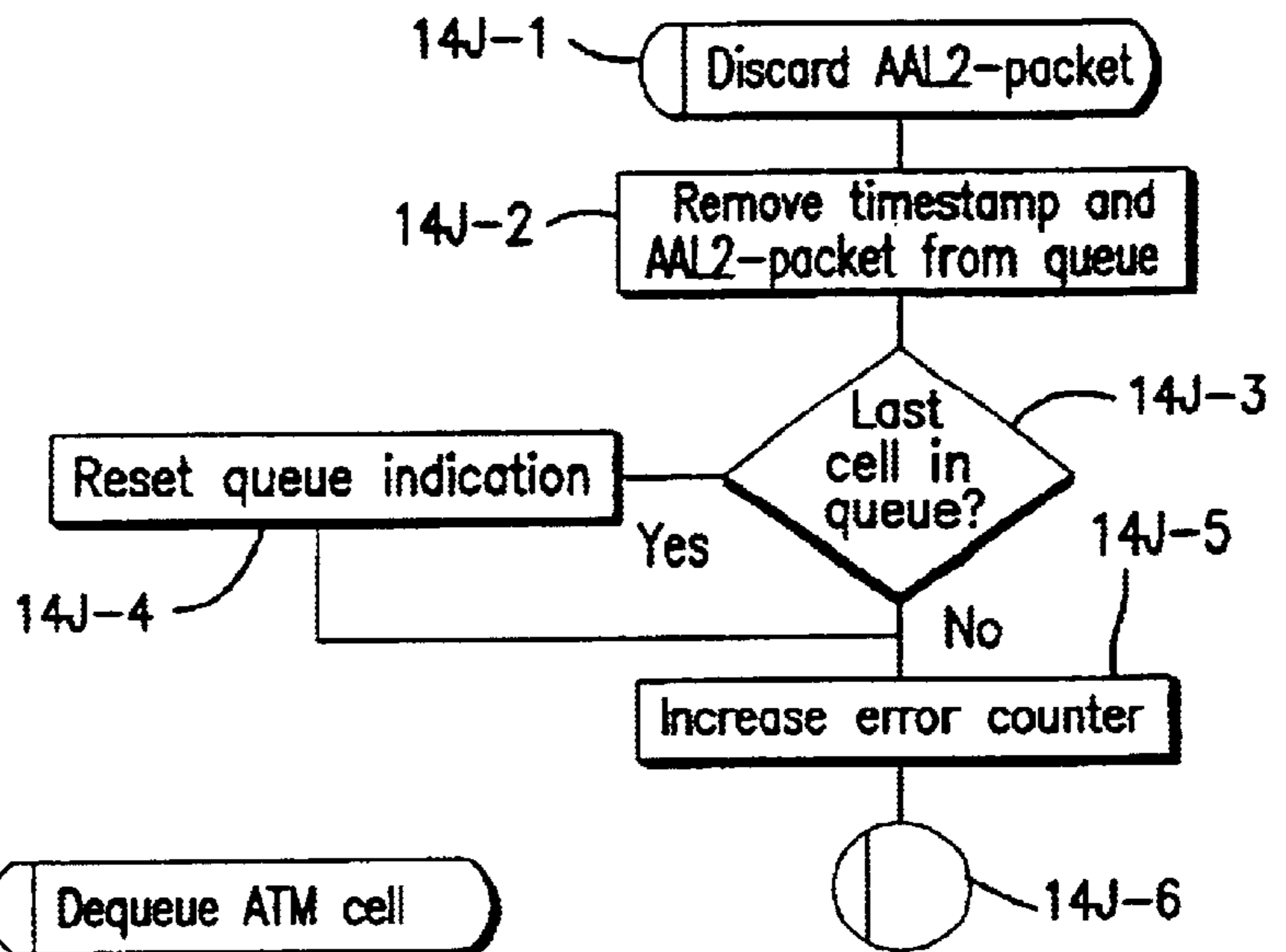
FIG. 14J DISCARD AAL2 PACKET FUNCTION
