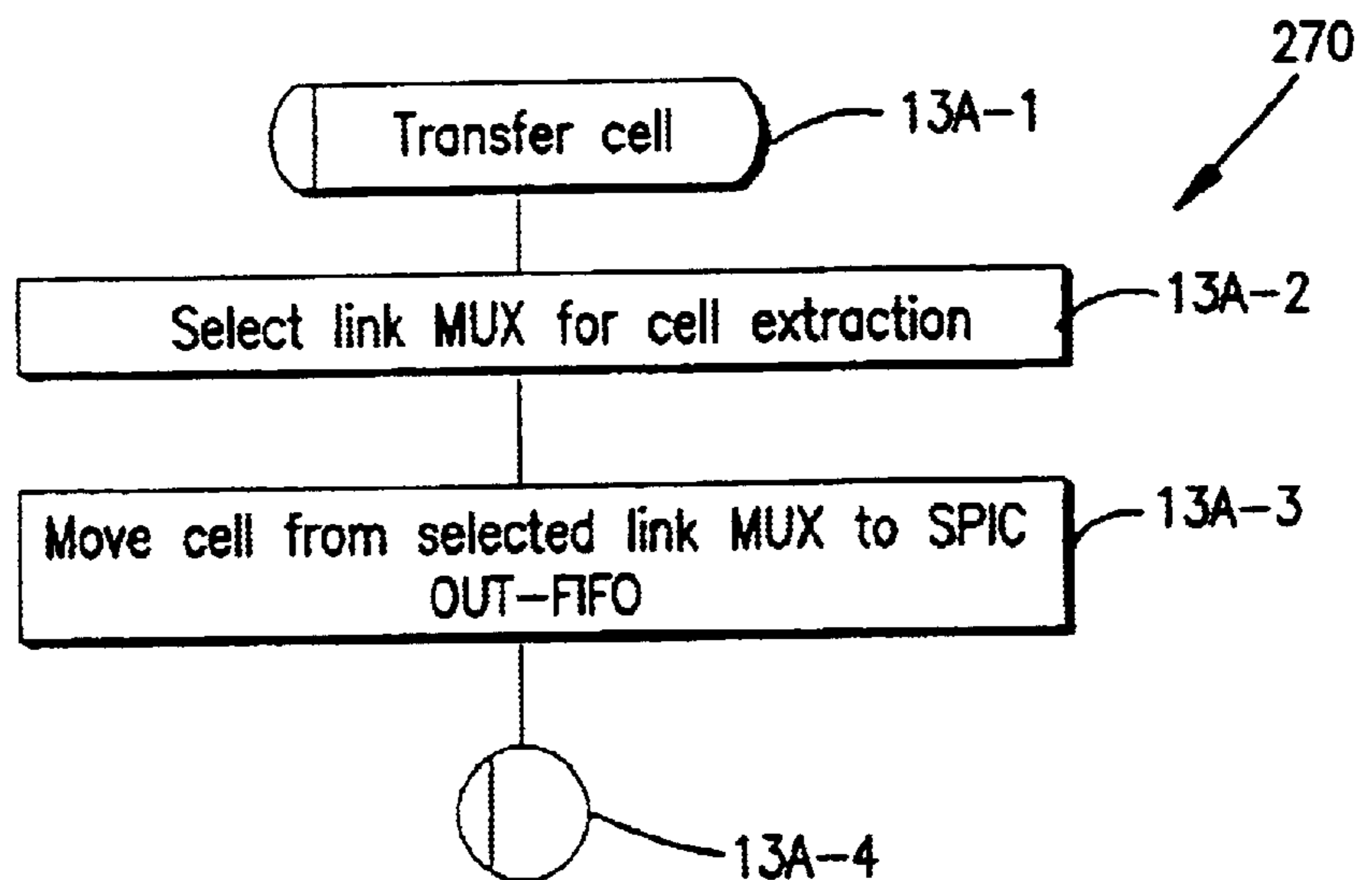
FIG. 13A TRANSFER CELL FUNCTION
