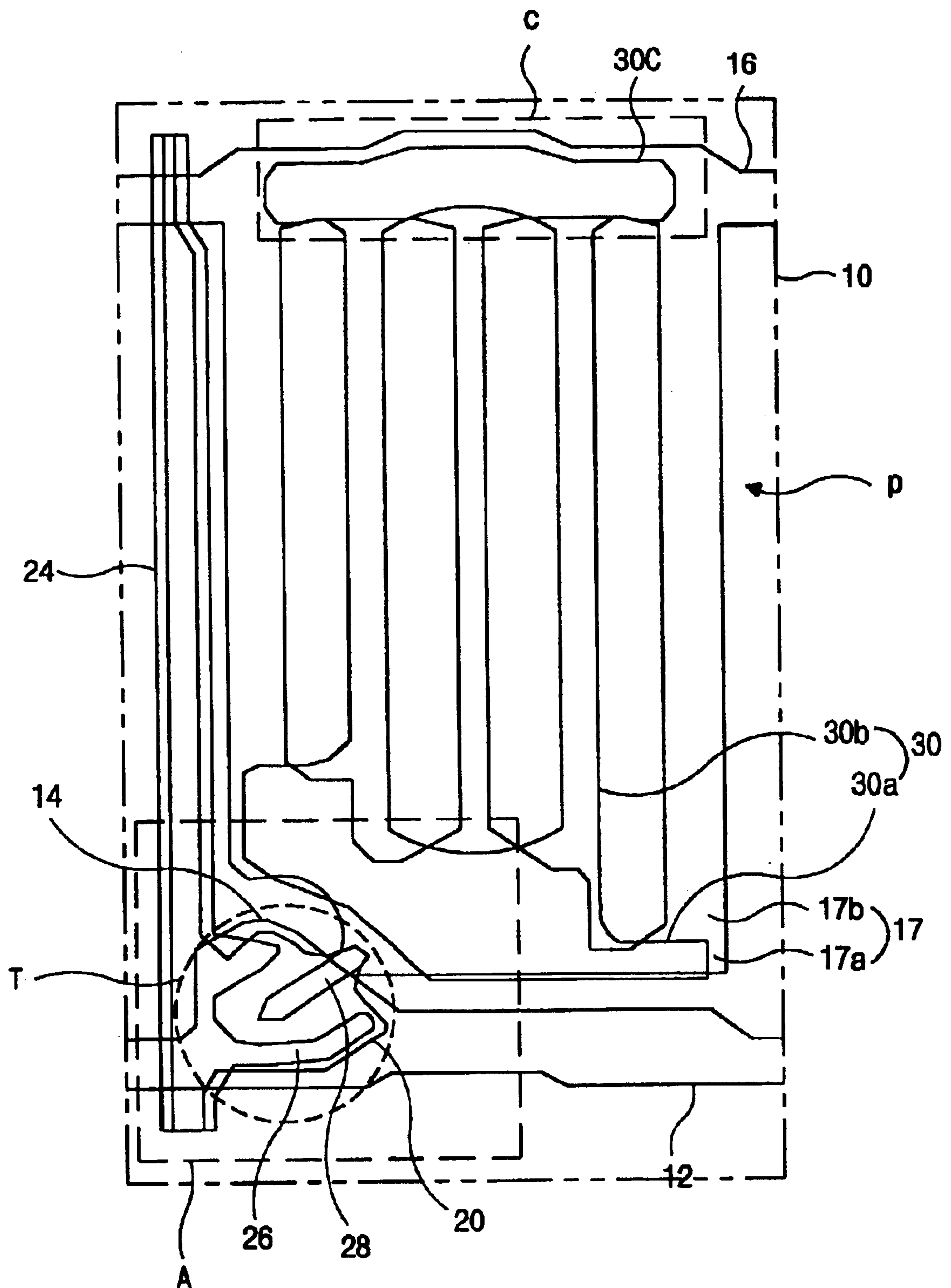
FIG. 1 (RELATED ART)
