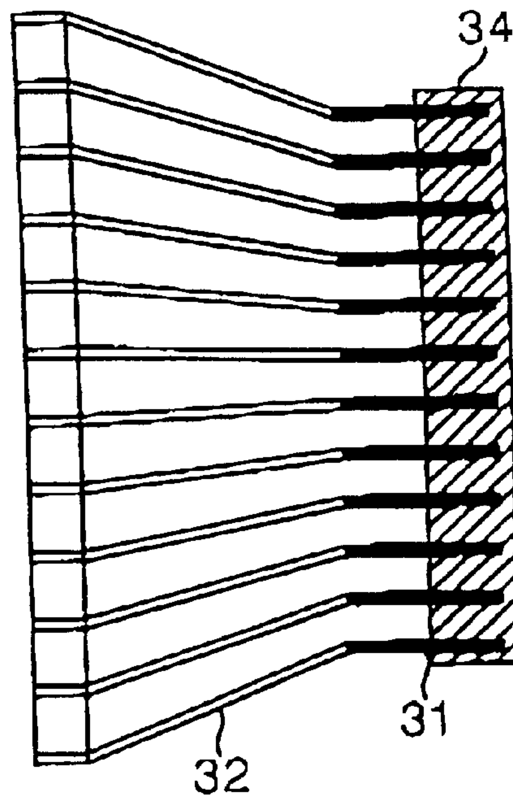
FIG. 4 CONVENTIONAL ART
