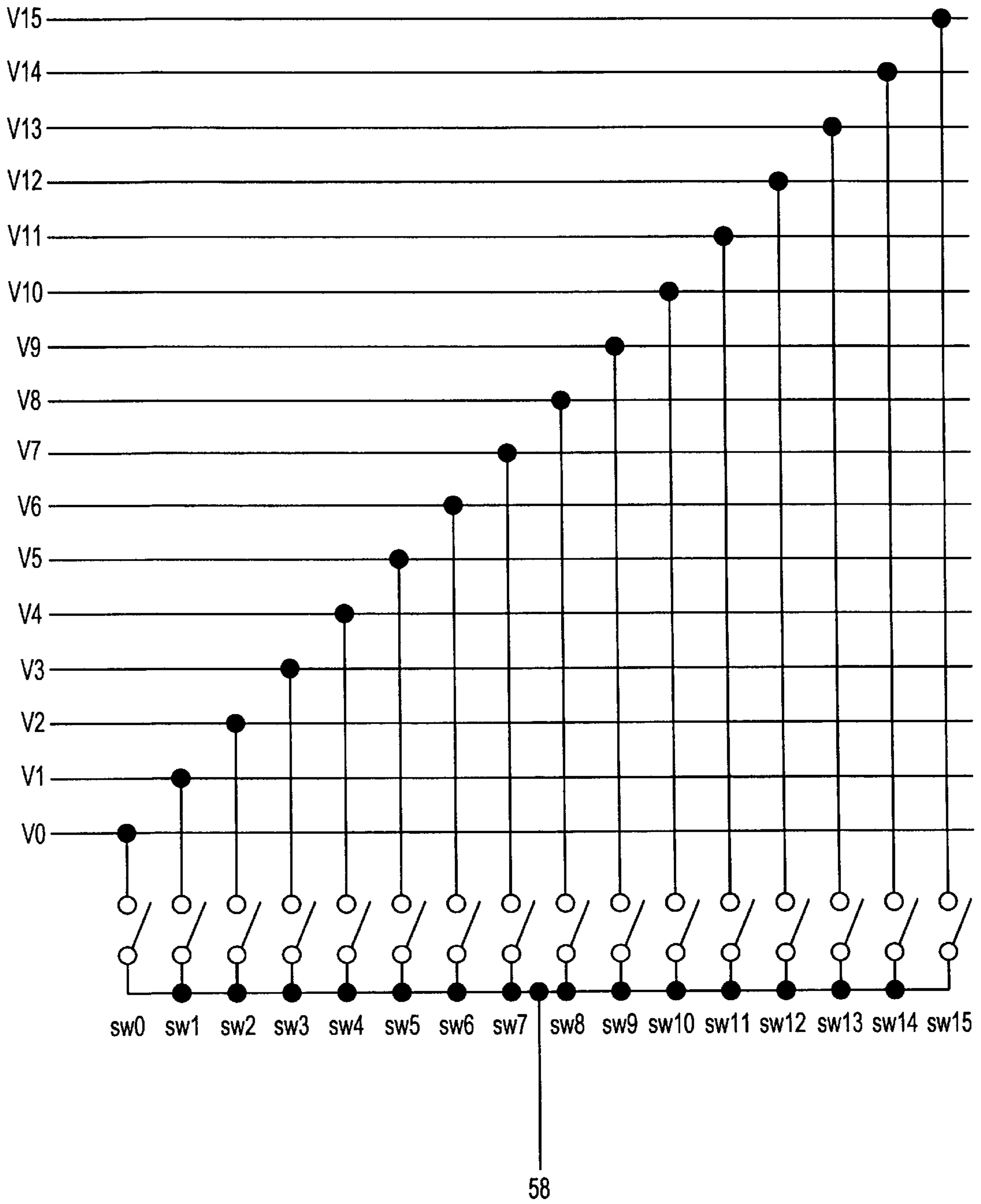
FIG. 35 PRIOR ART
