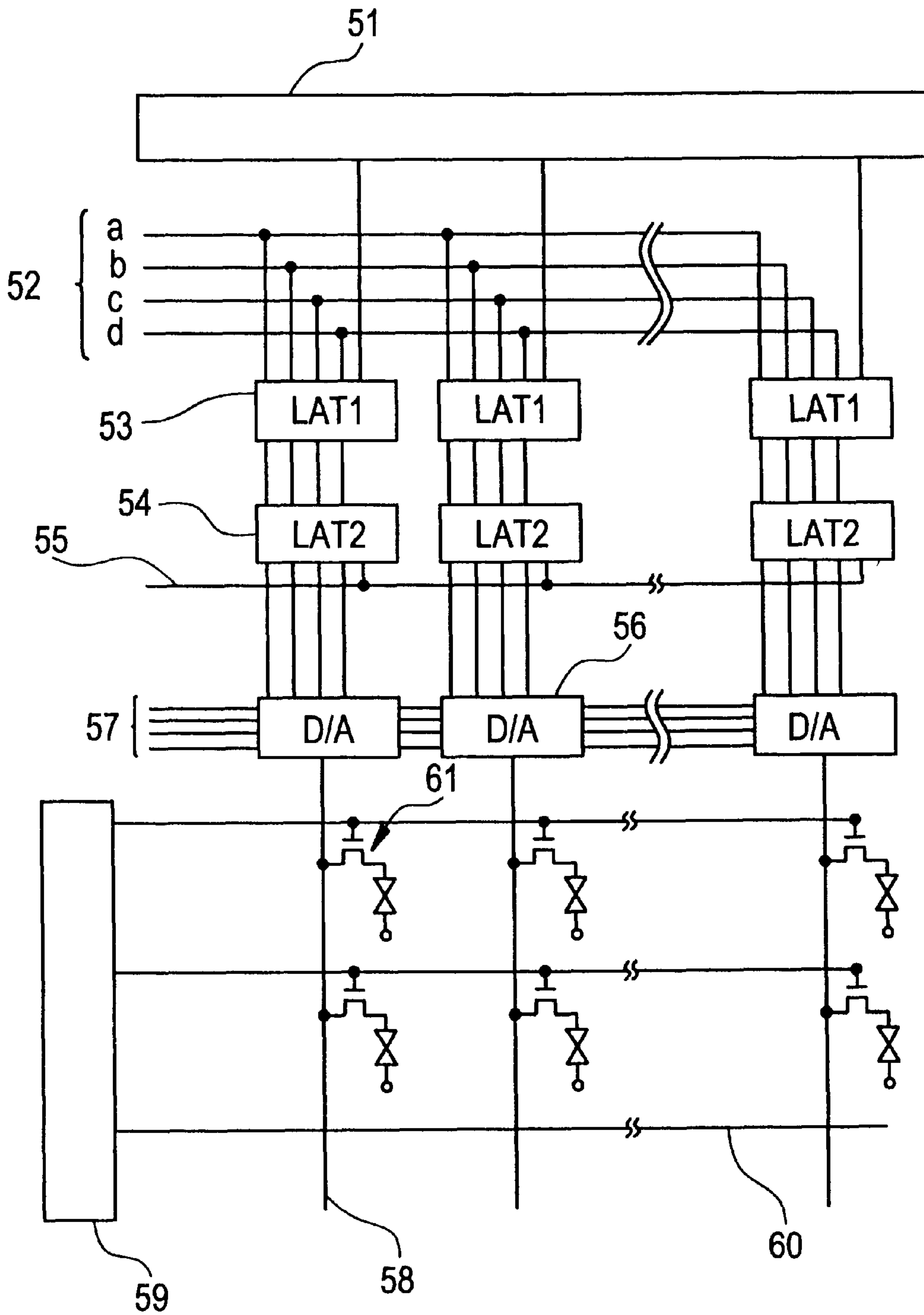
FIG. 34 PRIOR ART
