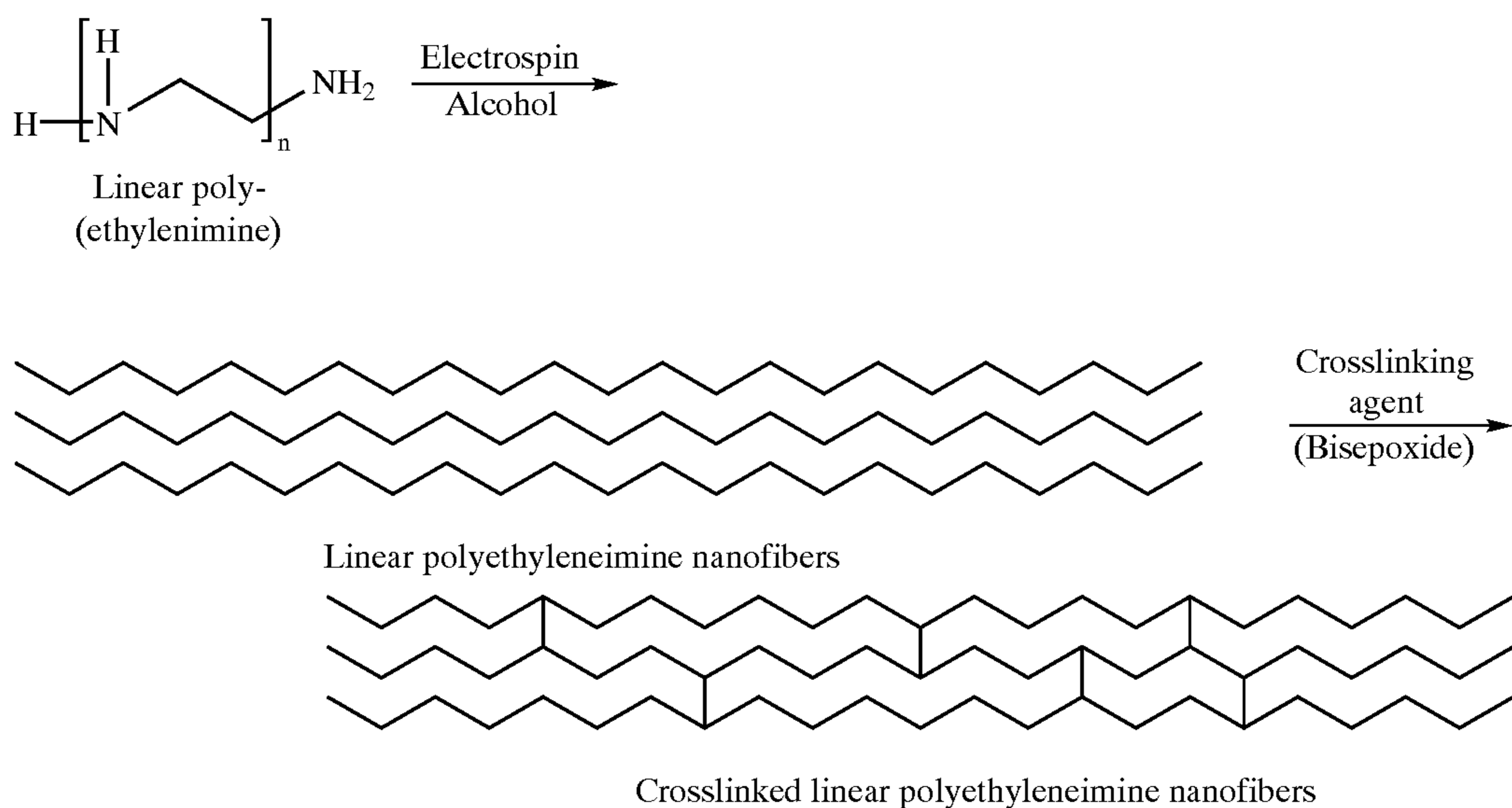
(Scheme III)
