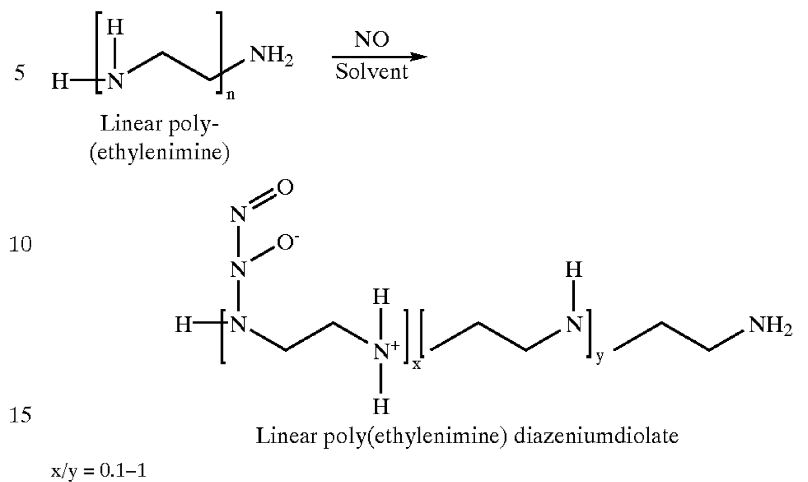
(Scheme I)
