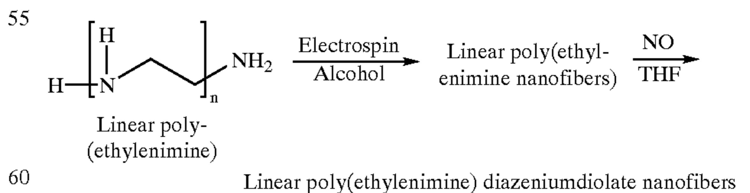
(Scheme II)
