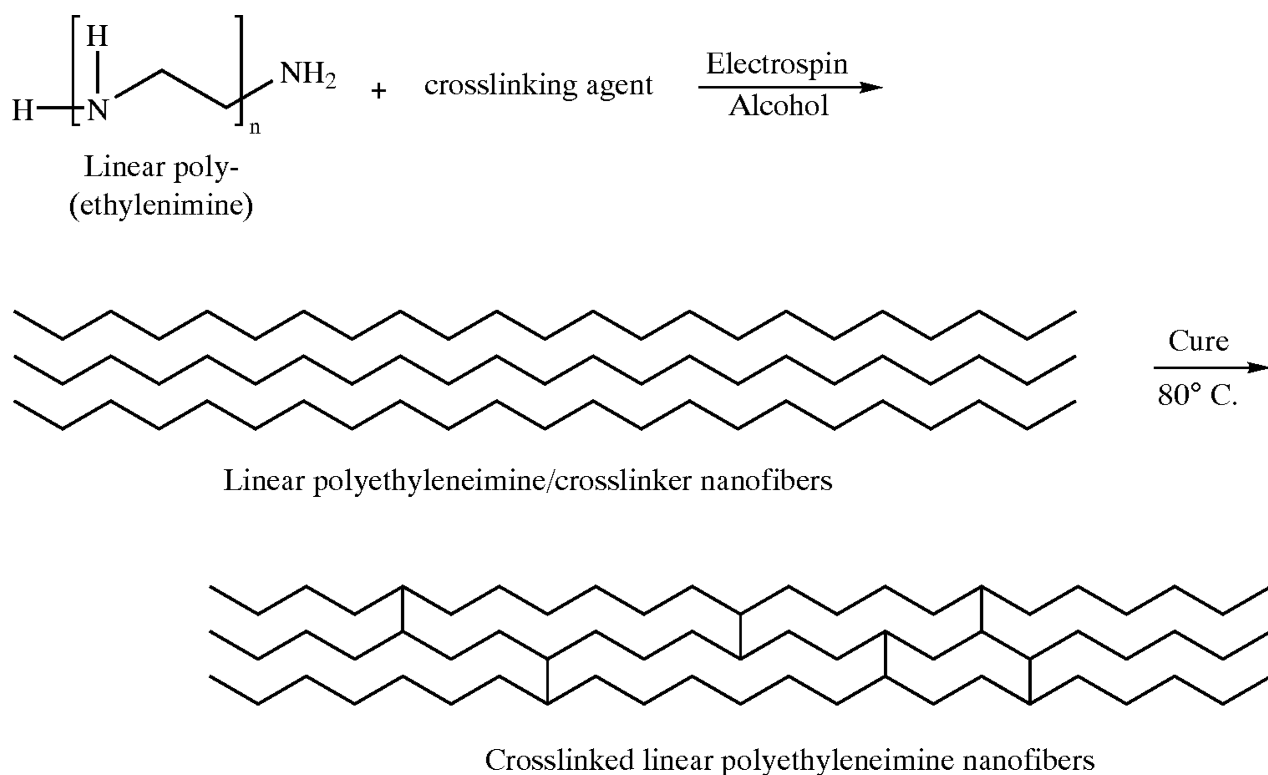
(Scheme IV)
