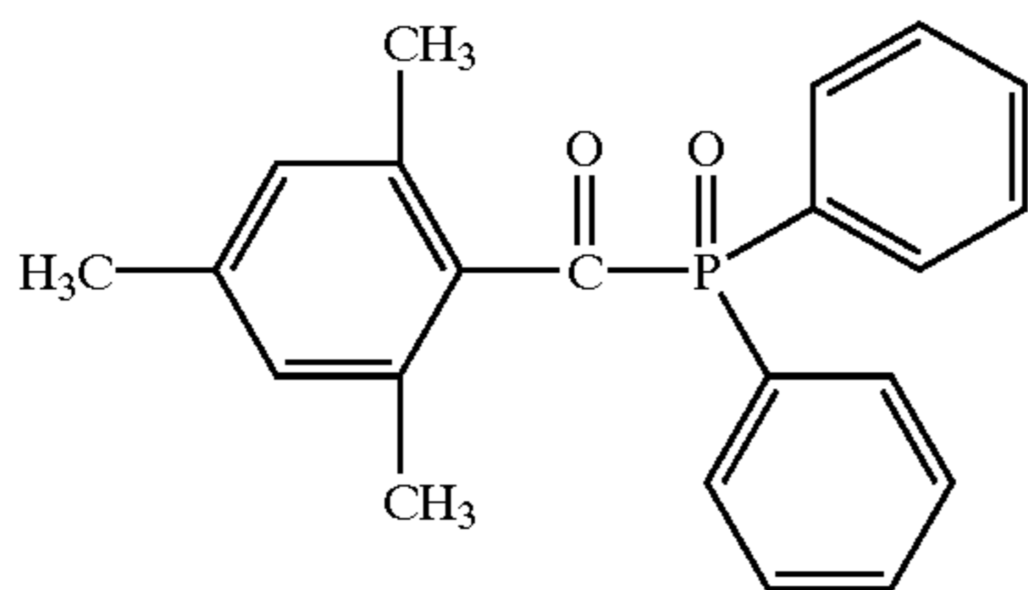
Example 2. Structure of 2,4,6-trimethylbenzoyldiphenylphosphine oxide
