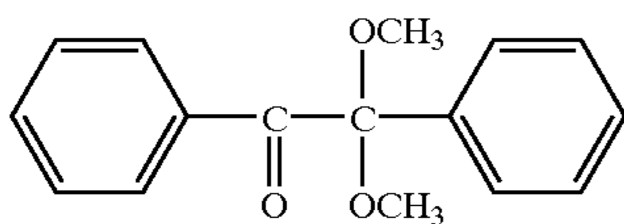
Example 1B: Structure of 2,2-dimethoxy-2-phenylacetophenone (DMPA)
