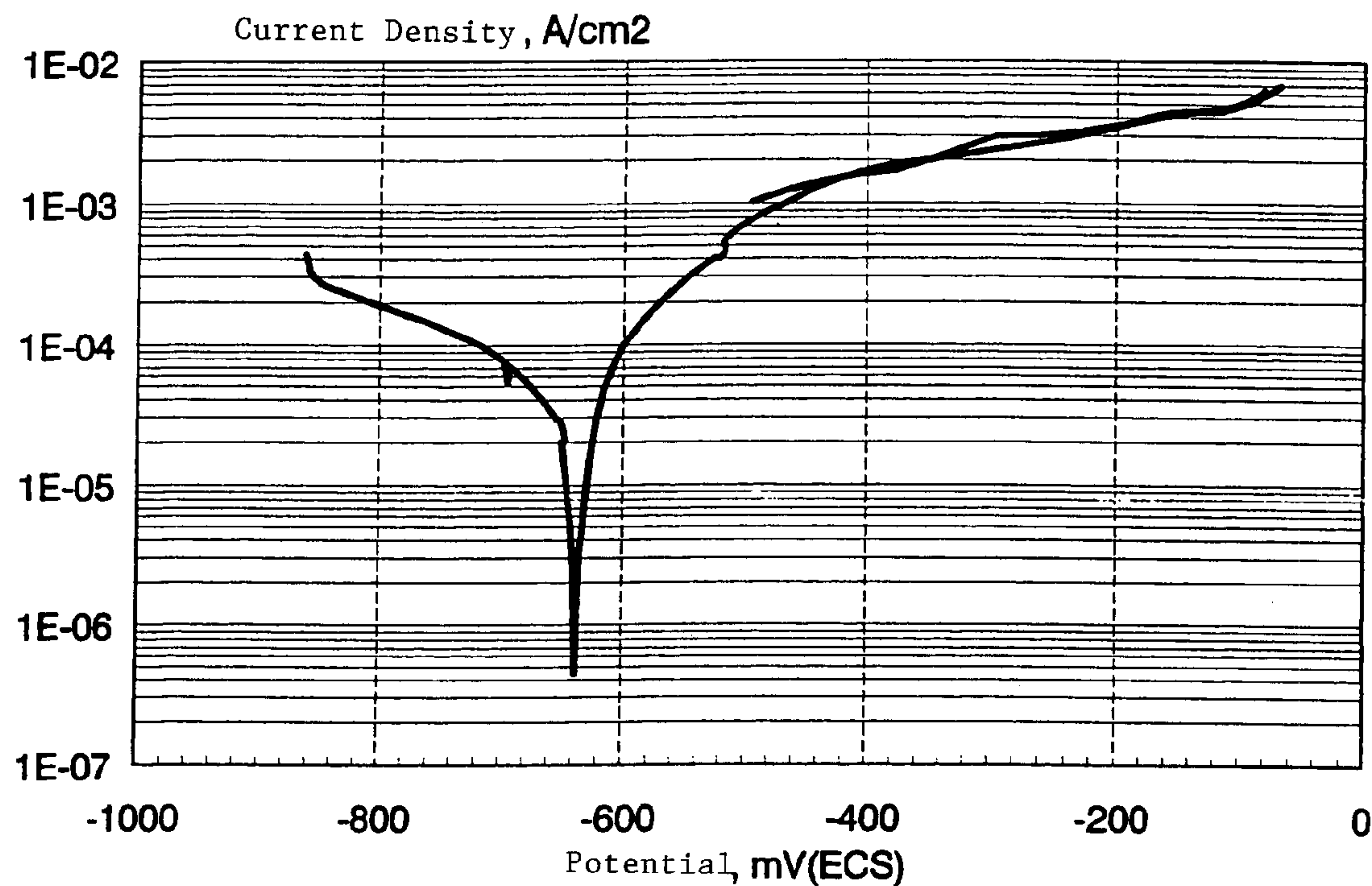
FIGURE 1 - Aluminum Bronze
