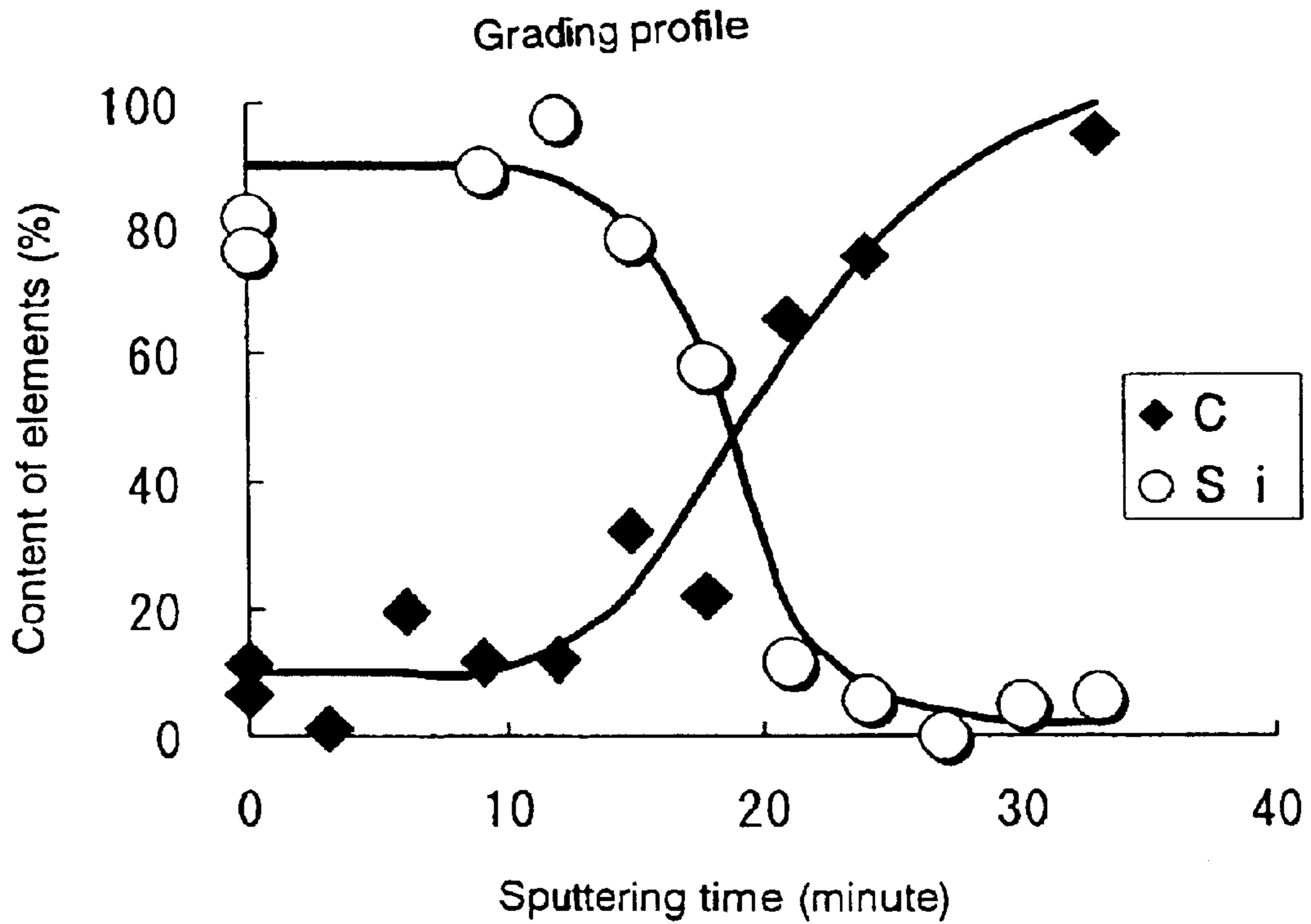
Fig. 26 Grading profile
