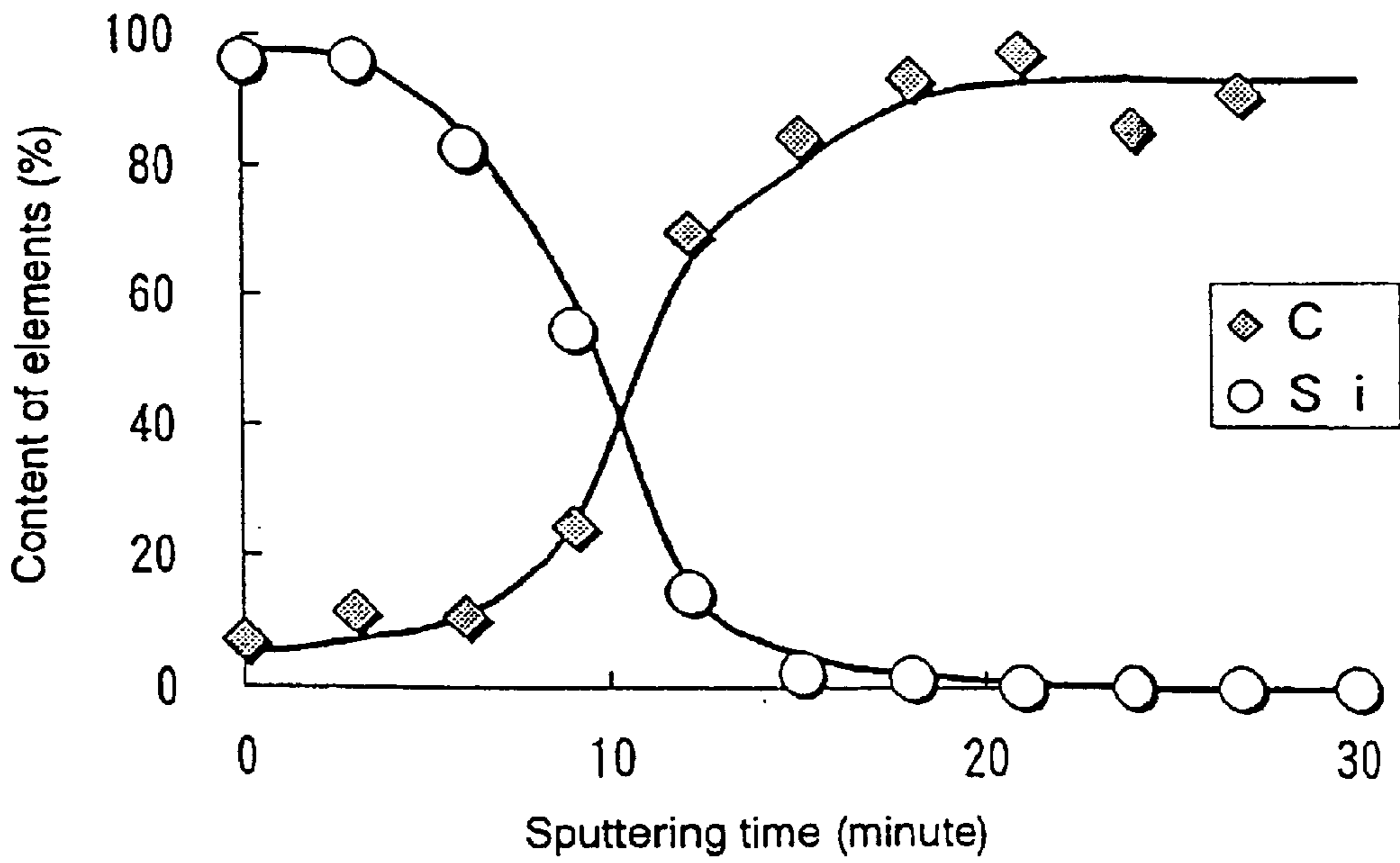
Fig. 29 Grading profile
