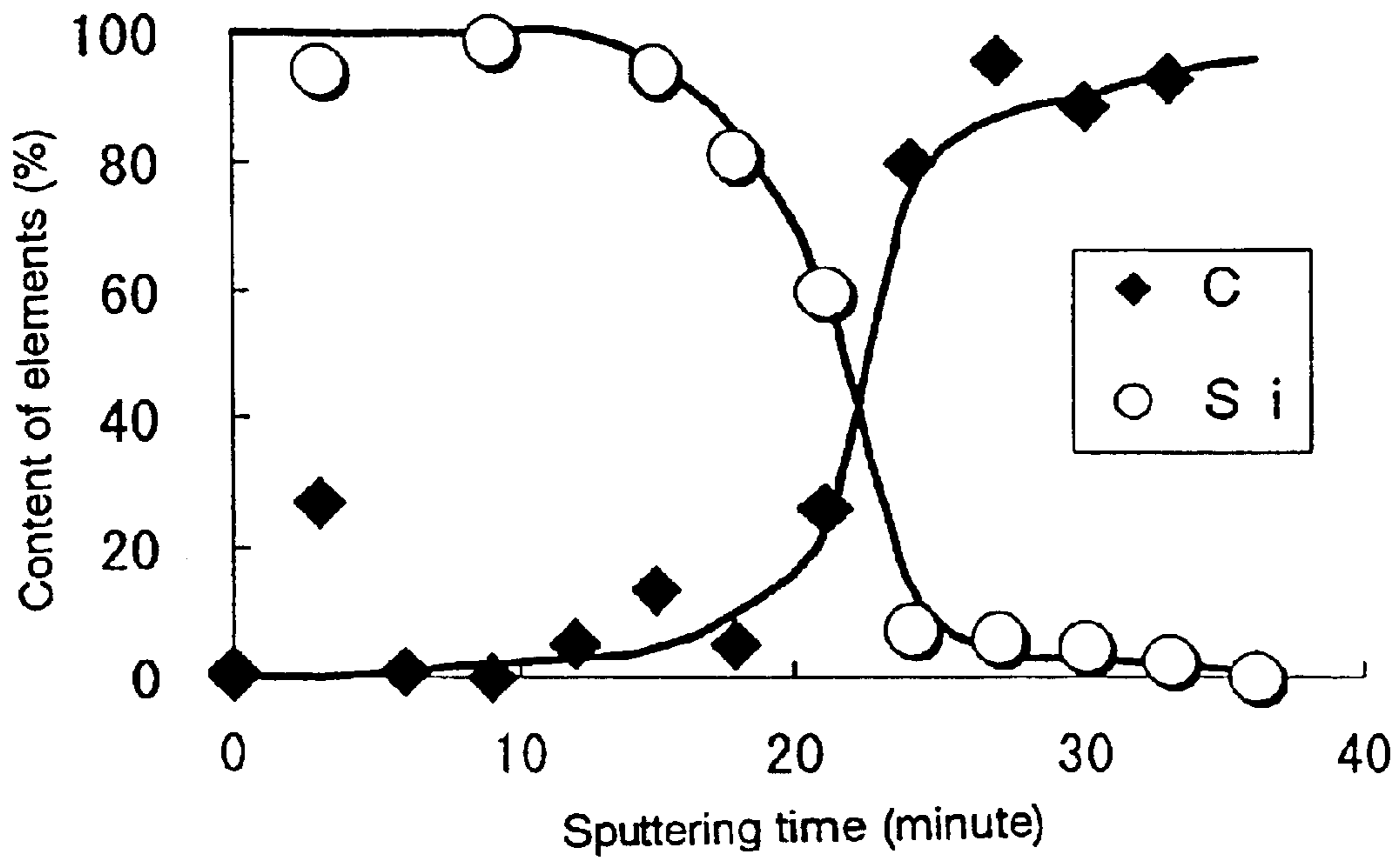
Fig. 25 Grading profile
