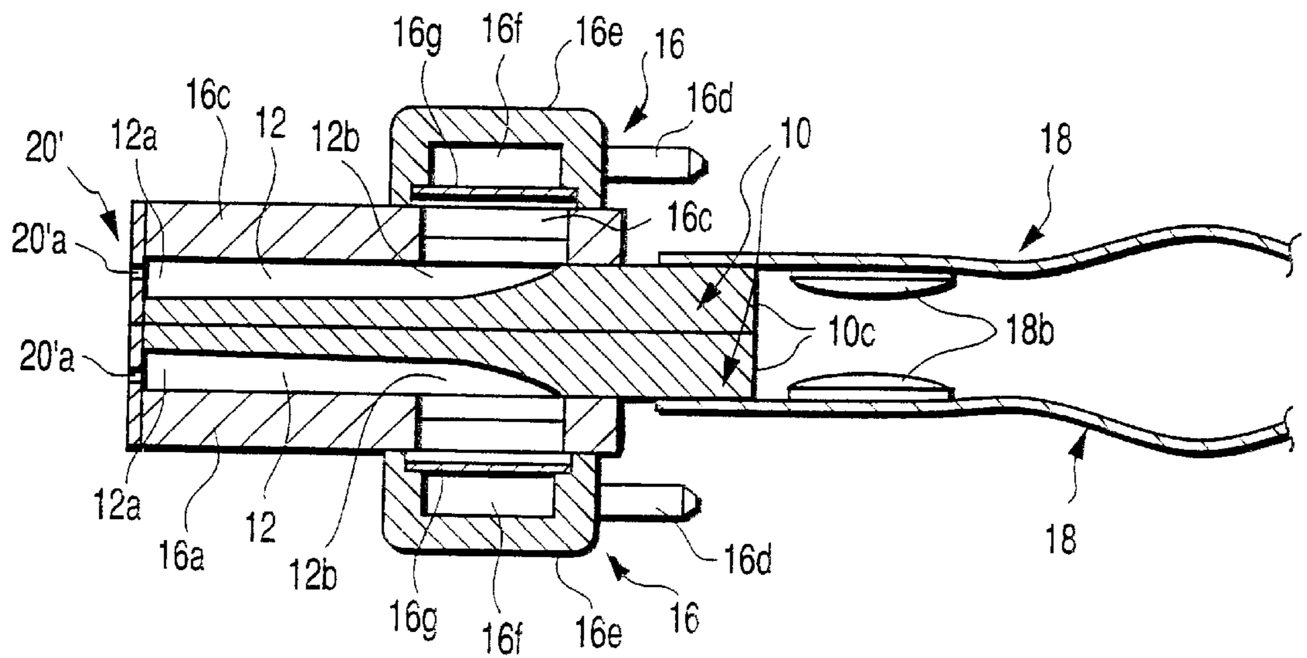
FIG. 4 (PRIOR ART)
