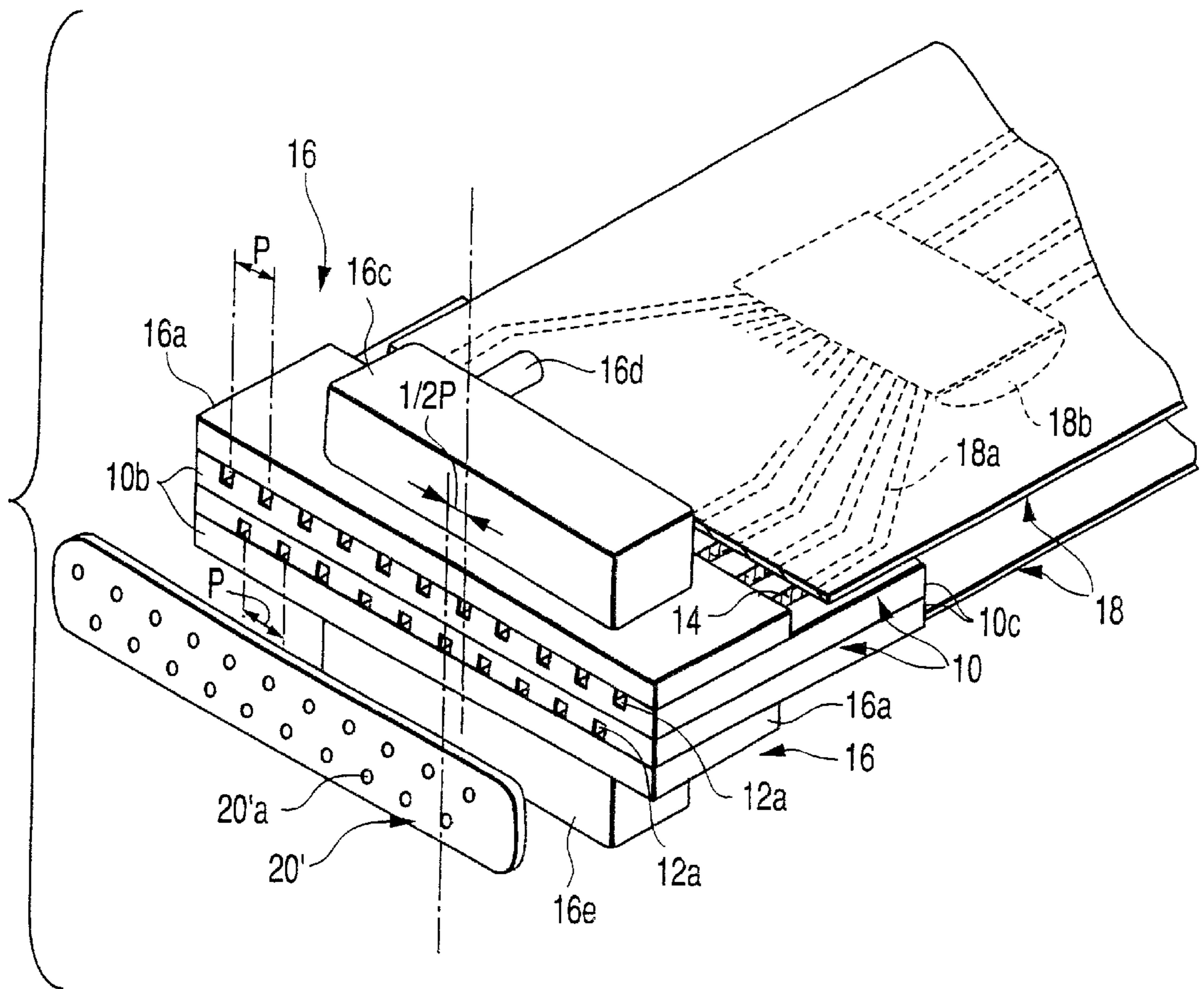
FIG. 3 (PRIOR ART)
