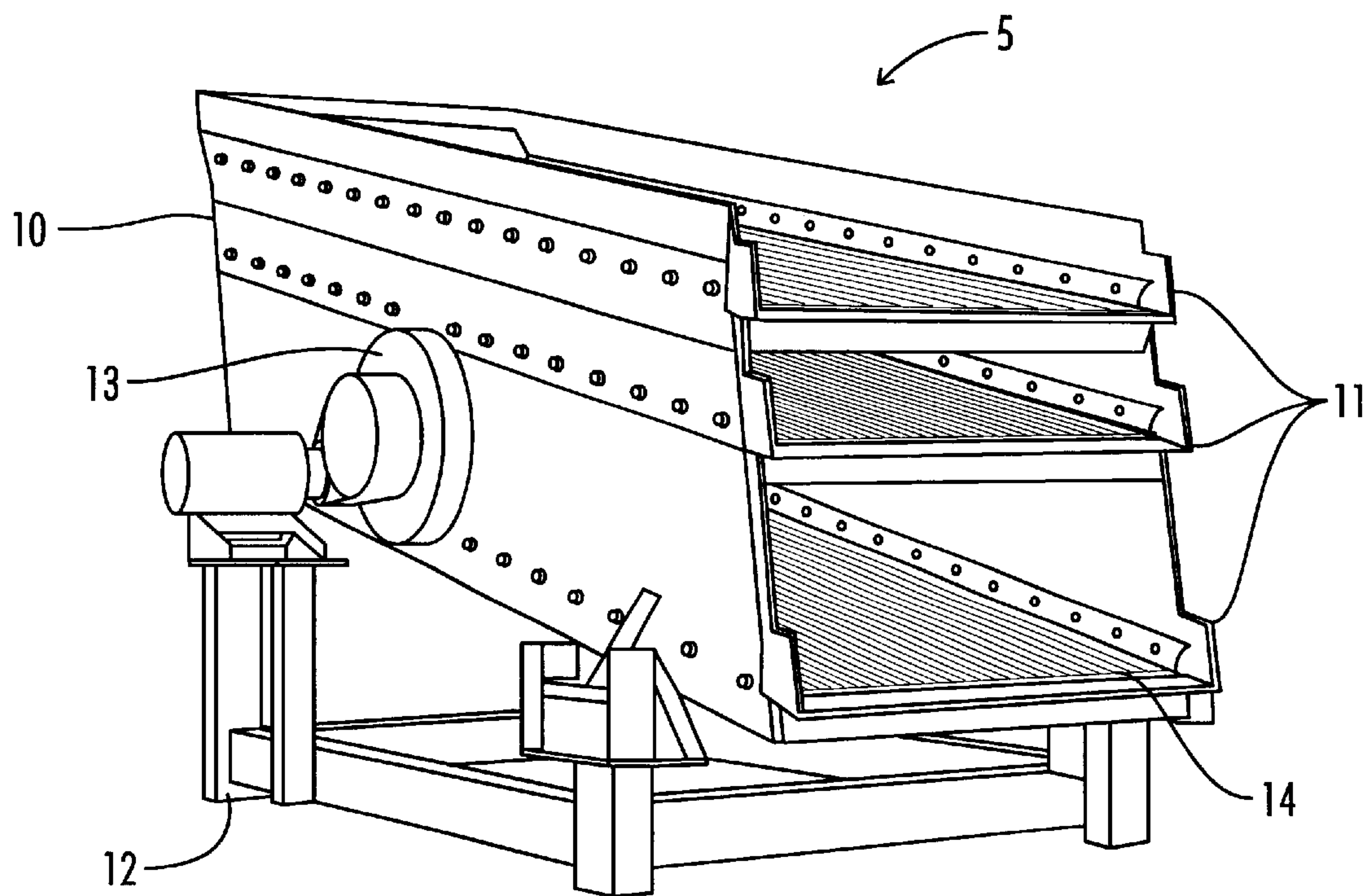
FIG. 1 (Prior Art)
