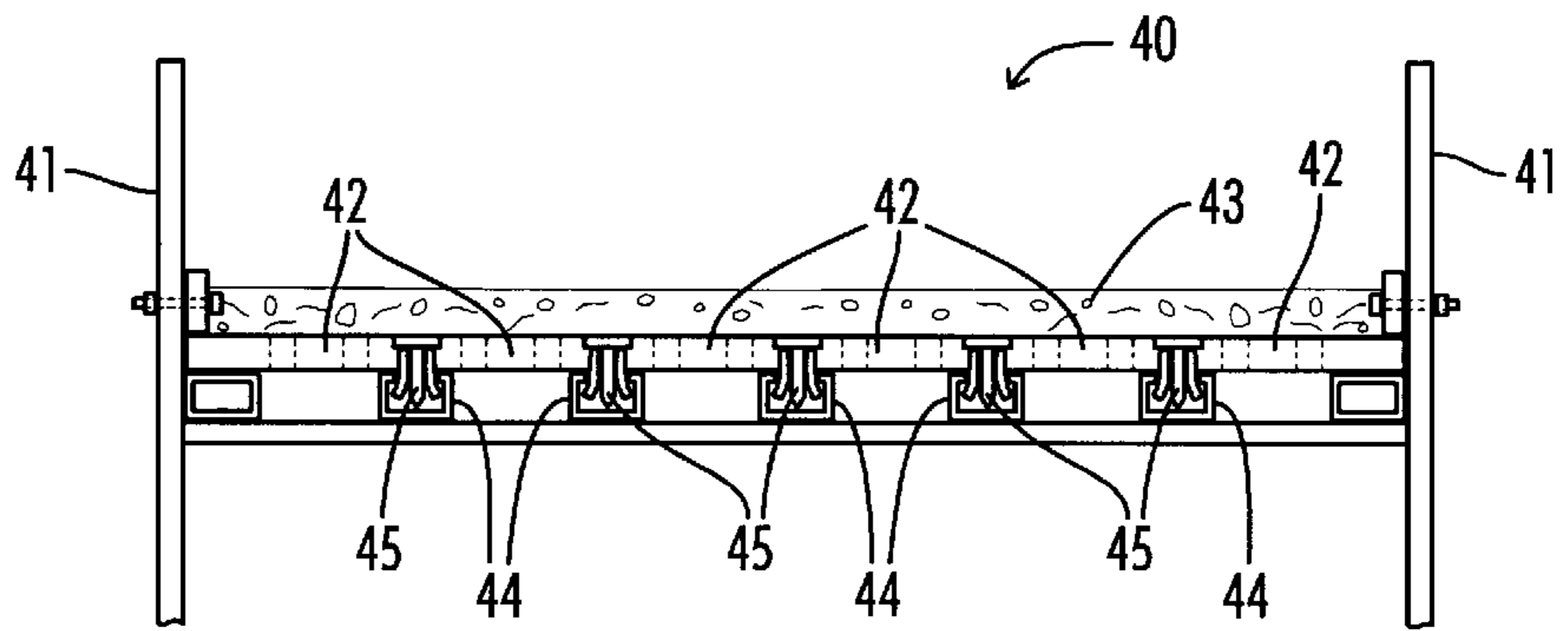
FIG. 4 (Prior Art)
