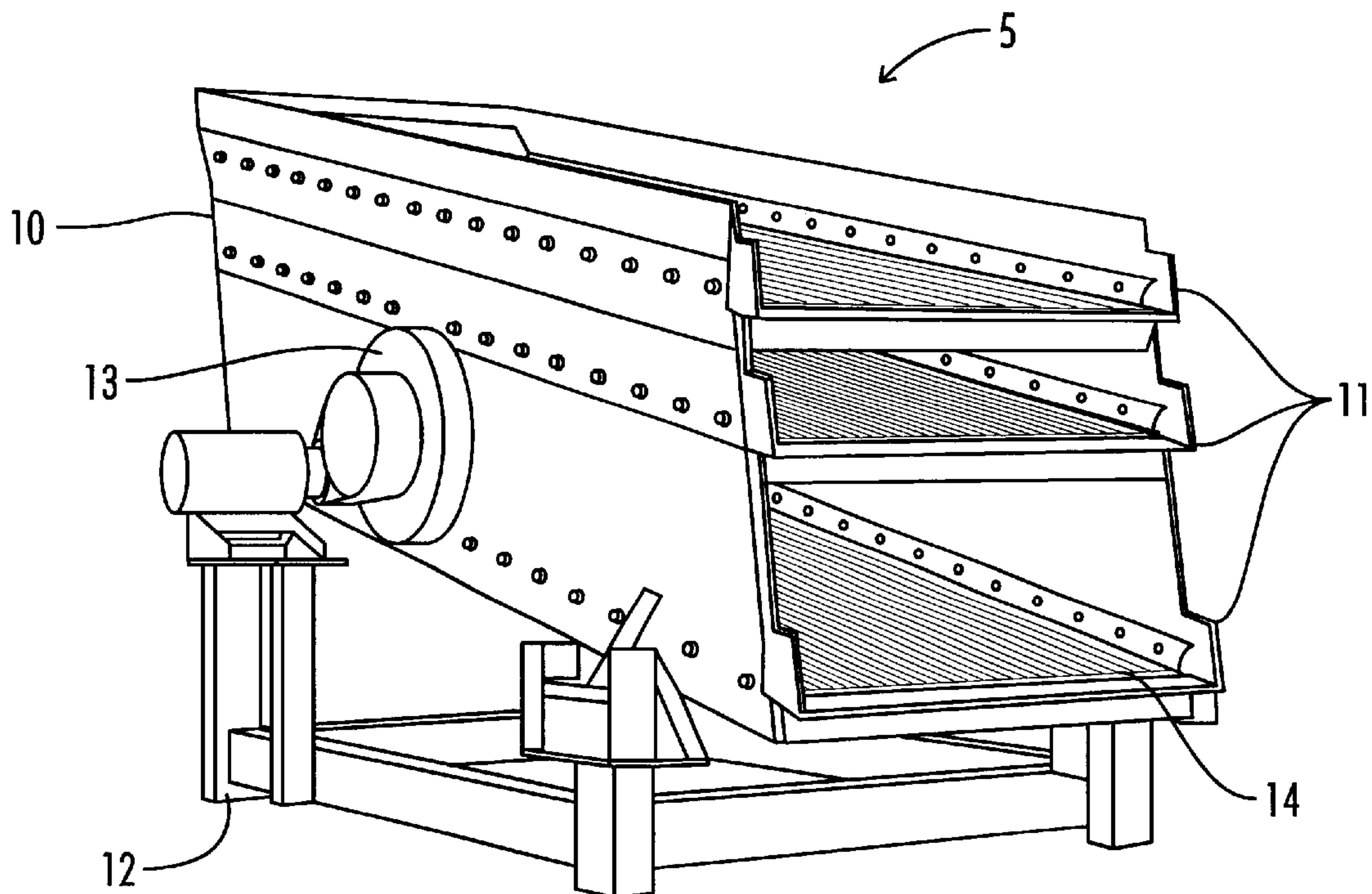
FIG. 1 (Prior Art)
