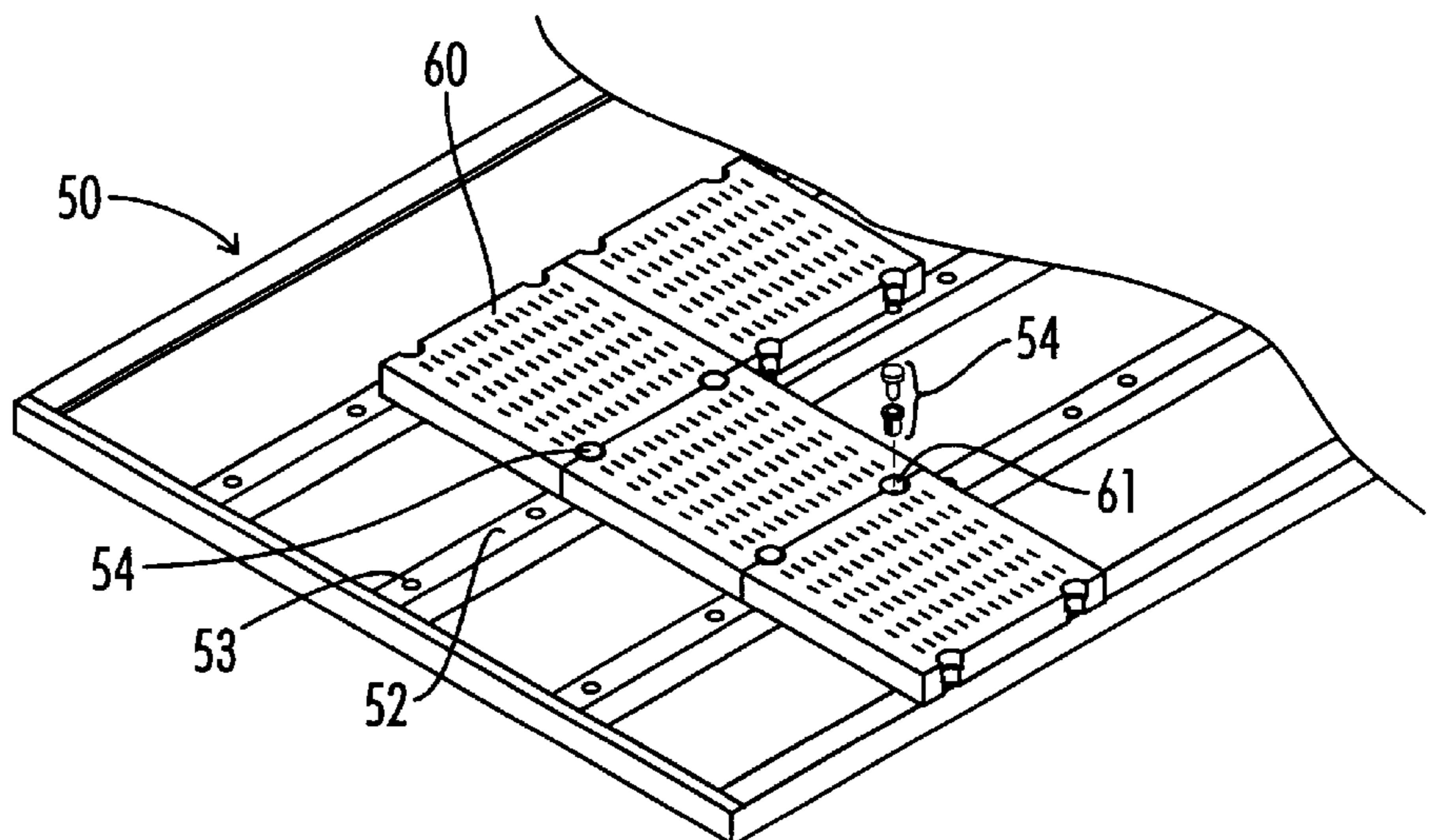
FIG. 7 (Prior Art)
