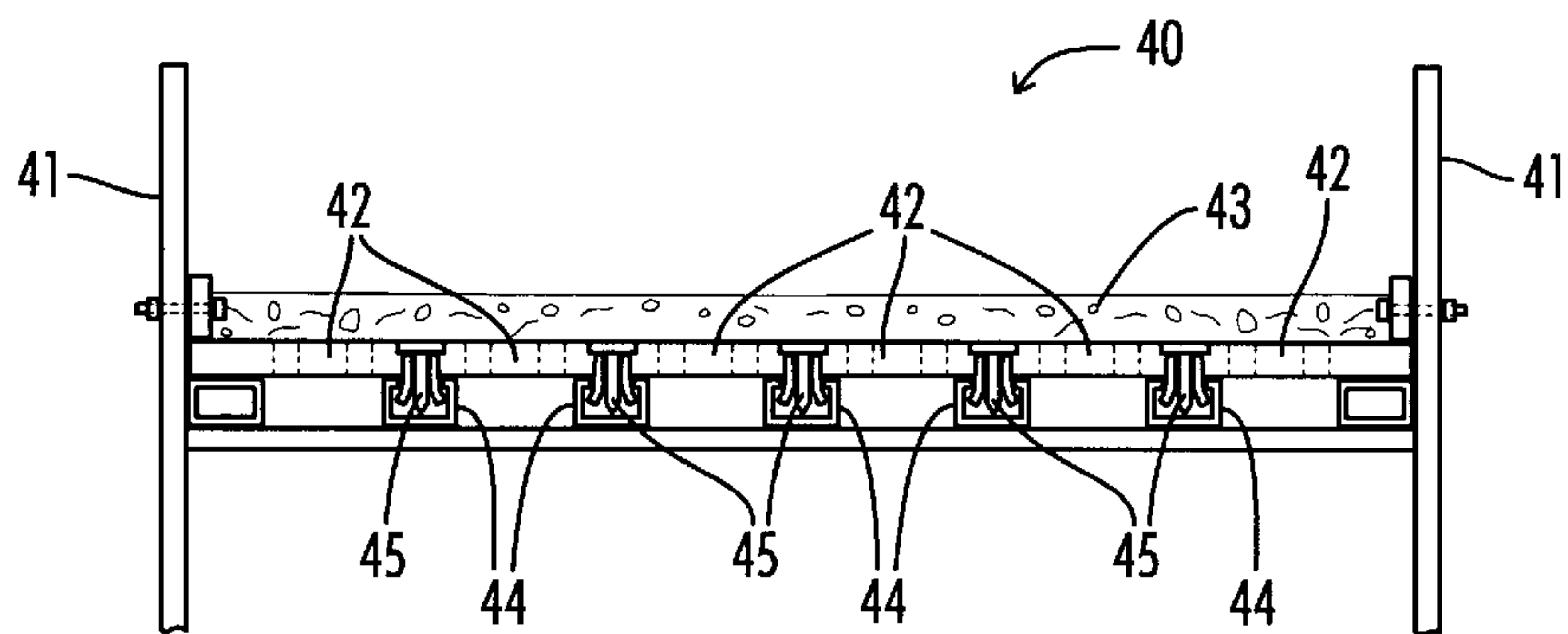
FIG. 4 (Prior Art)
