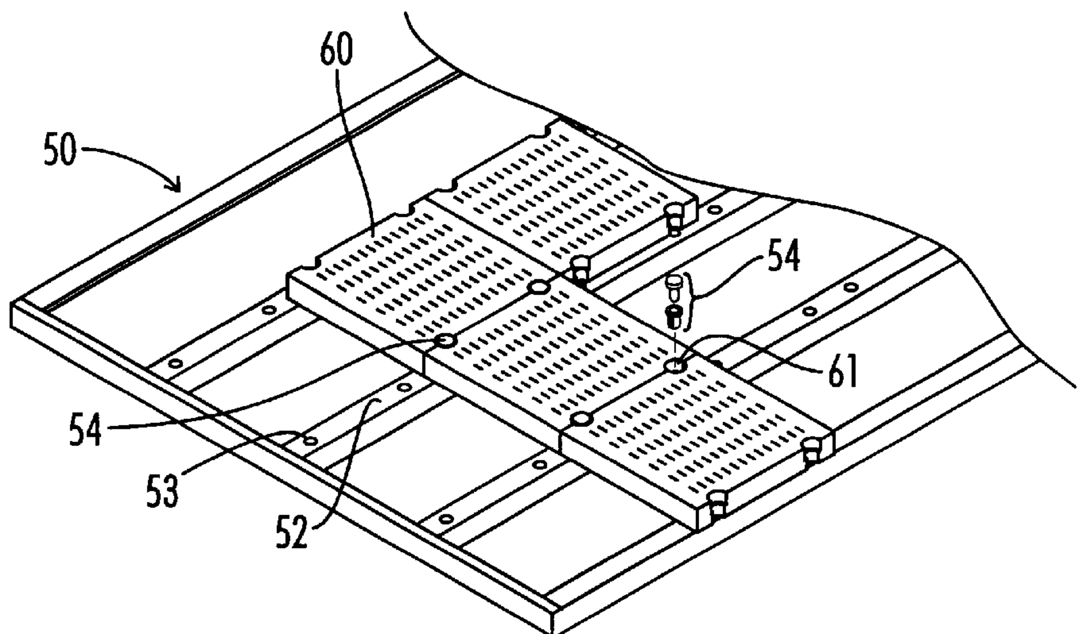
FIG. 7 (Prior Art)
