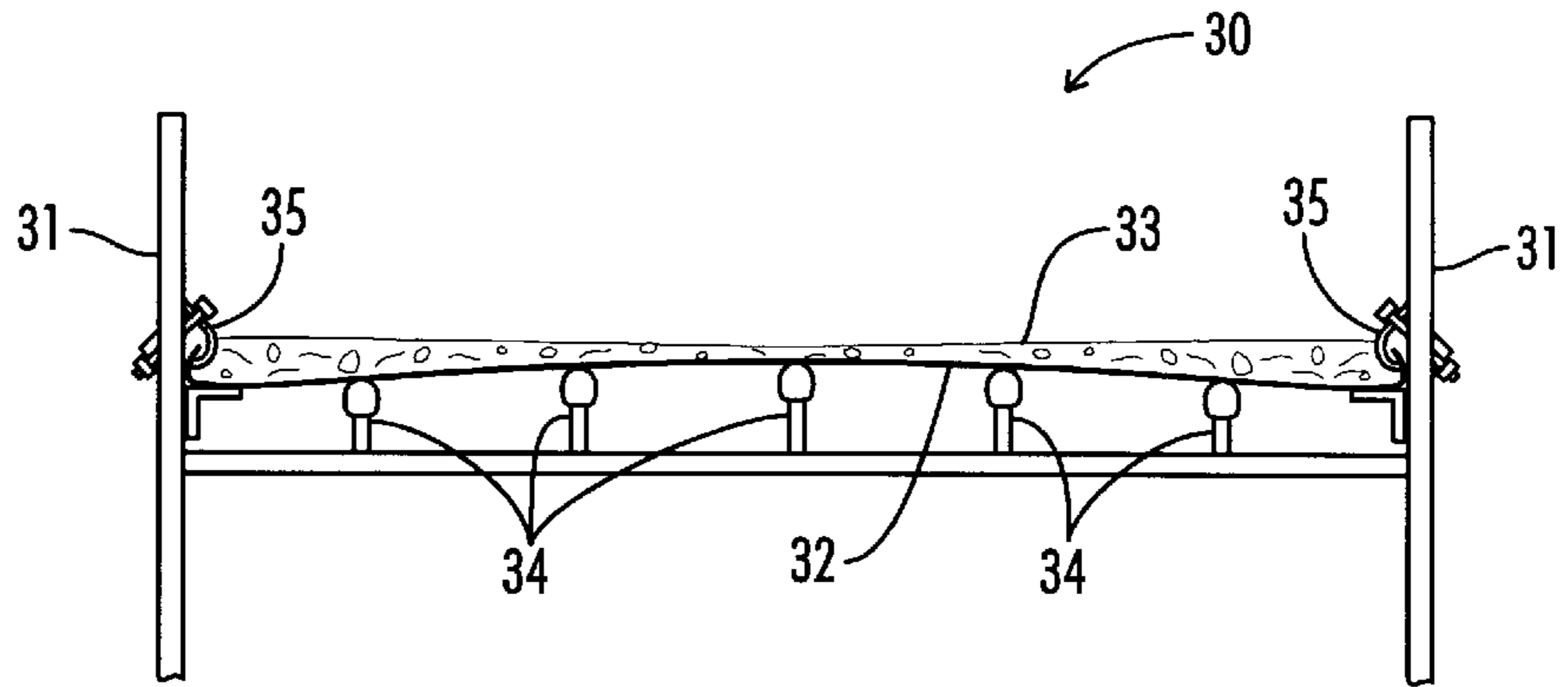
FIG. 3 (Prior Art)
