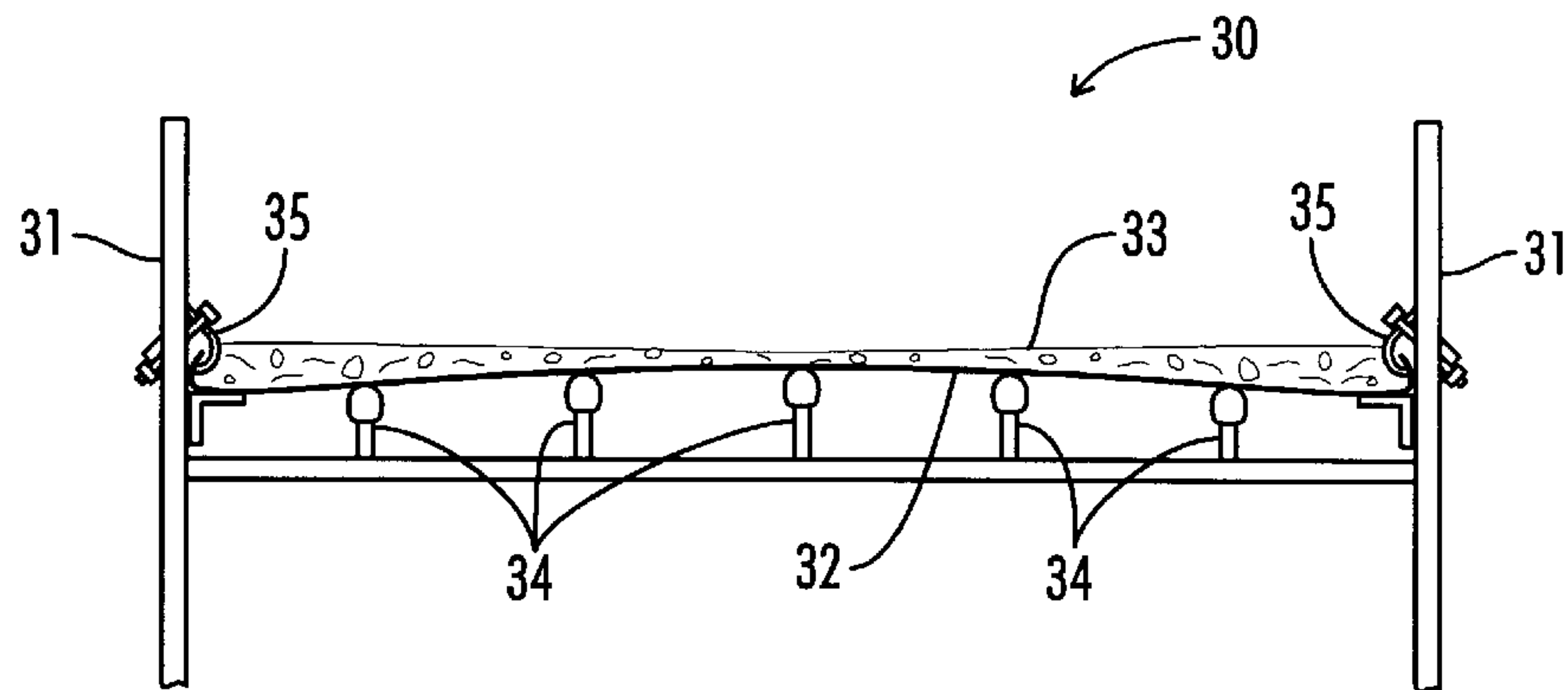
FIG. 3 (Prior Art)
