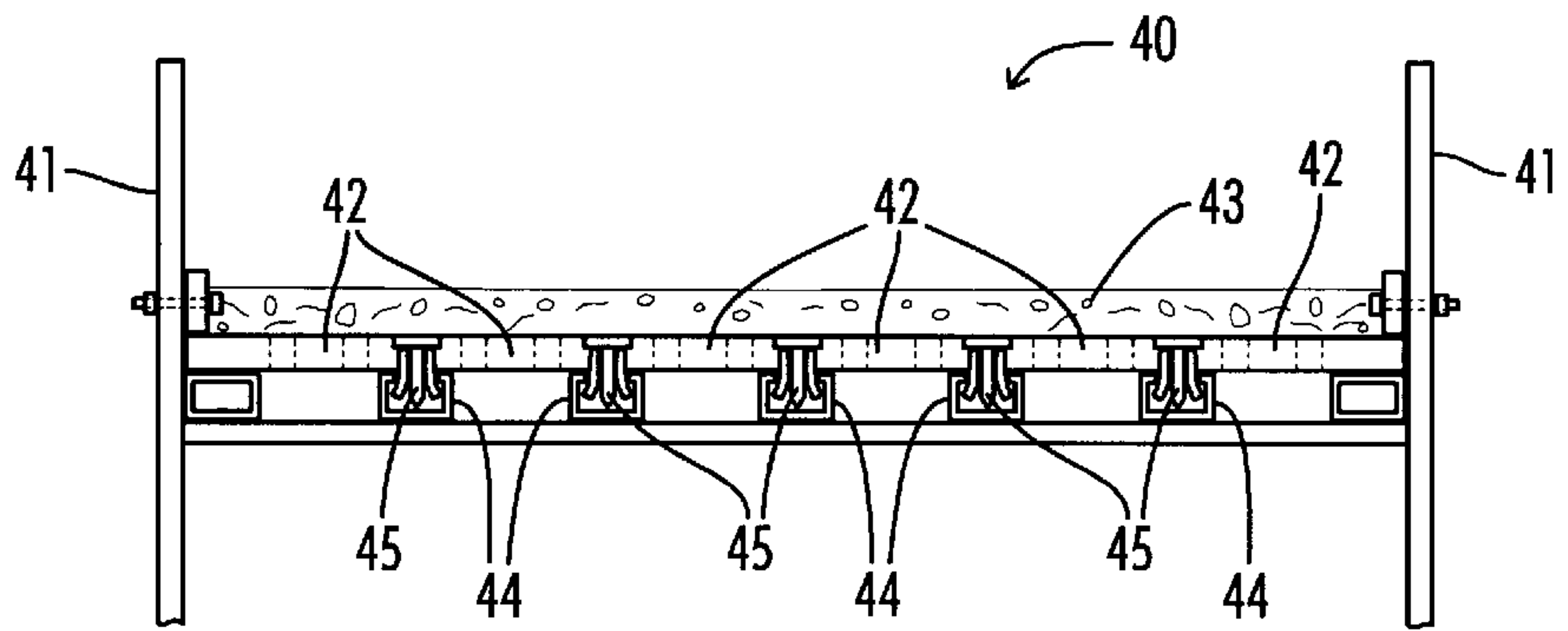
FIG. 4 (Prior Art)
