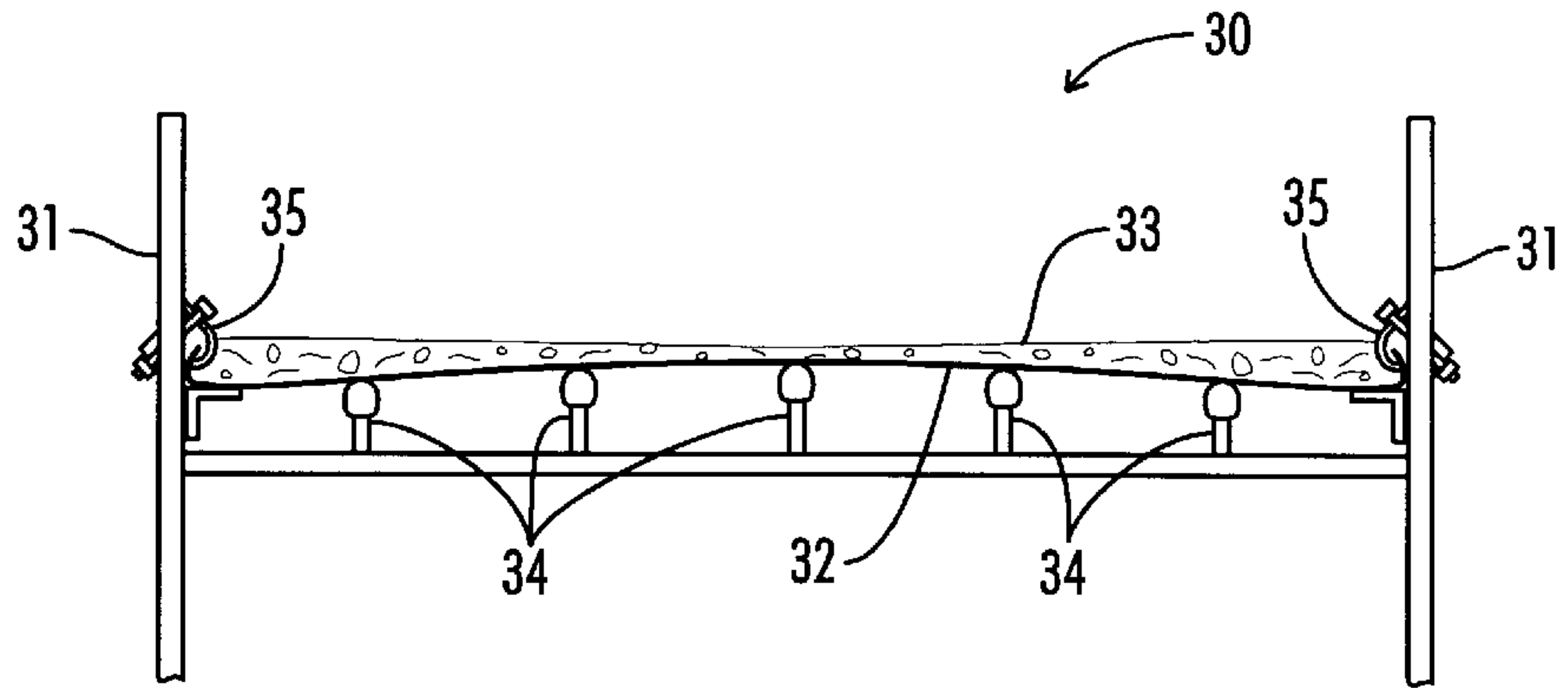
FIG. 3 (Prior Art)
