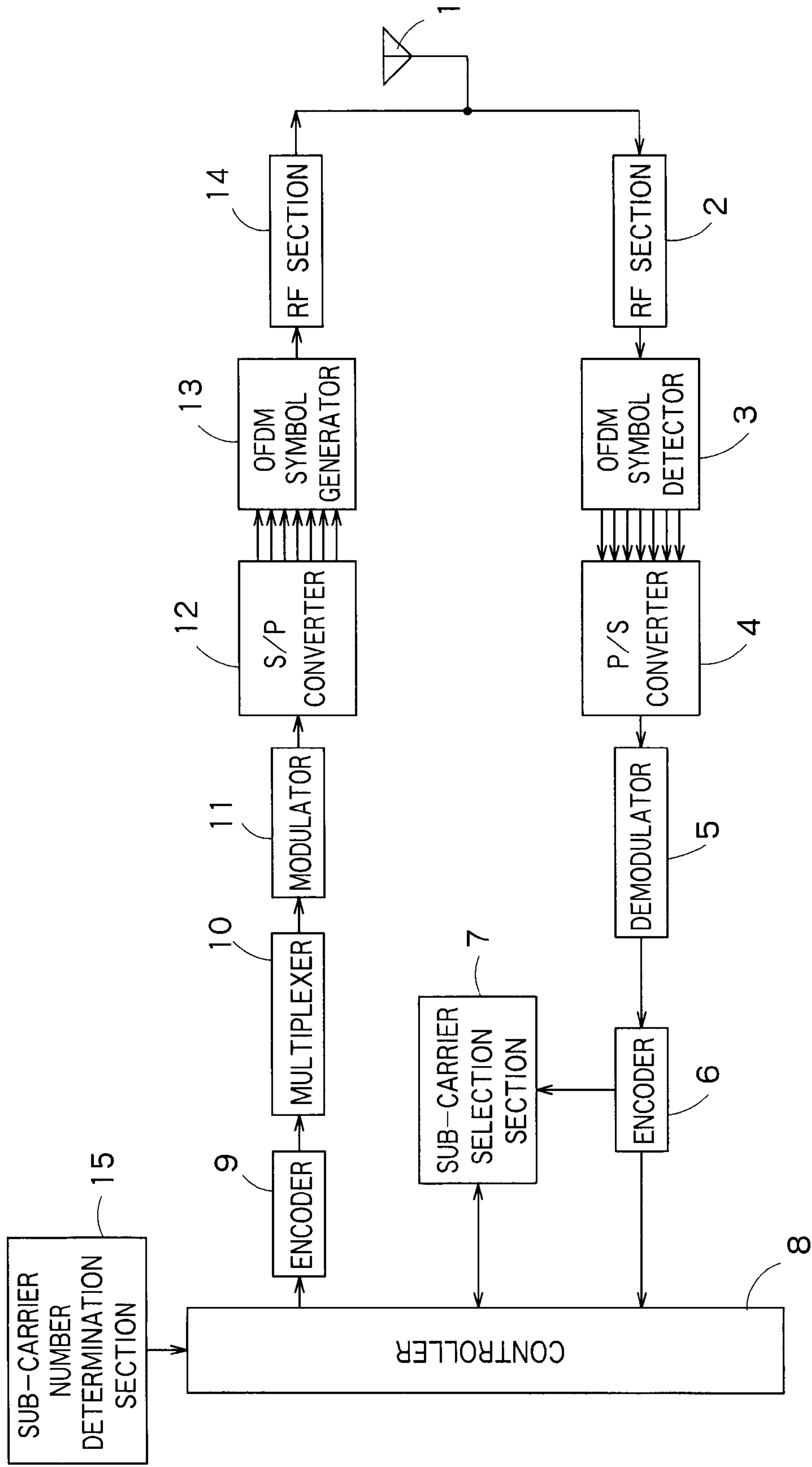
TERMINAL STATION CONSTITUTION
