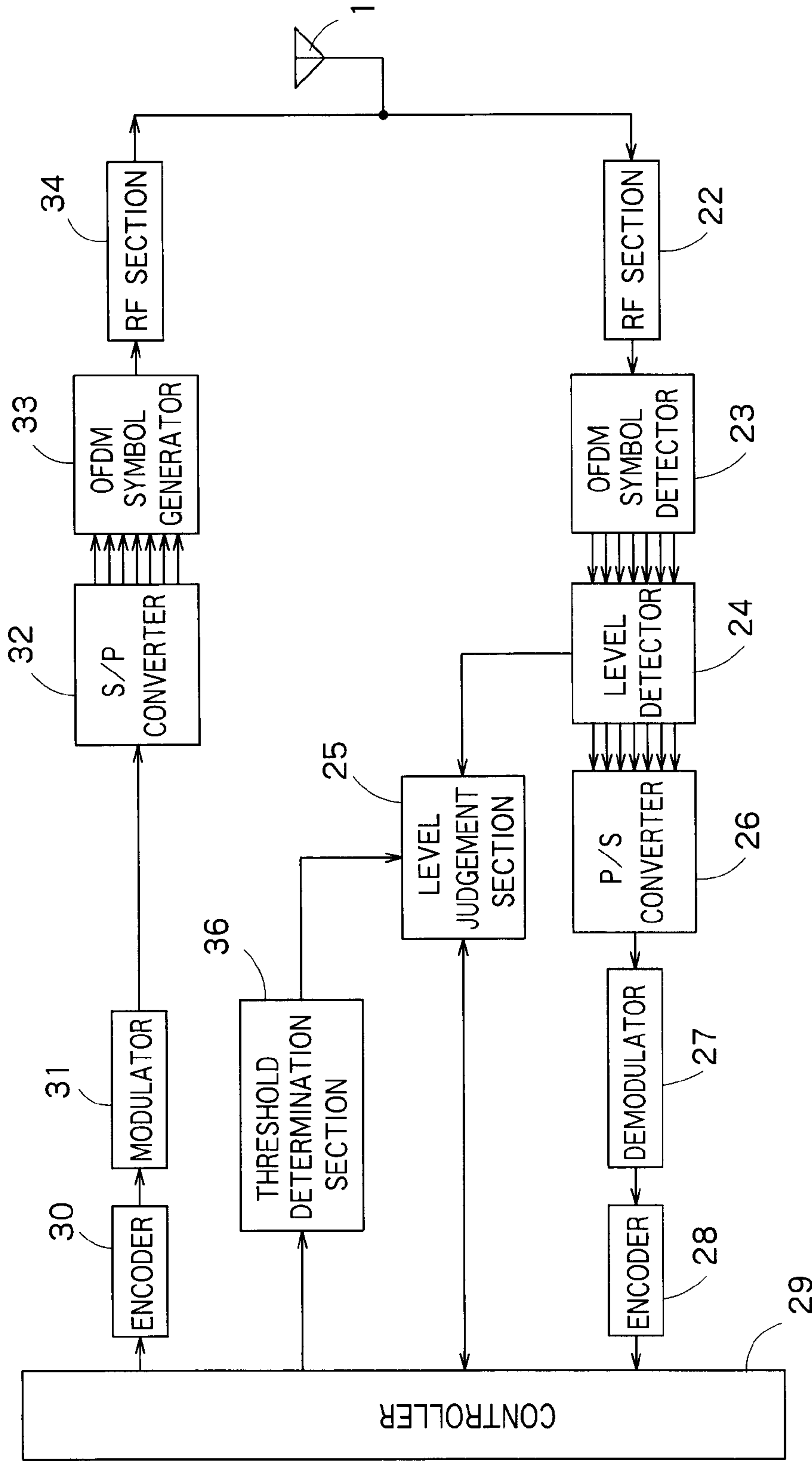
BASE STATION CONSTITUTION
