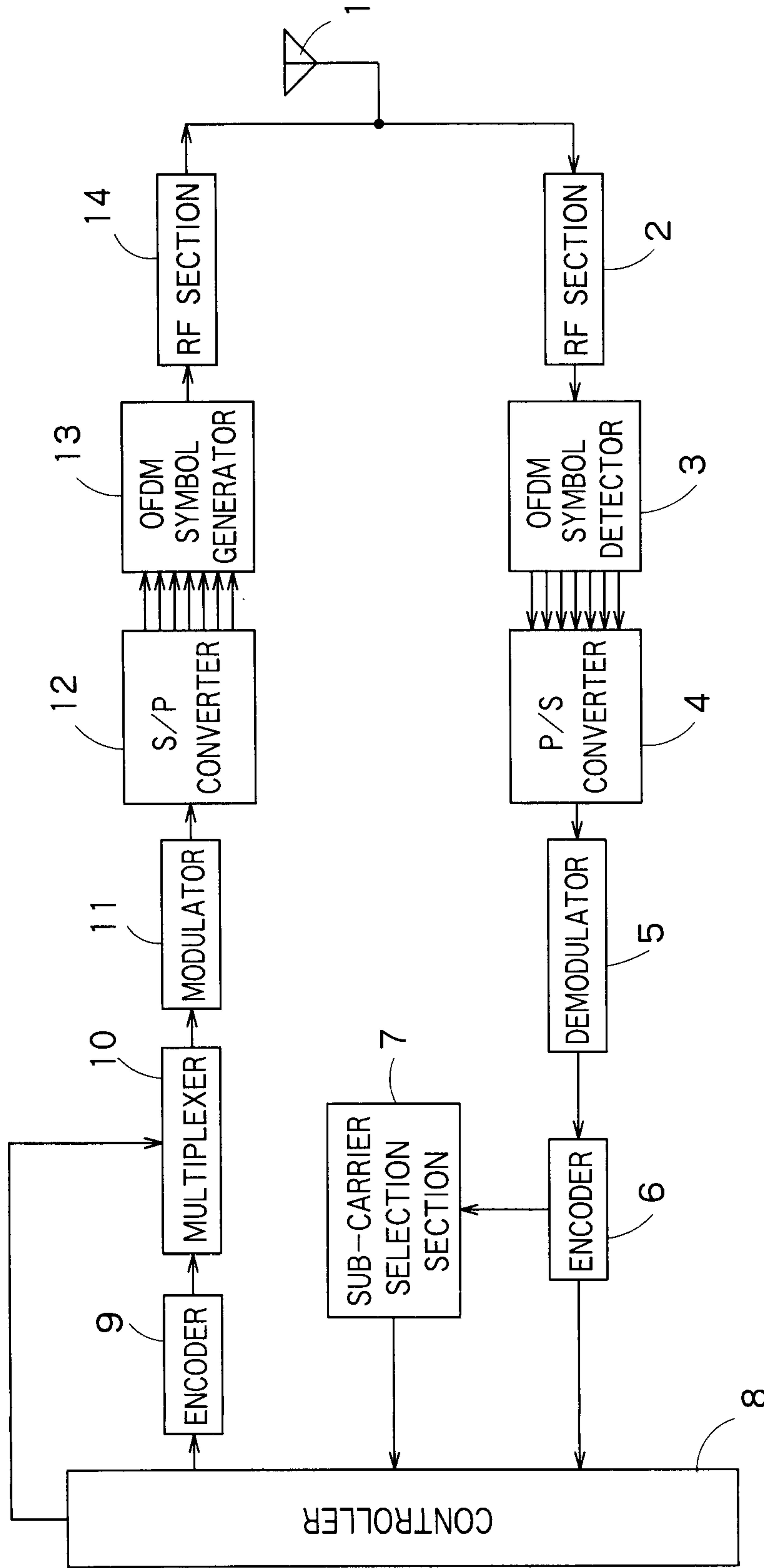
TERMINAL STATION CONSTITUTION
