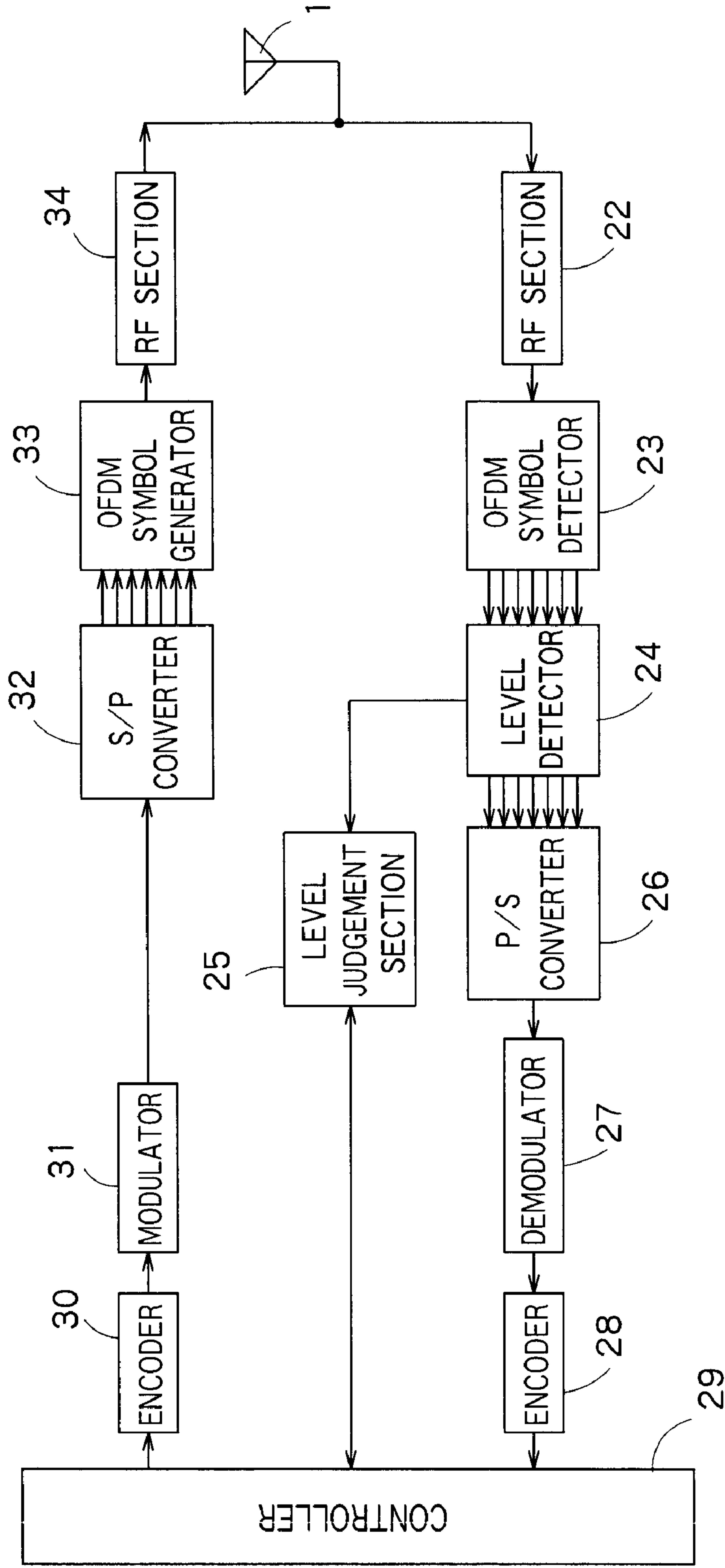
BASE STATION CONSTITUTION
