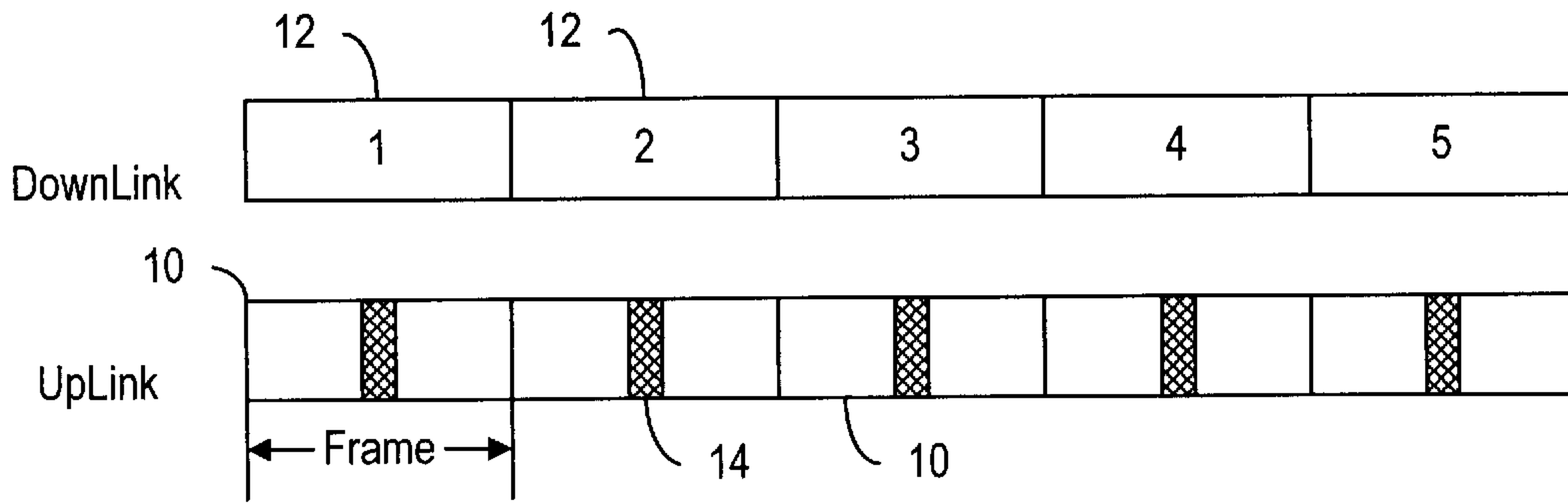
Figure 1 UpLink and DownLink Frames
