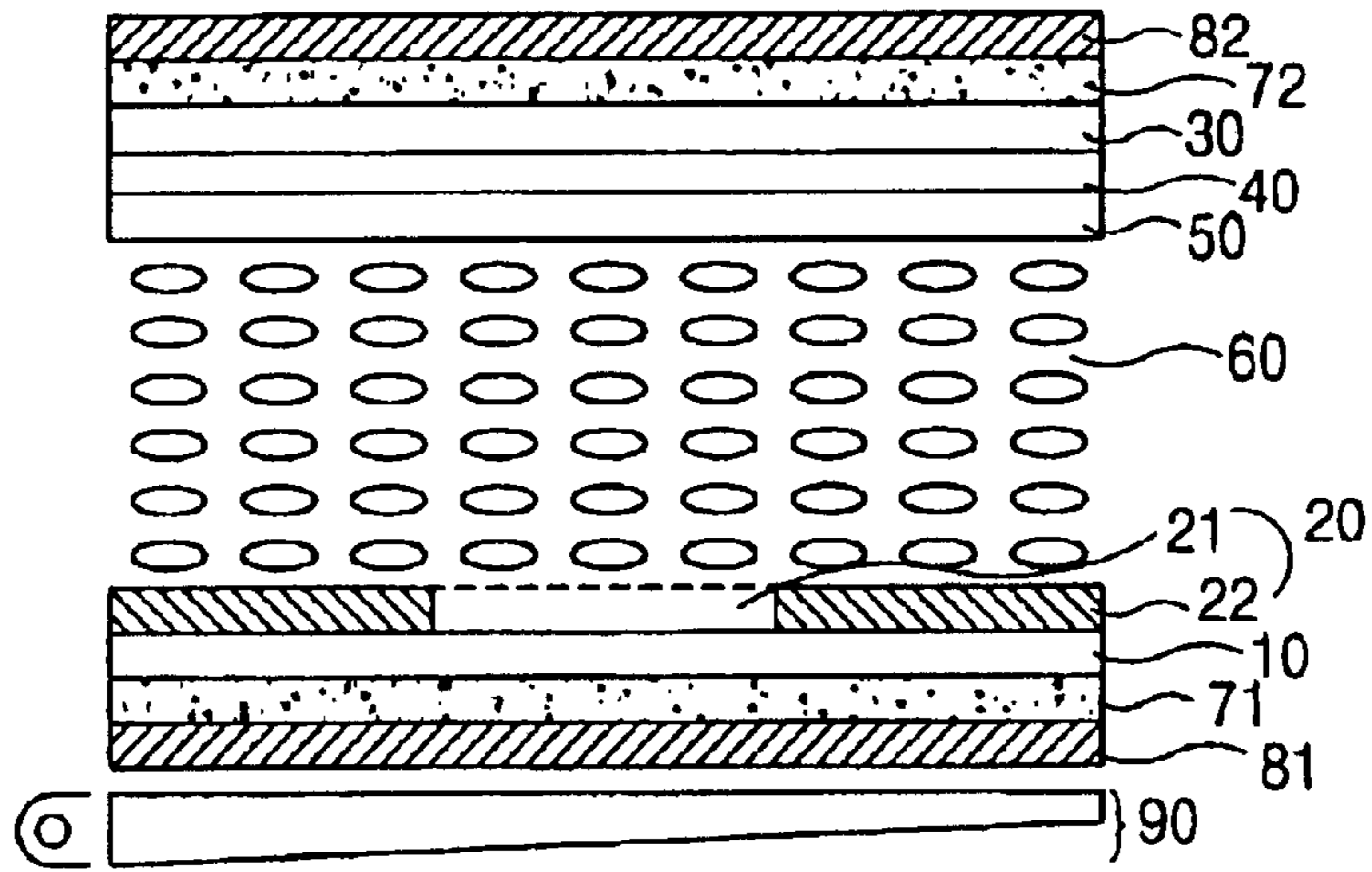
FIG. 1 (PRIOR ART)
