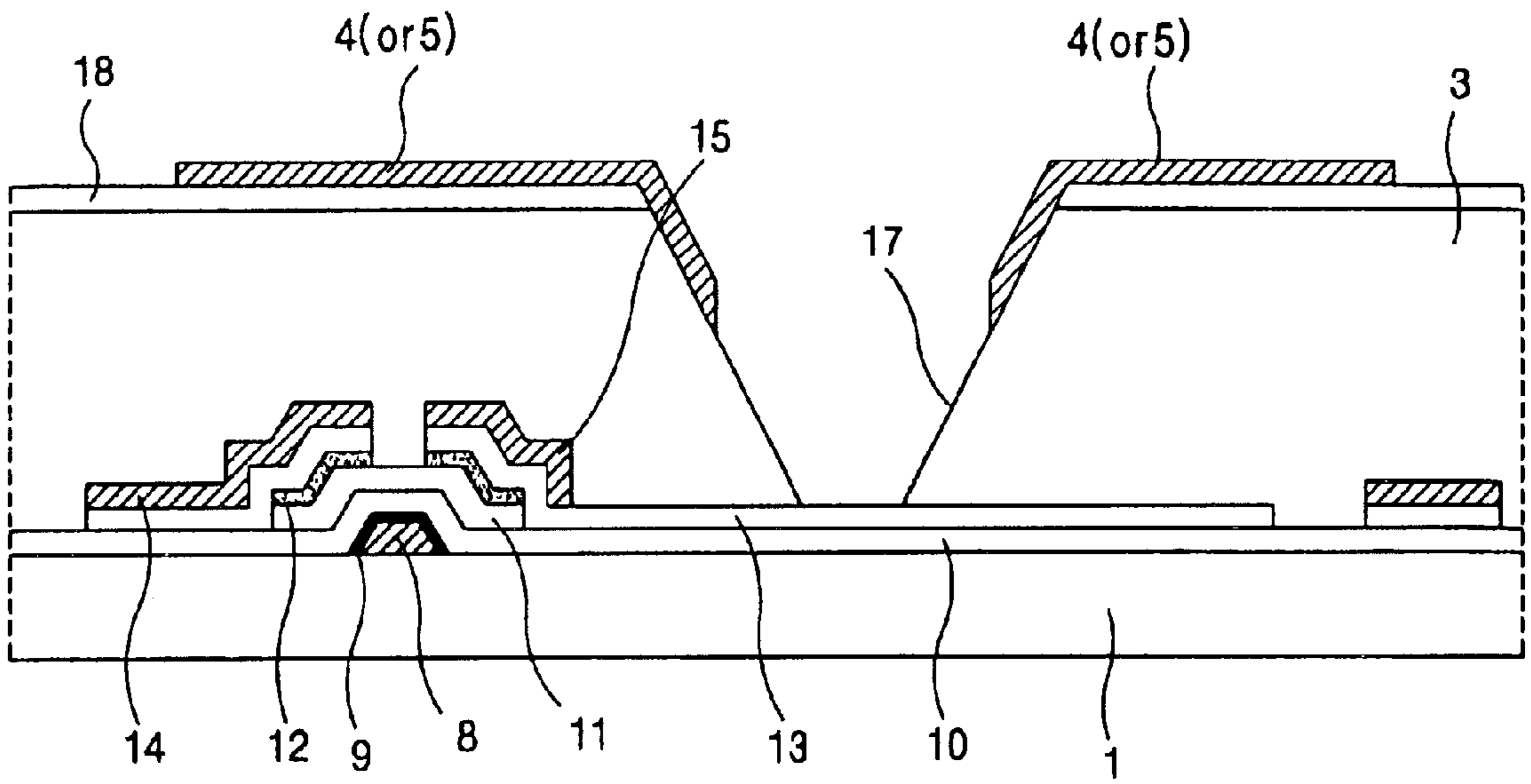
FIG. 5 (PRIOR ART)
