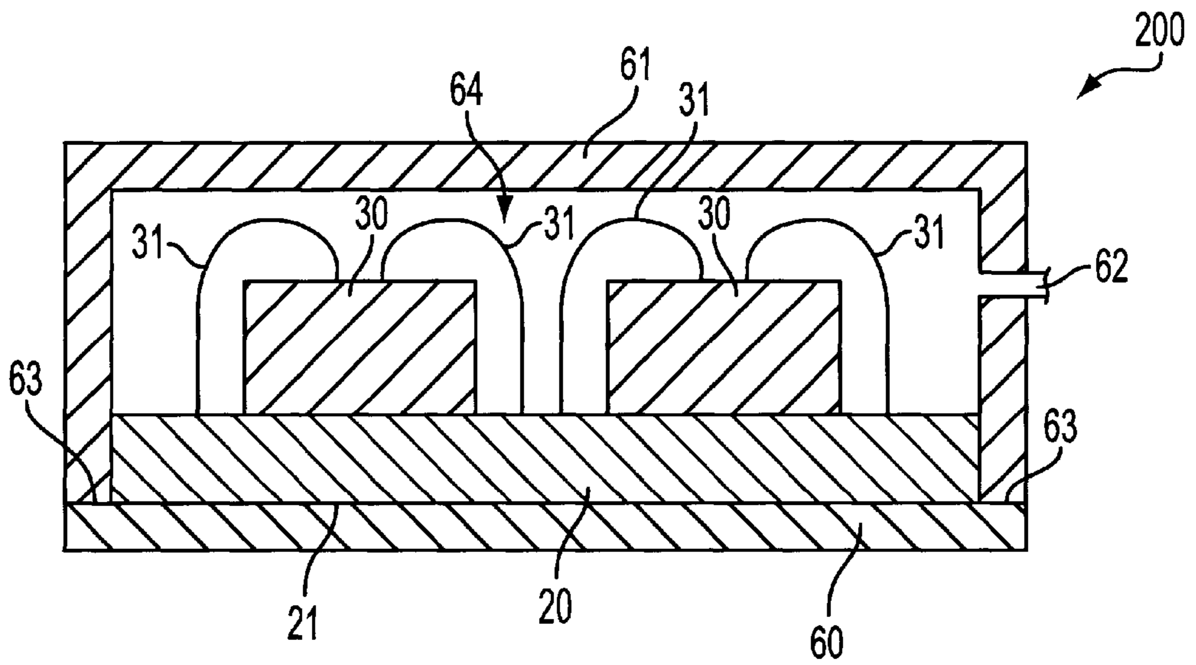
FIG. 3 (PRIOR ART)
