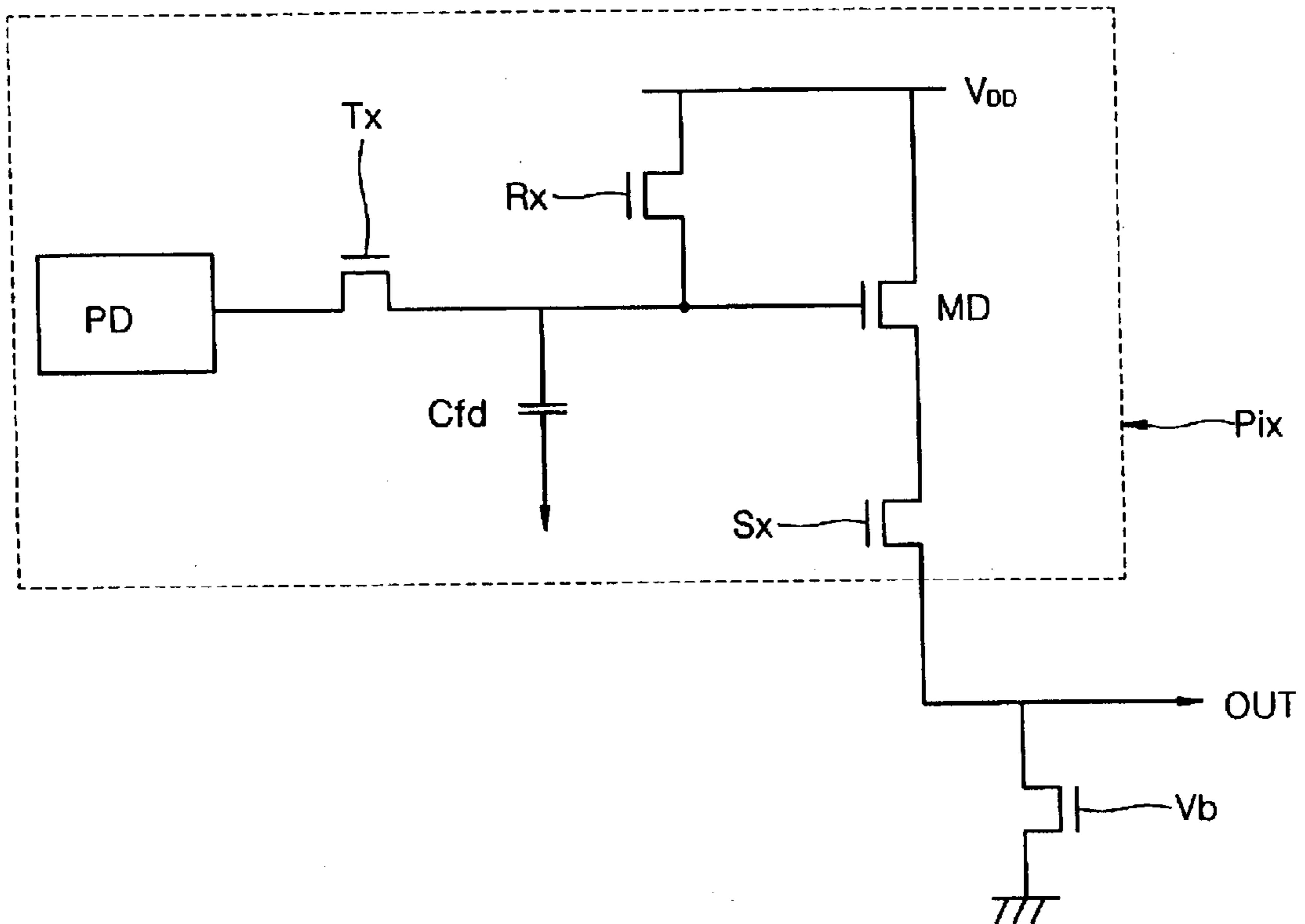
FIG. 2 (PRIOR ART)
