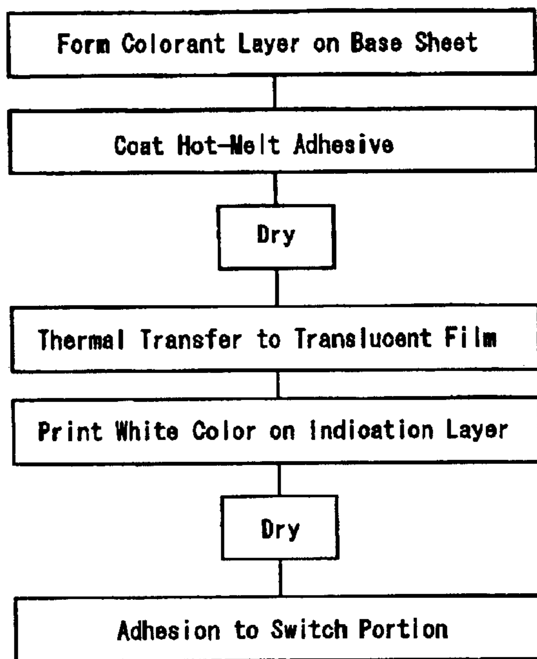
(b) MANUFACTURING FLOW OF PRESENT INVENTION
