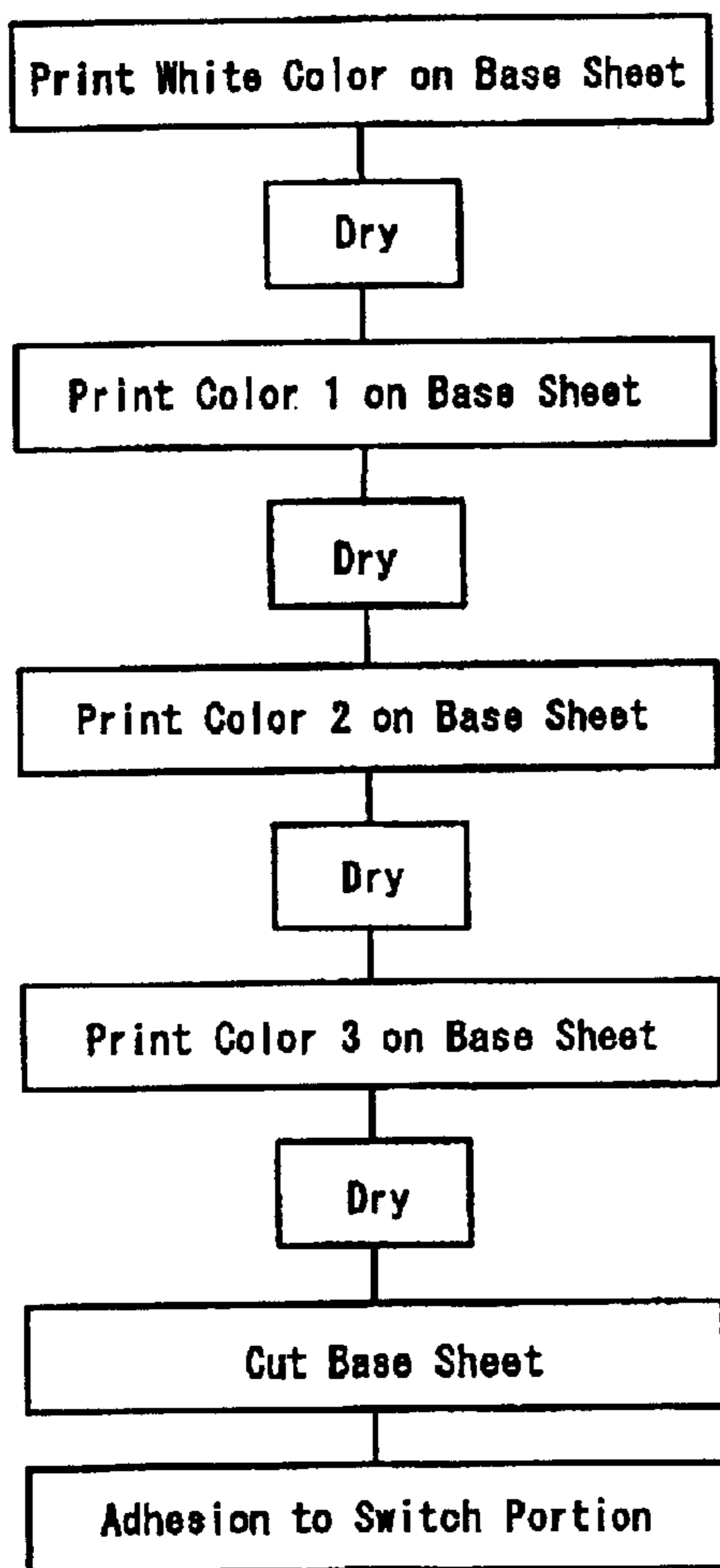
(a) CONVENTIONAL MANUFACTURING FLOW
