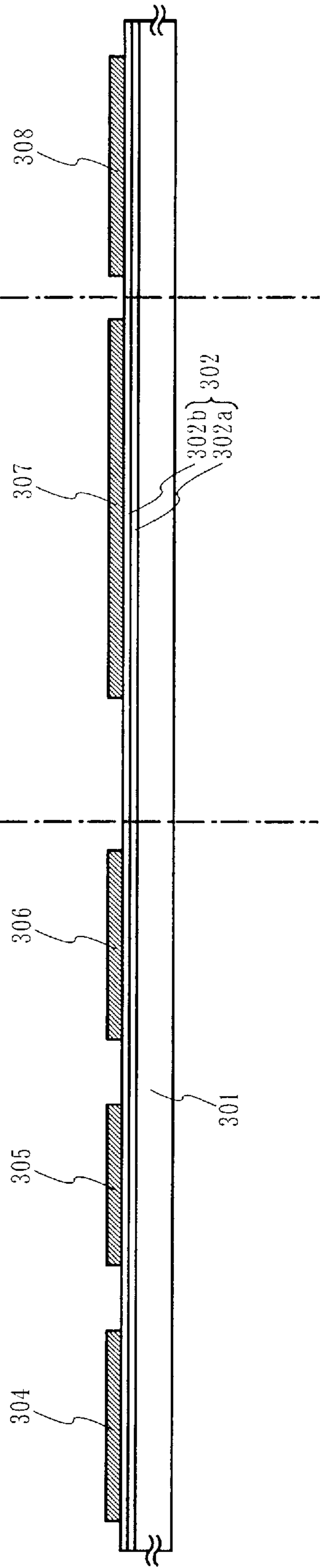
FIG. 8B DEPOSITING THE GATE INSULATING FILM/DEPOSITING THE GATE ELECTRODE
