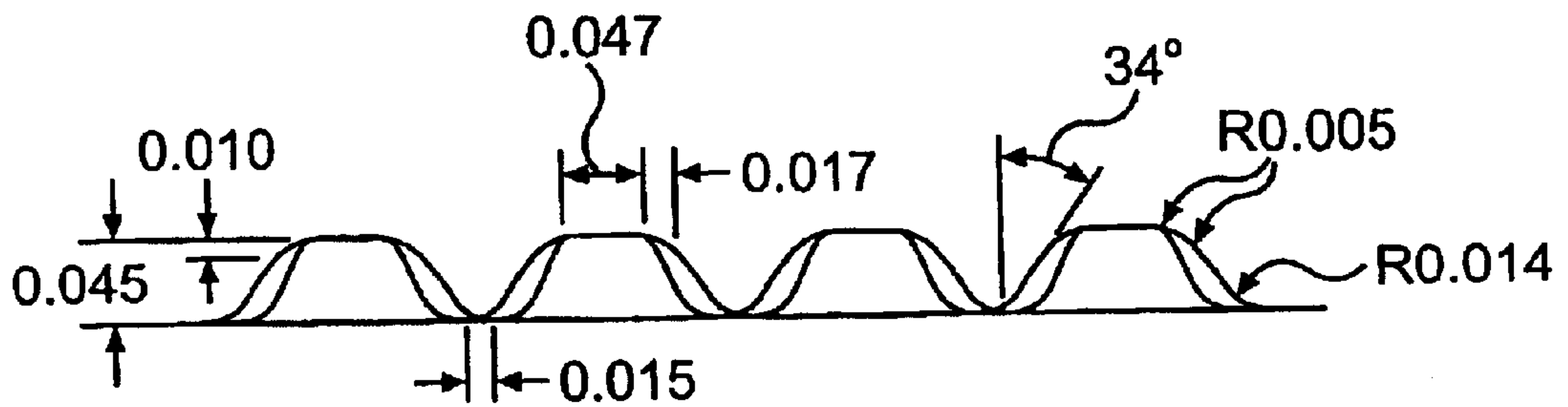
SIDE VIEW
