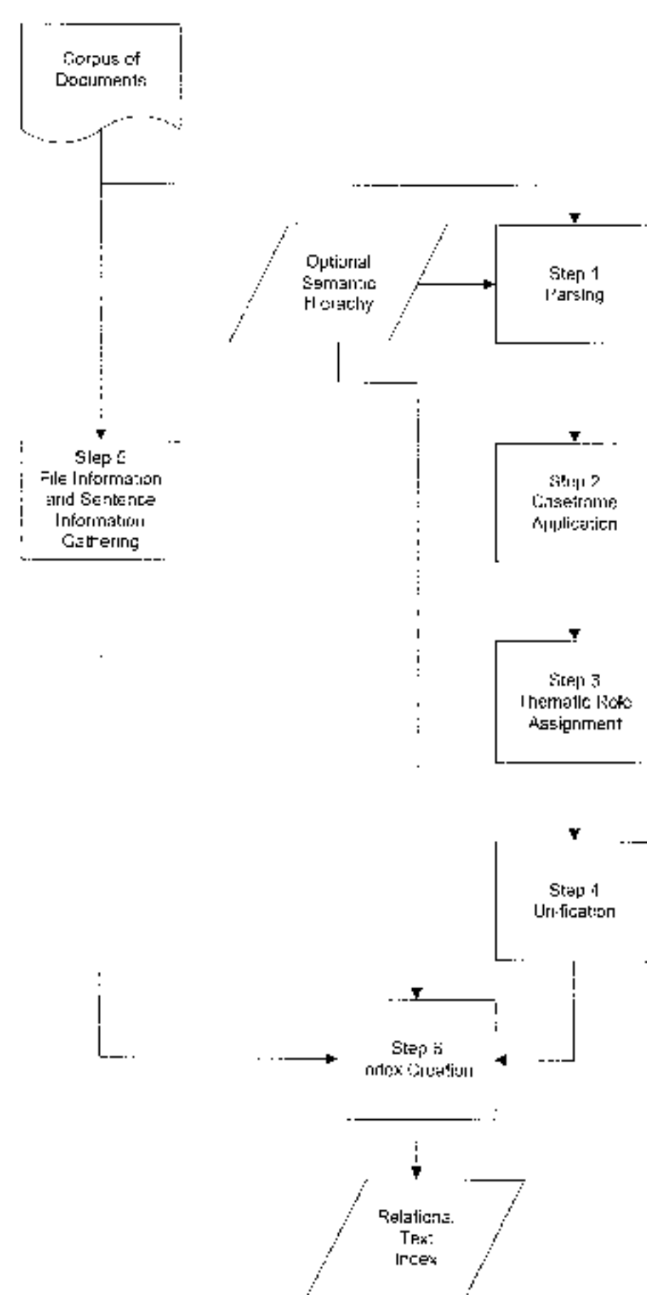
Index Creation Algorithm, High Level
