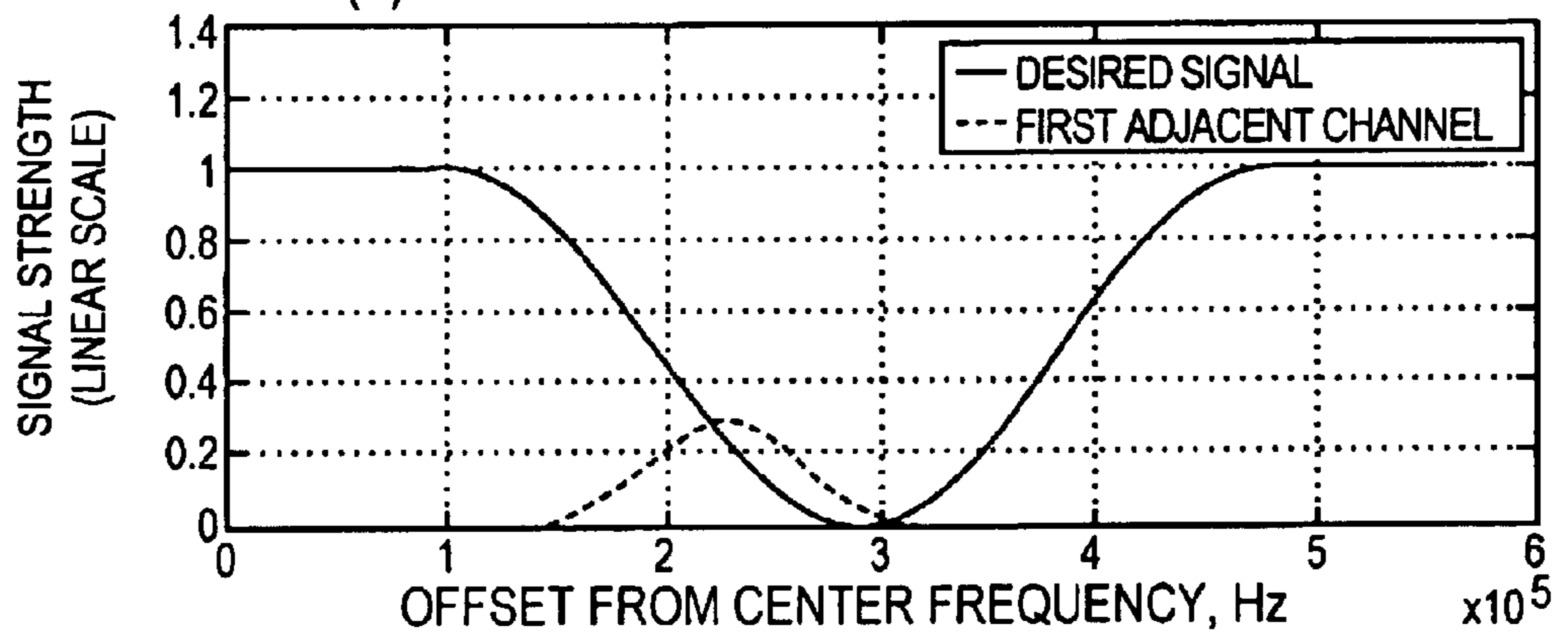
(B) SIGNAL STRENGTH AFTER T/1.5 SAMPLING
