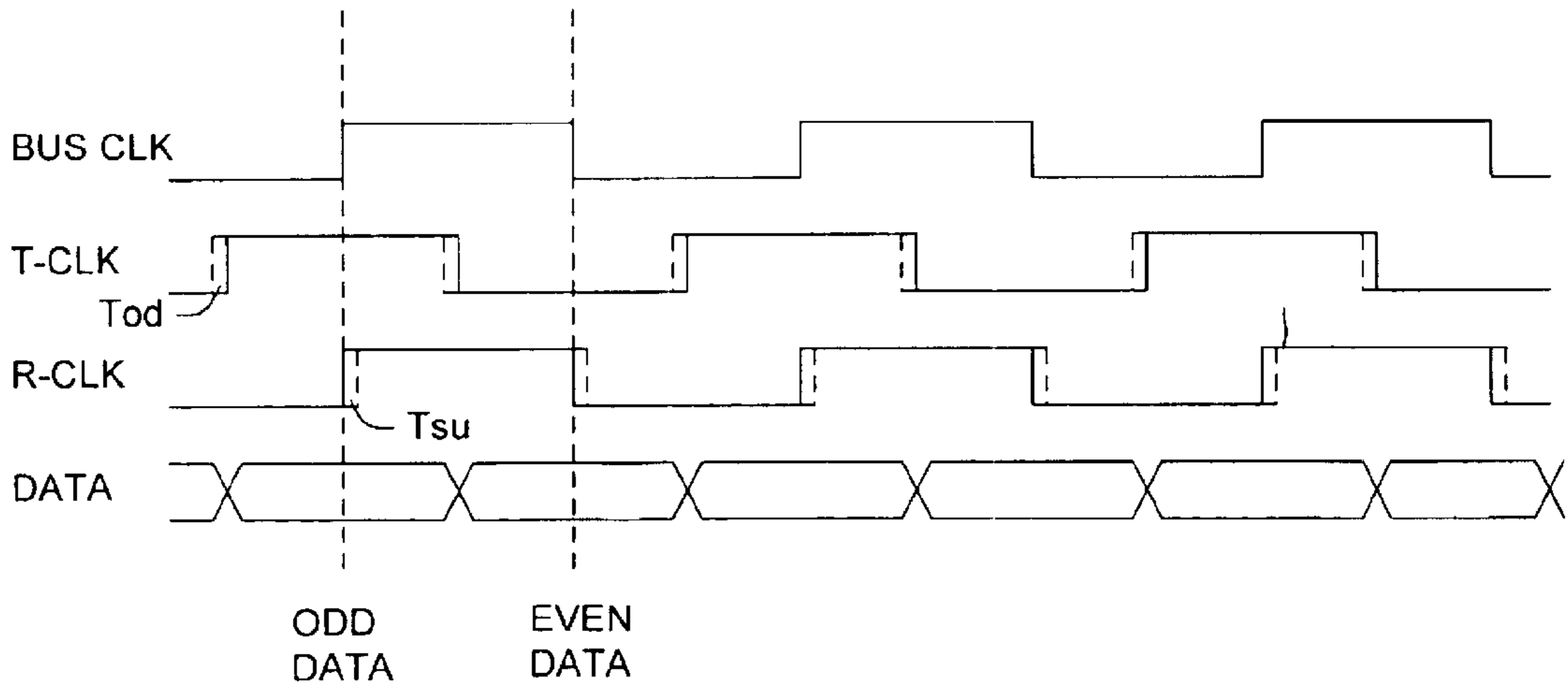
Fig. 2 (Prior Art)
