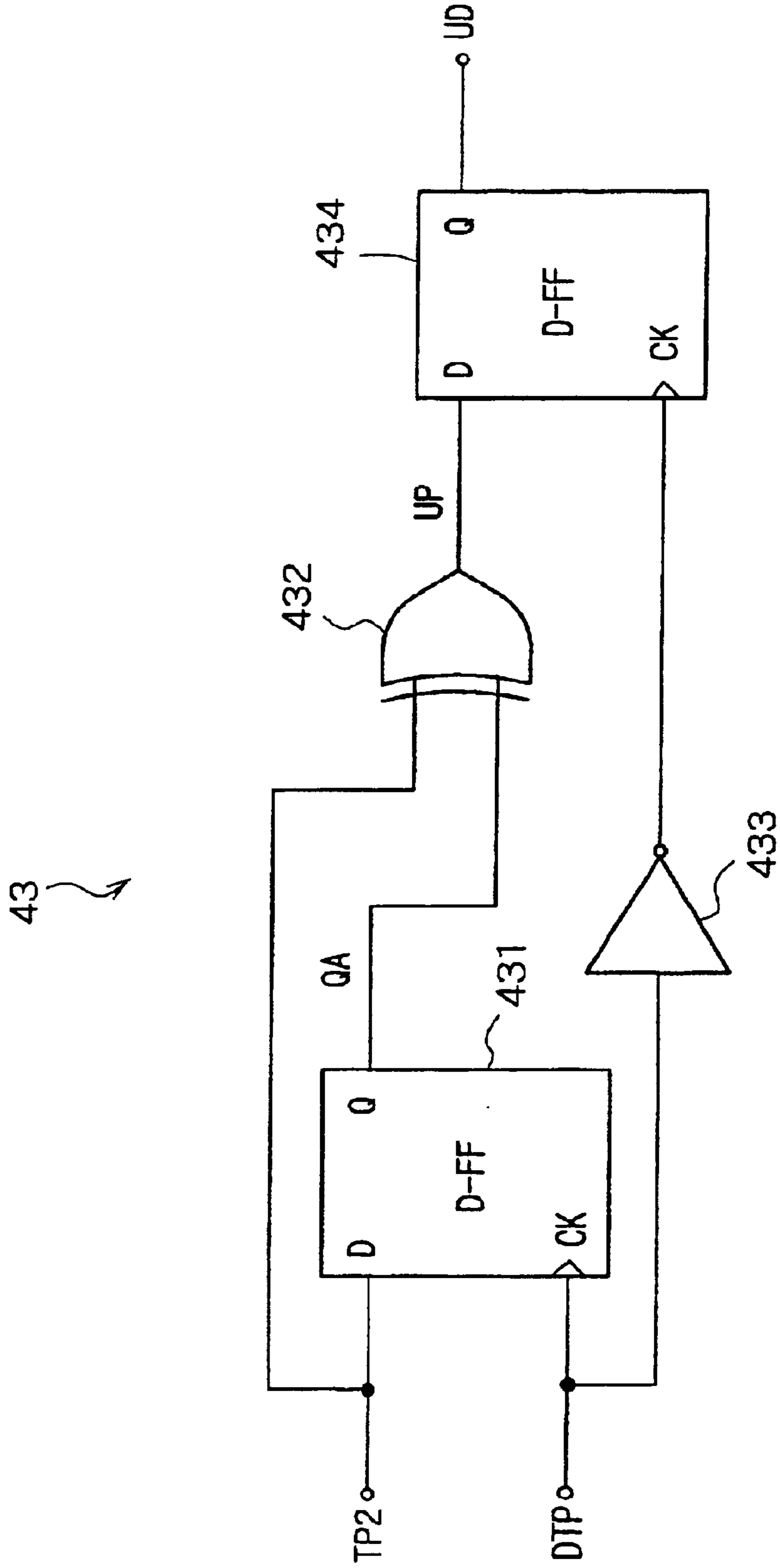
FIG.16 PRIOR ART
