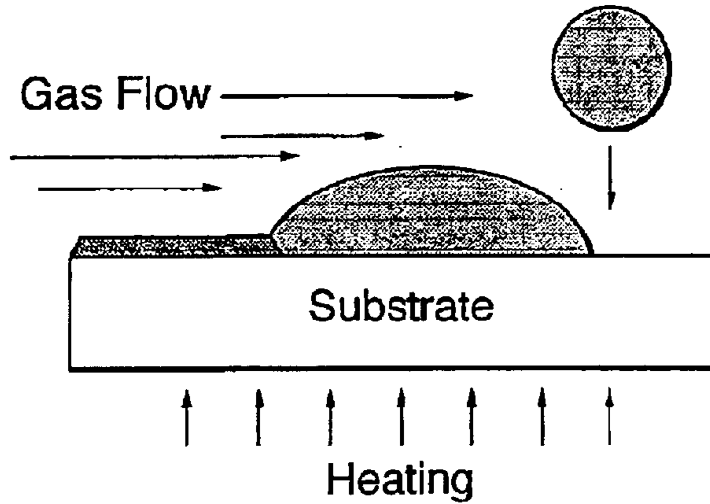
Fig.11. Continuous Inkjet Deposition
