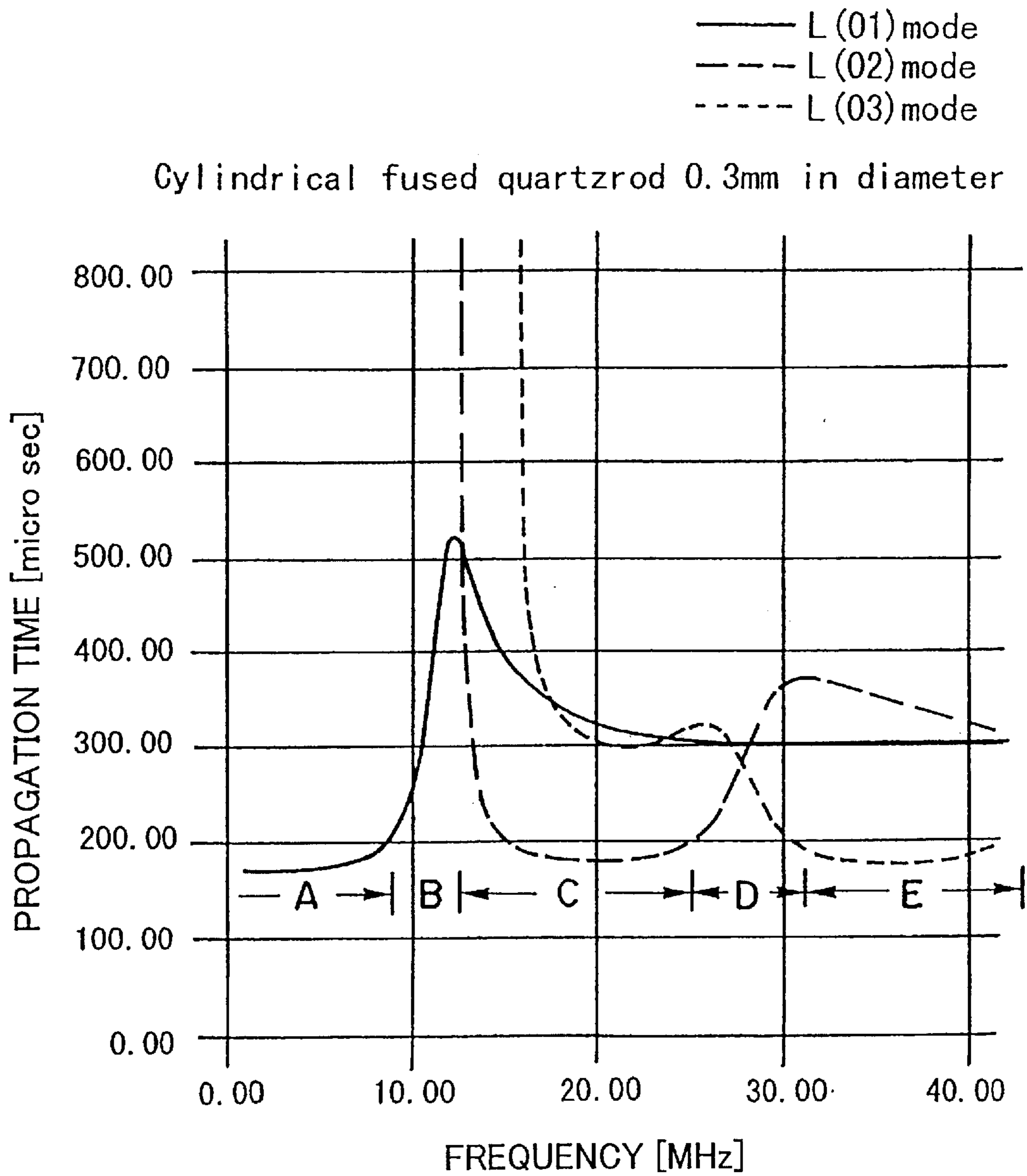
DISPERSION CHARACTERISTICS OF ELASTIC WAVE PROPAGATING THROUGH A FUSED QUARTZ ROD
