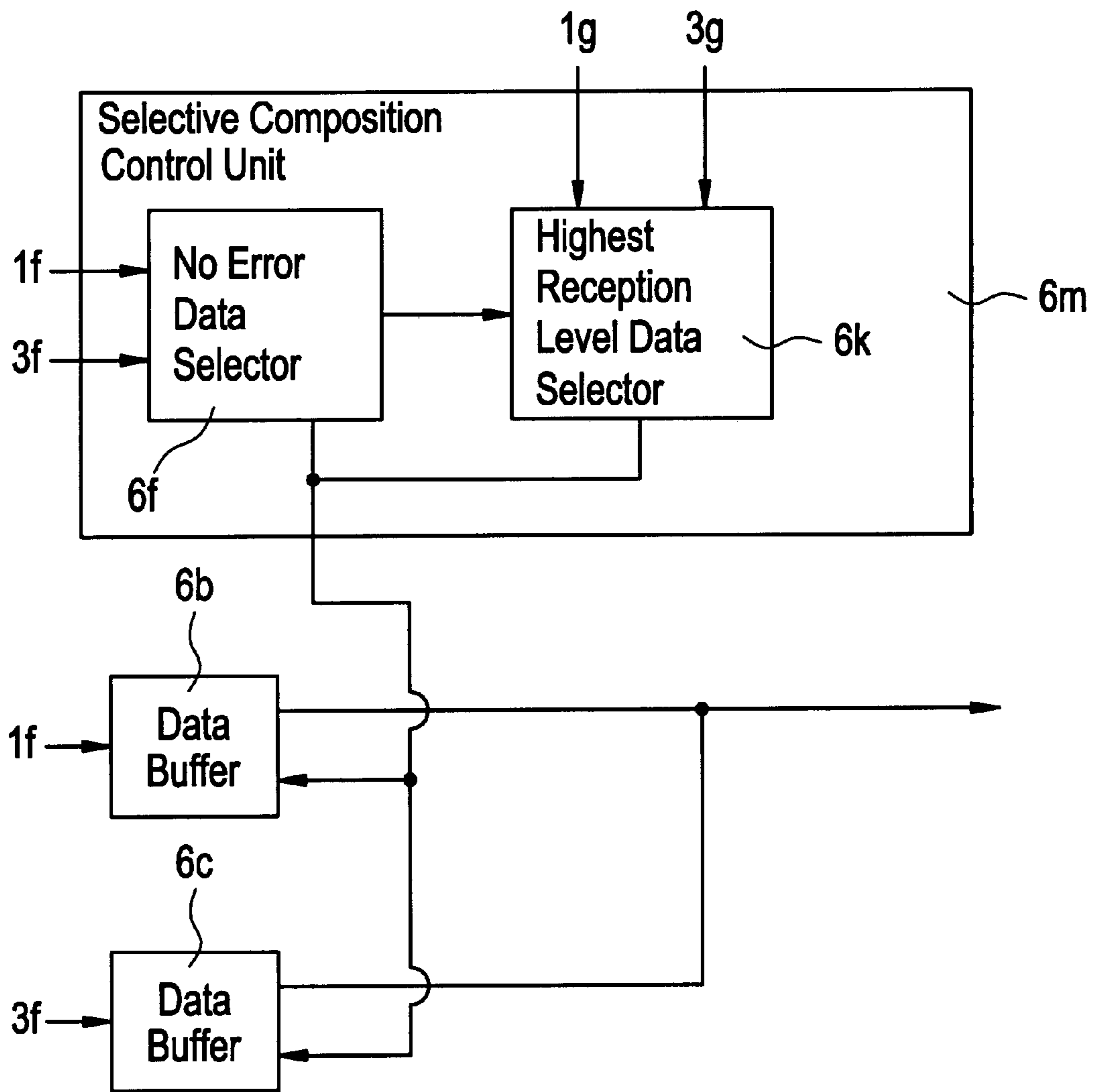
FIG. 3 PRIOR ART
