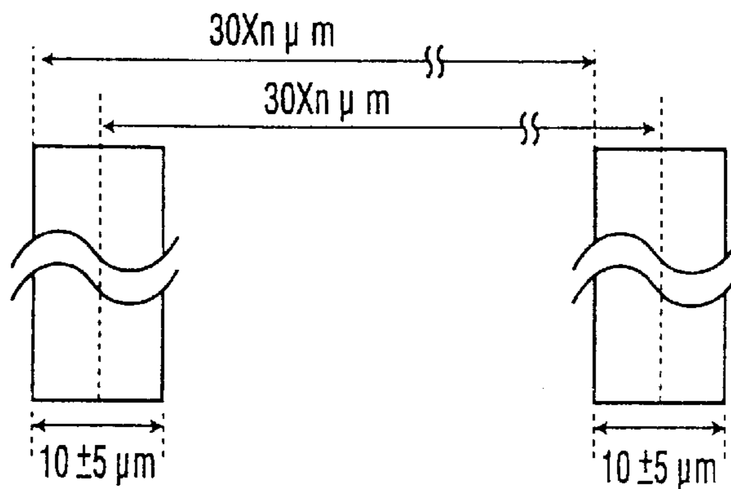
DIMENSIONAL ACCURACY OF SLIT (AT r=22.2\text{mm} )
