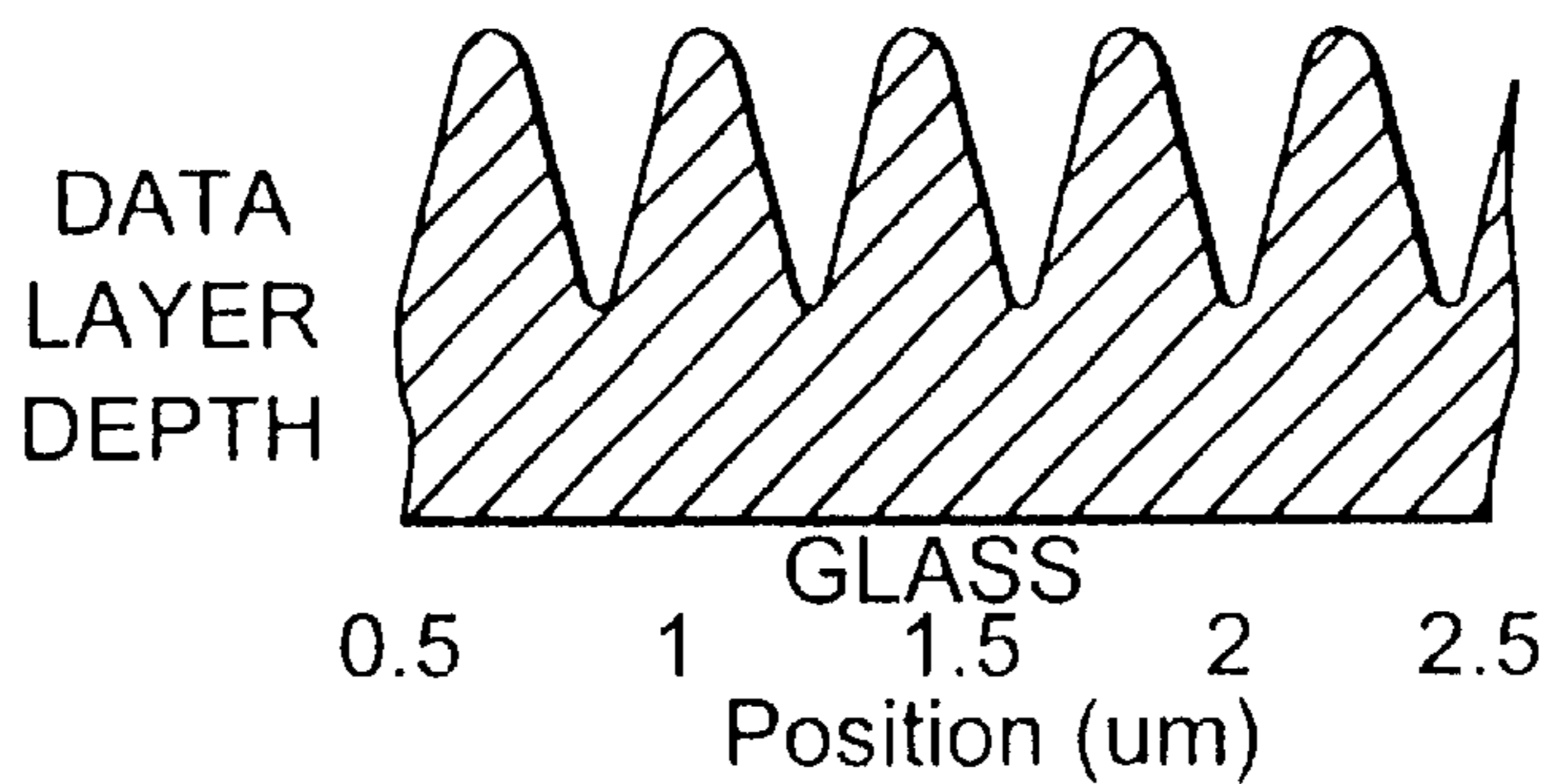
FIG. 2 PRIOR ART
