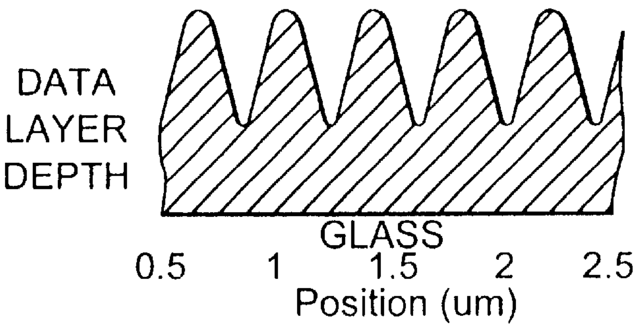
FIG. 2 PRIOR ART
