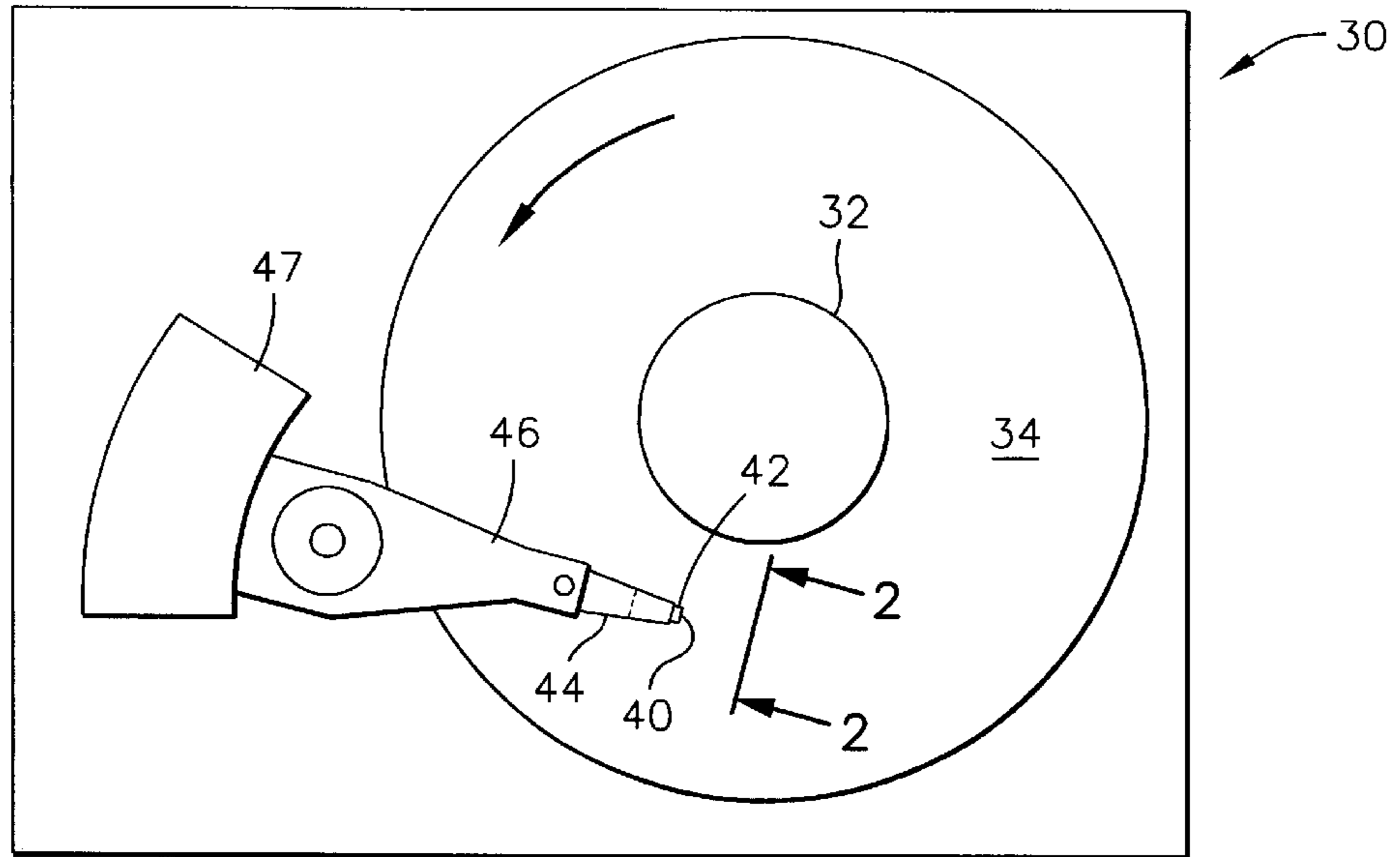
FIG. 1 (PRIOR ART)
