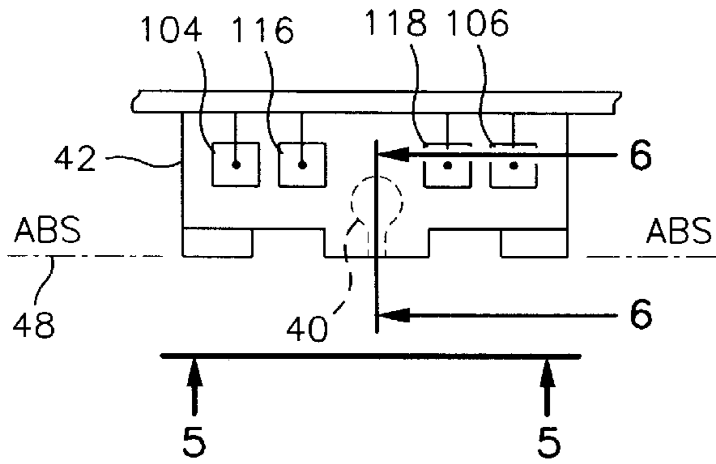
FIG. 2 (PRIOR ART)
