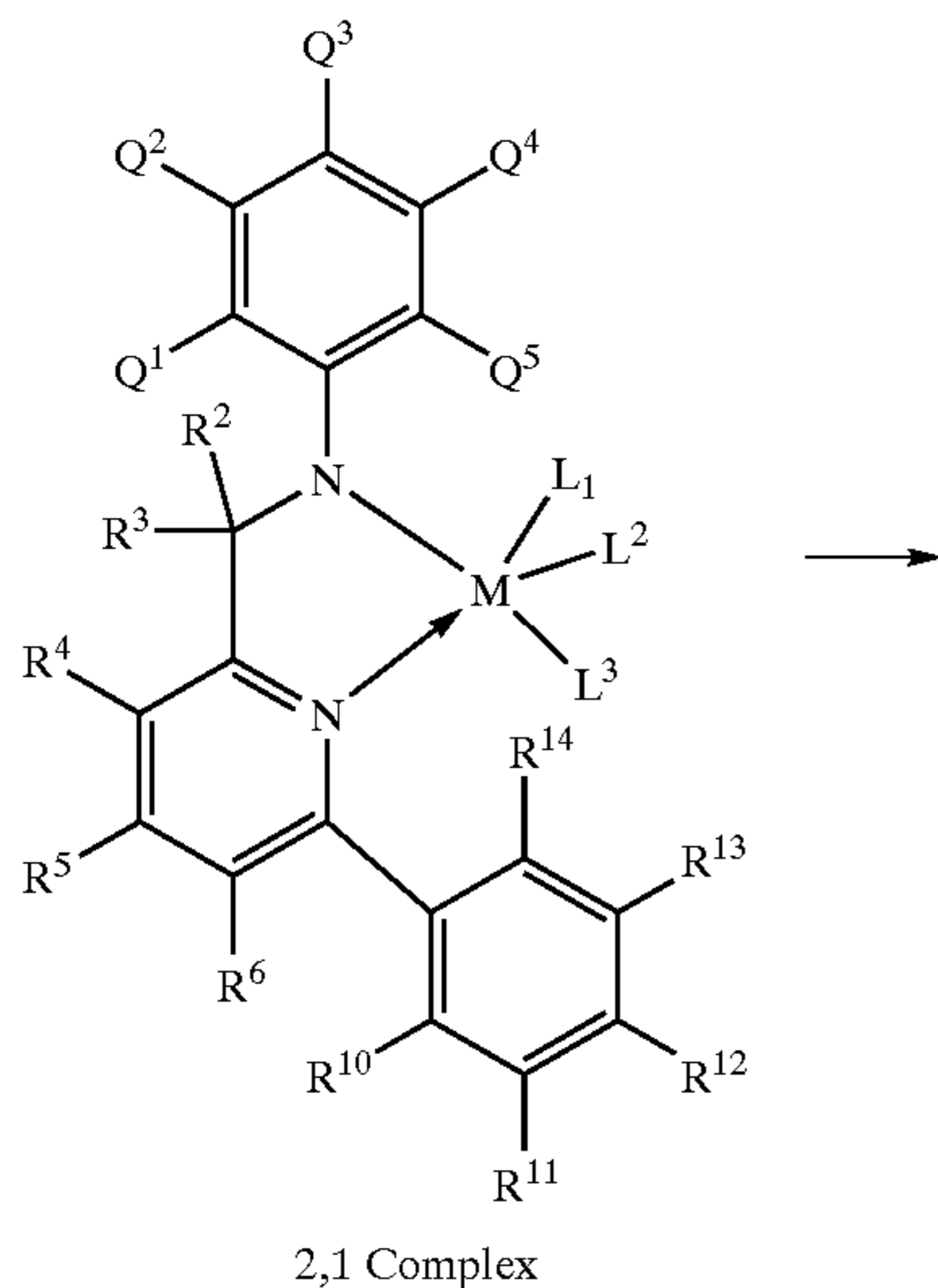
Scheme 3
